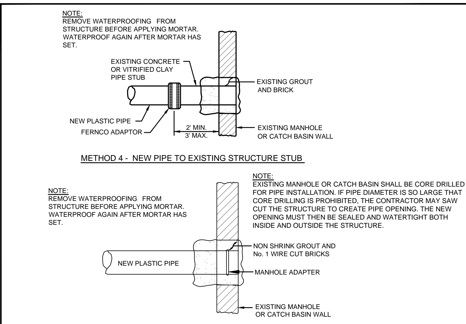
(G) PLASTIC PIPE CONNECTION METHODS 3 & 4 N.T.S.
