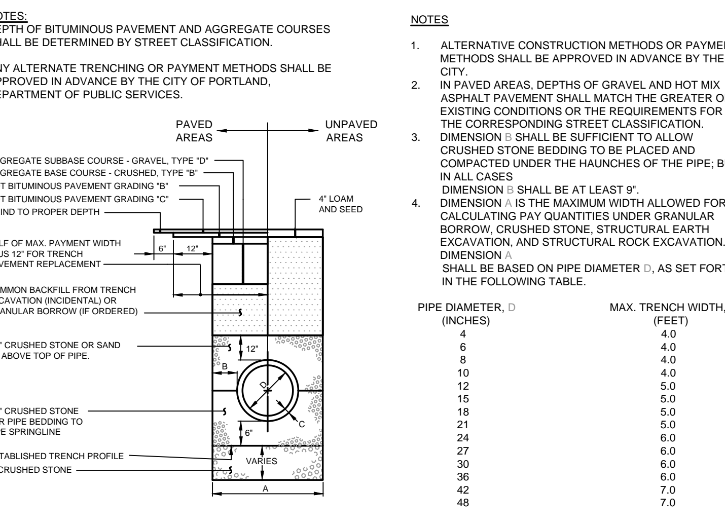
(C) TYPICAL TRENCH INSTALLATION AND NOTES N.T.S.
