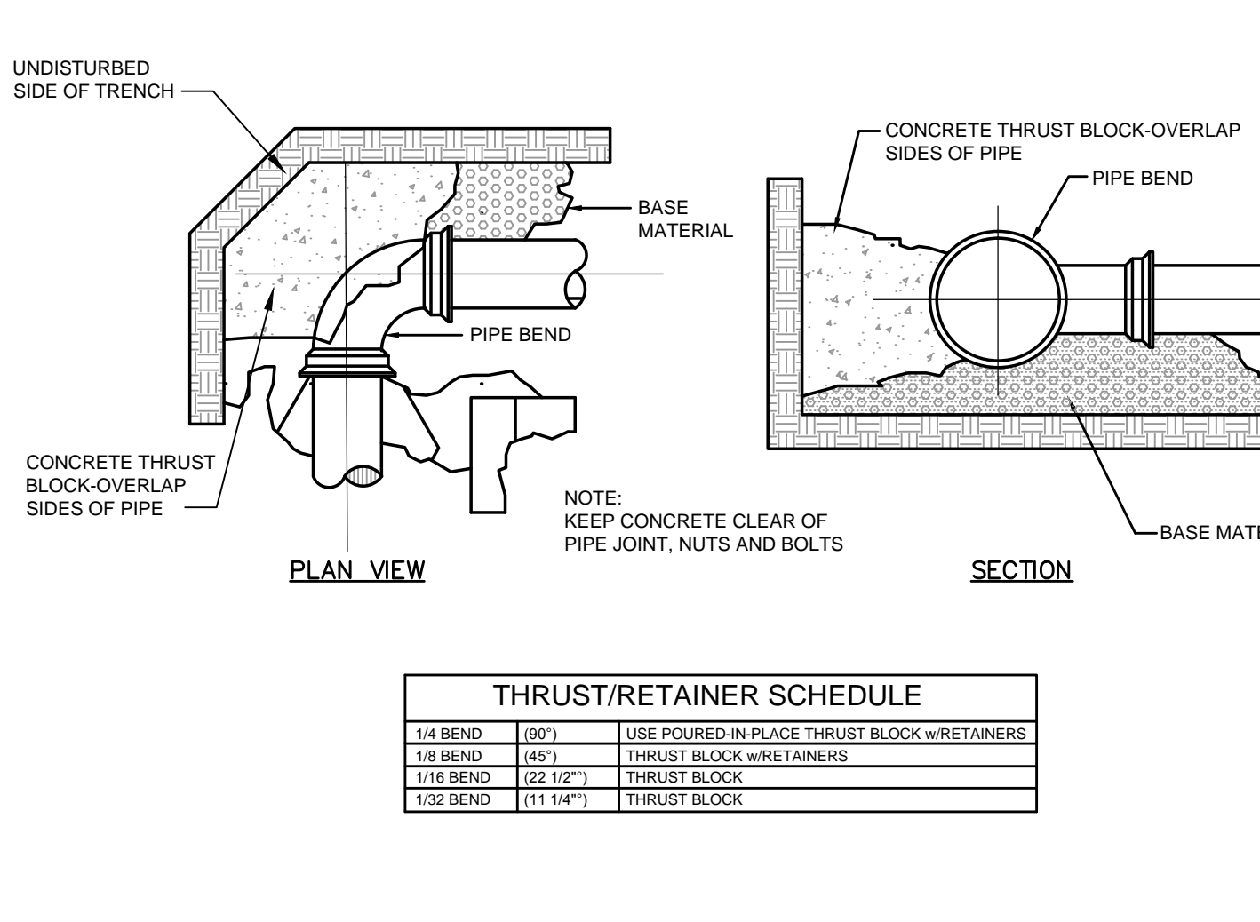
(F) FORCE MAIN CONCRETE THRUST BLOCK PLACEMENT ON VERTICAL & HORIZONTAL BENDS N.T.S.
