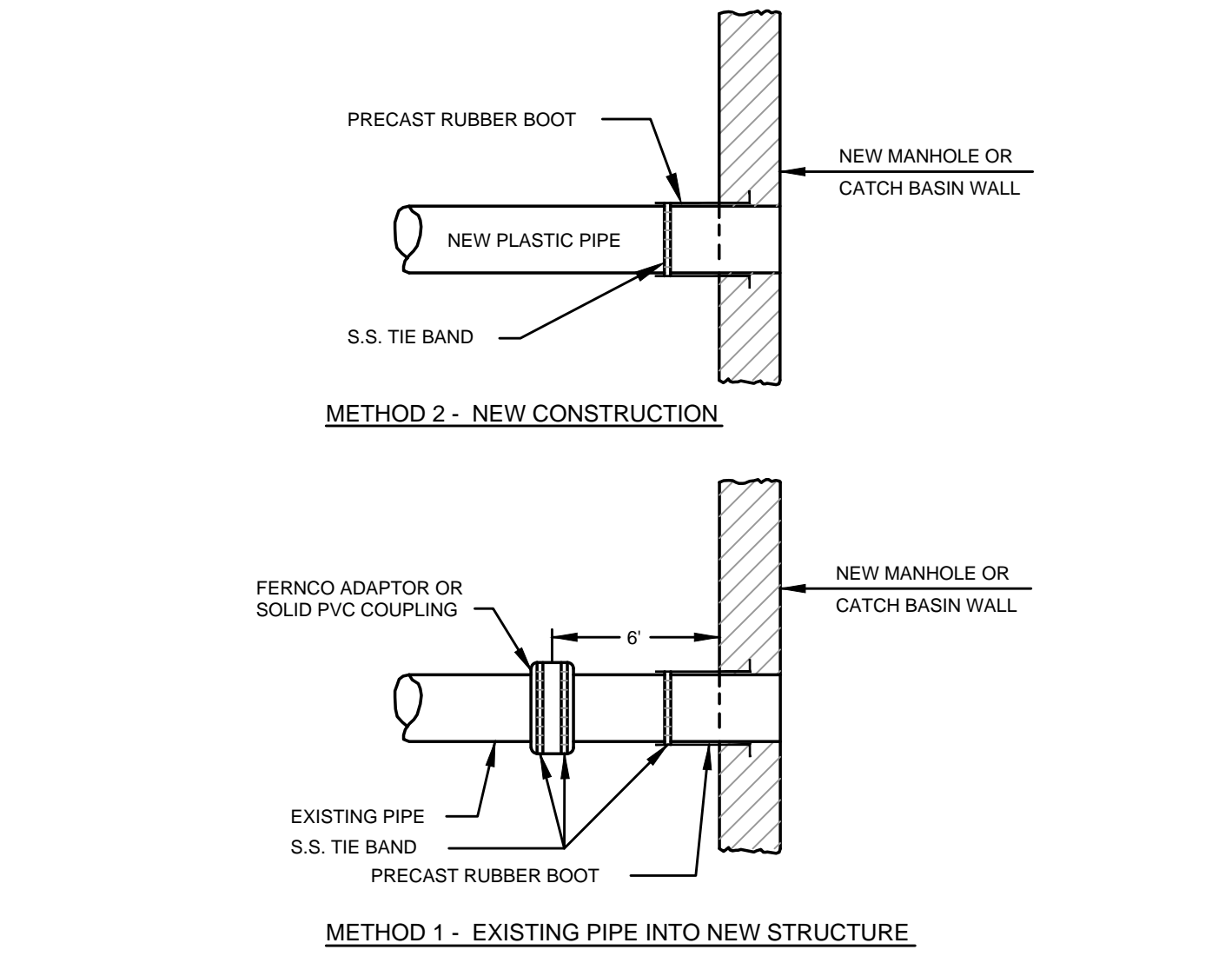
(E) PLASTIC PIPE CONNECTION METHODS 1 & 2 N.T.S.
