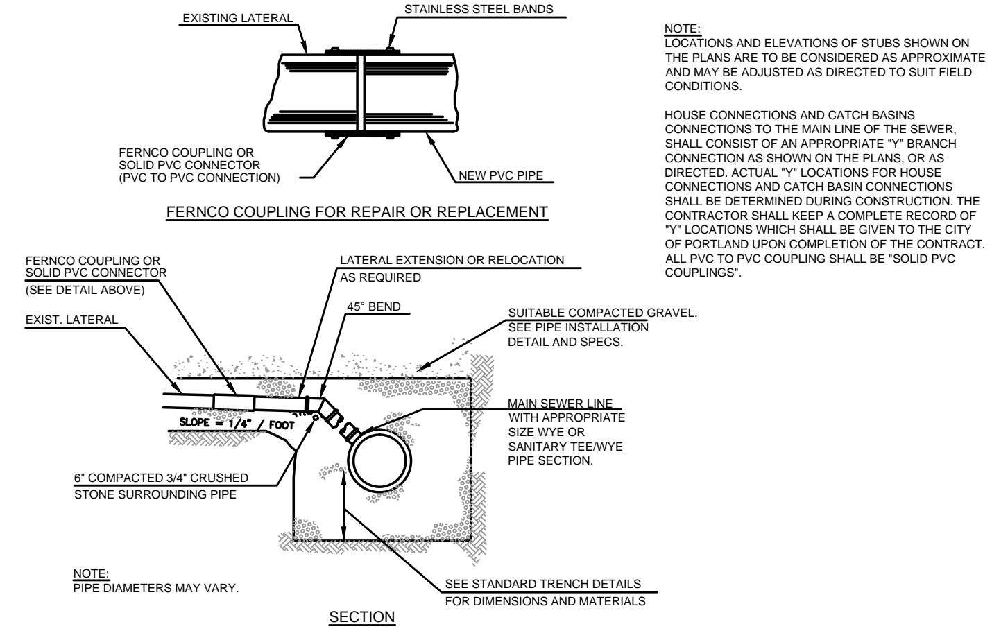
(B) TYPICAL EXISTING LATERAL CONNECTION N.T.S.
