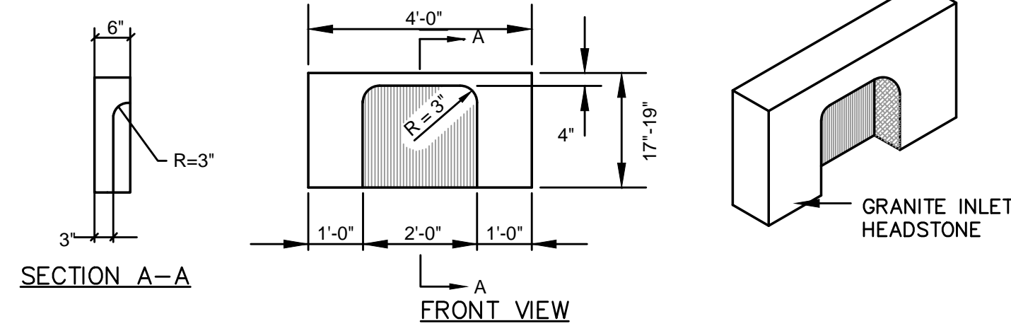
(A) 4' GRANITE HEADSTONE FOR CATCH BASIN INLET N.T.S.
