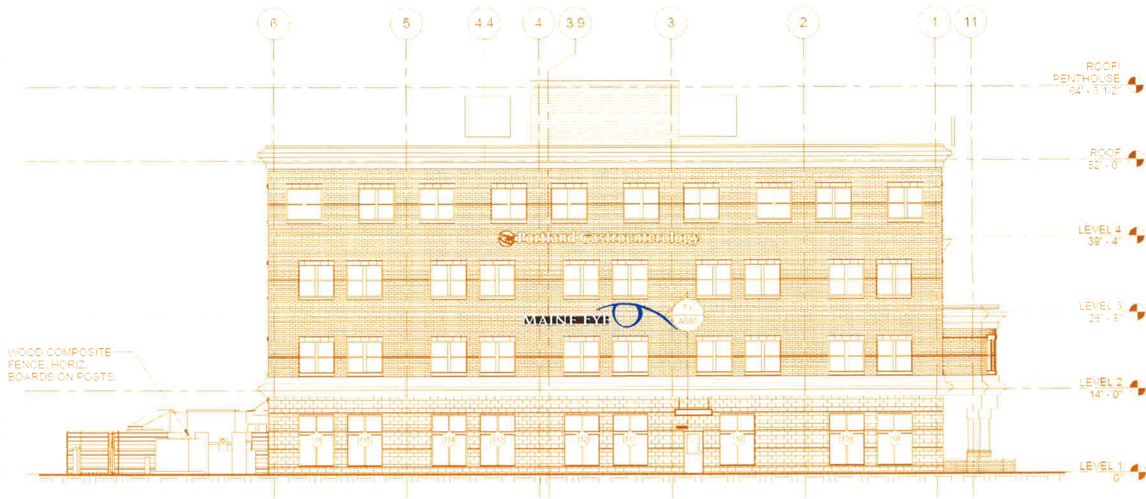
4 WEST ELEVATION
