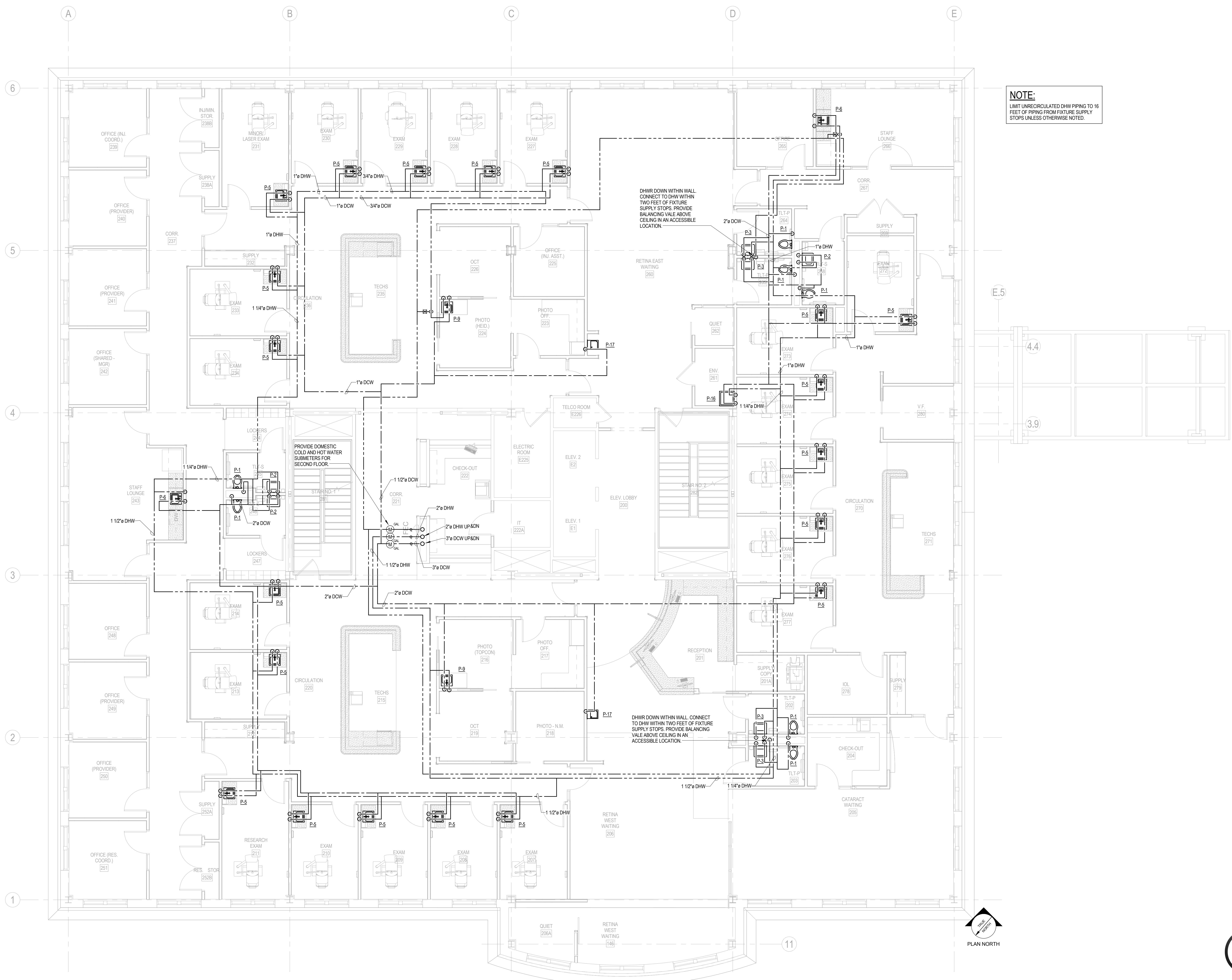
1 PLUMBING DOMESTIC WATER LEVEL 2 NEW PLAN 3/16" = 1'-0"
