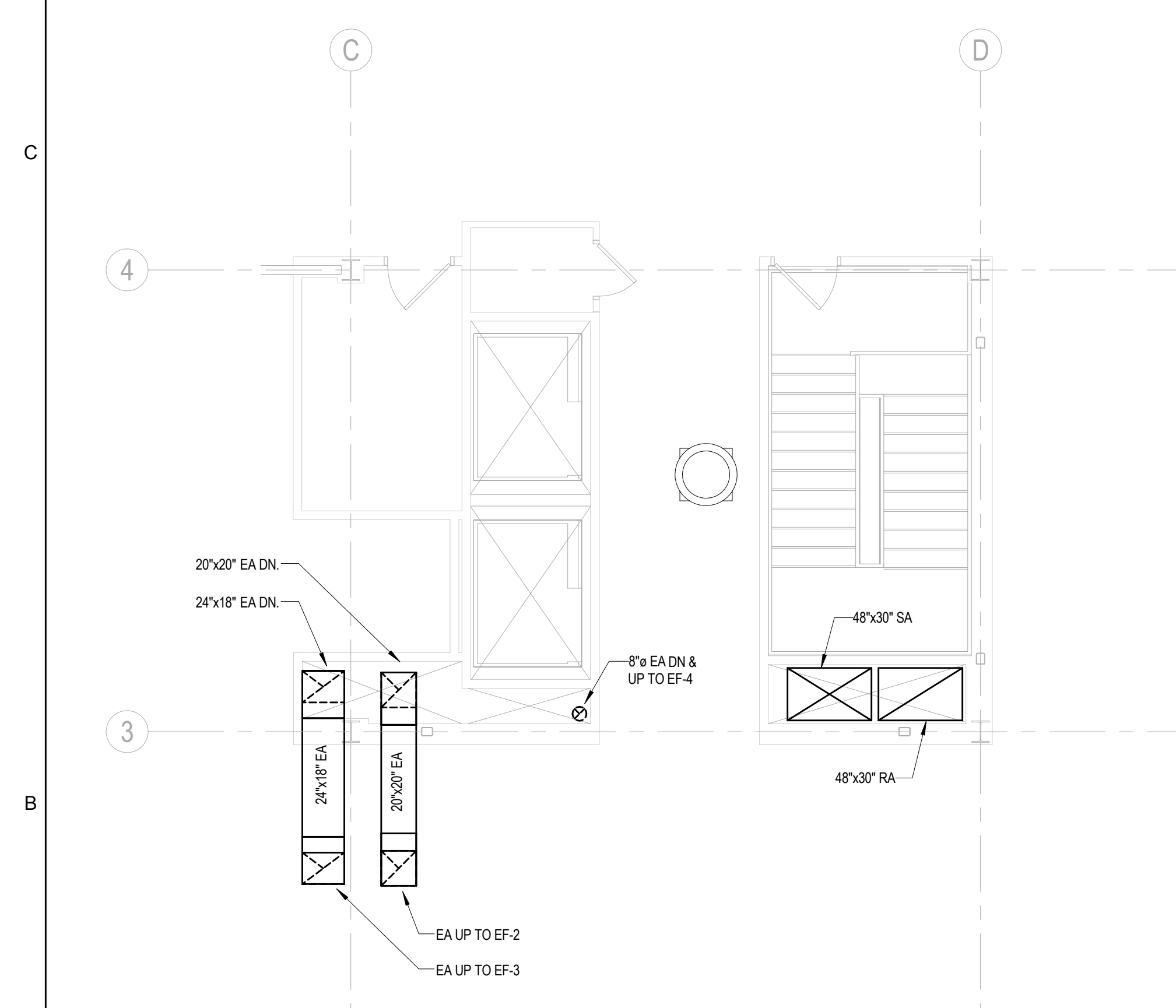
③ HVAC DUCTWORK LEVEL 4 NEW PLAN 3/16" = 1'-0"
