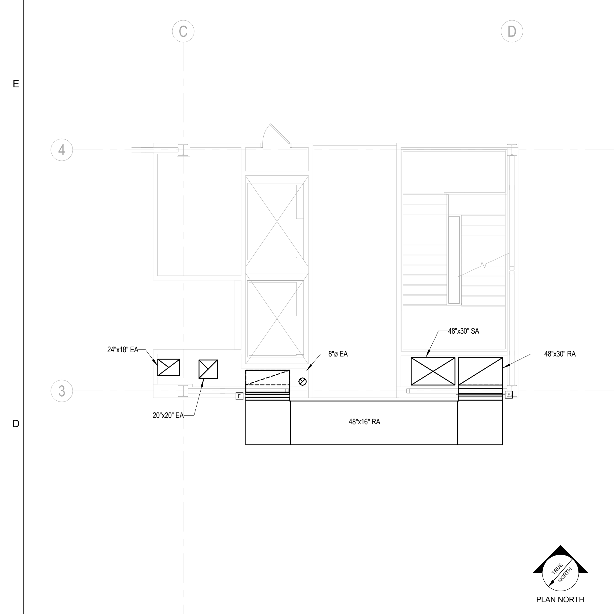
② HVAC DUCTWORK LEVEL 3 NEW PLAN 3/16" = 1'-0"
