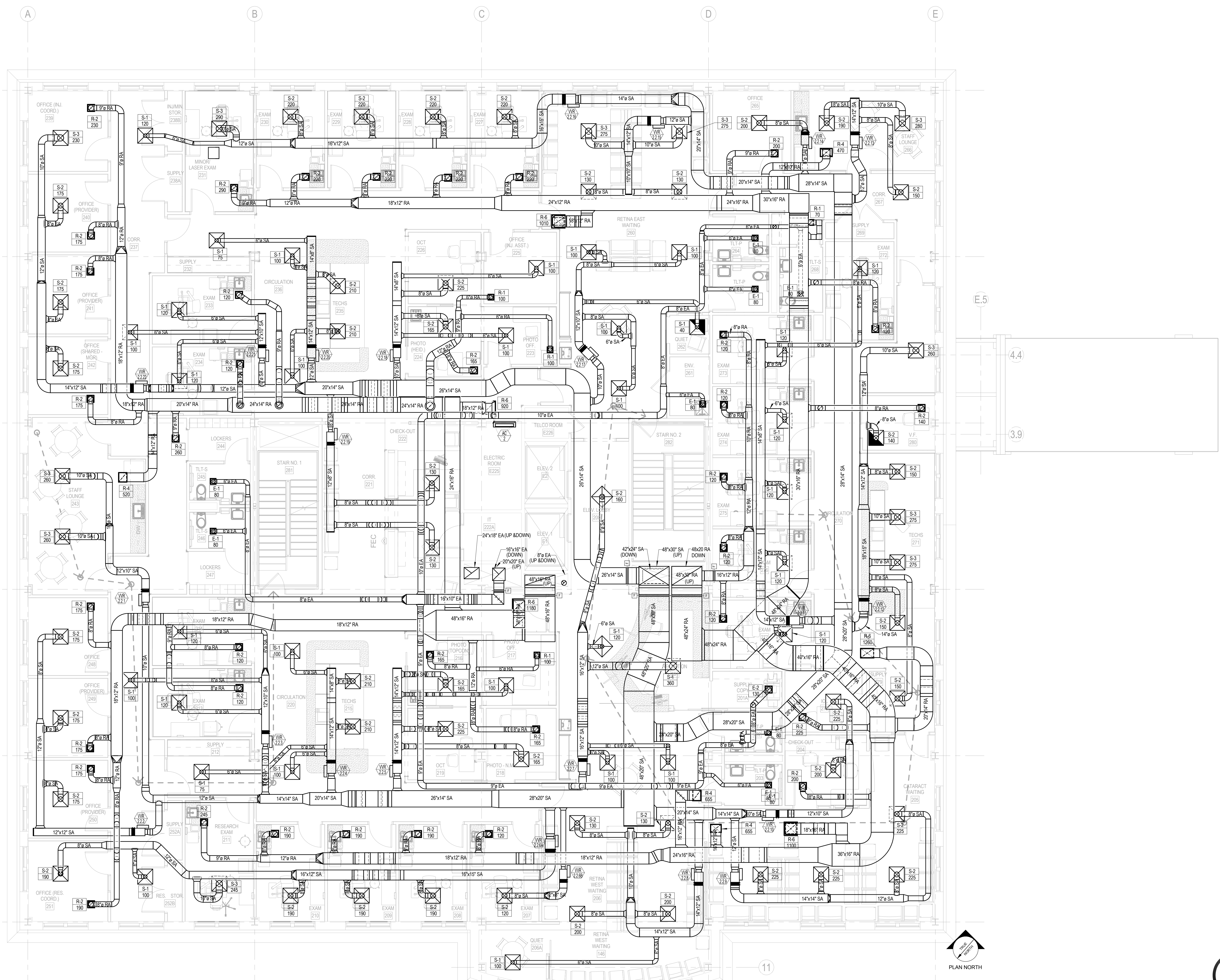
1 HVAC DUCTWORK LEVEL 2 NEW PLAN 3/16" = 1'-0"
