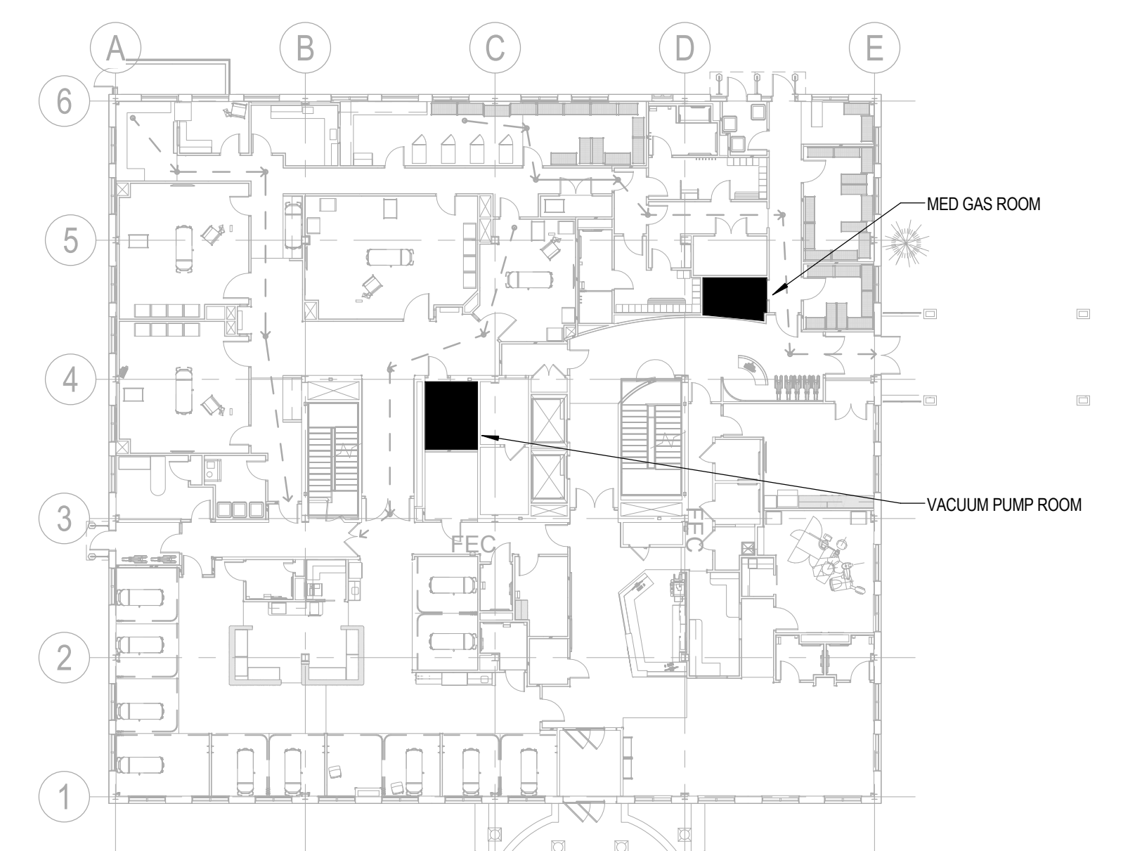
2 LEVEL 1 KEY PLAN 3/64" = 1'-0"
