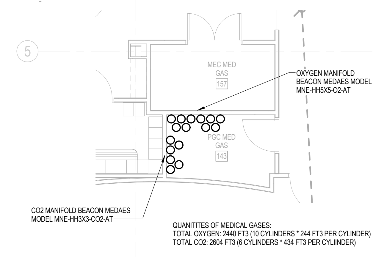
3 PLUMBING MEDICAL GAS LEVEL 1 MEDICAL GAS ROOM PART PLAN 3/16" = 1'-0"
