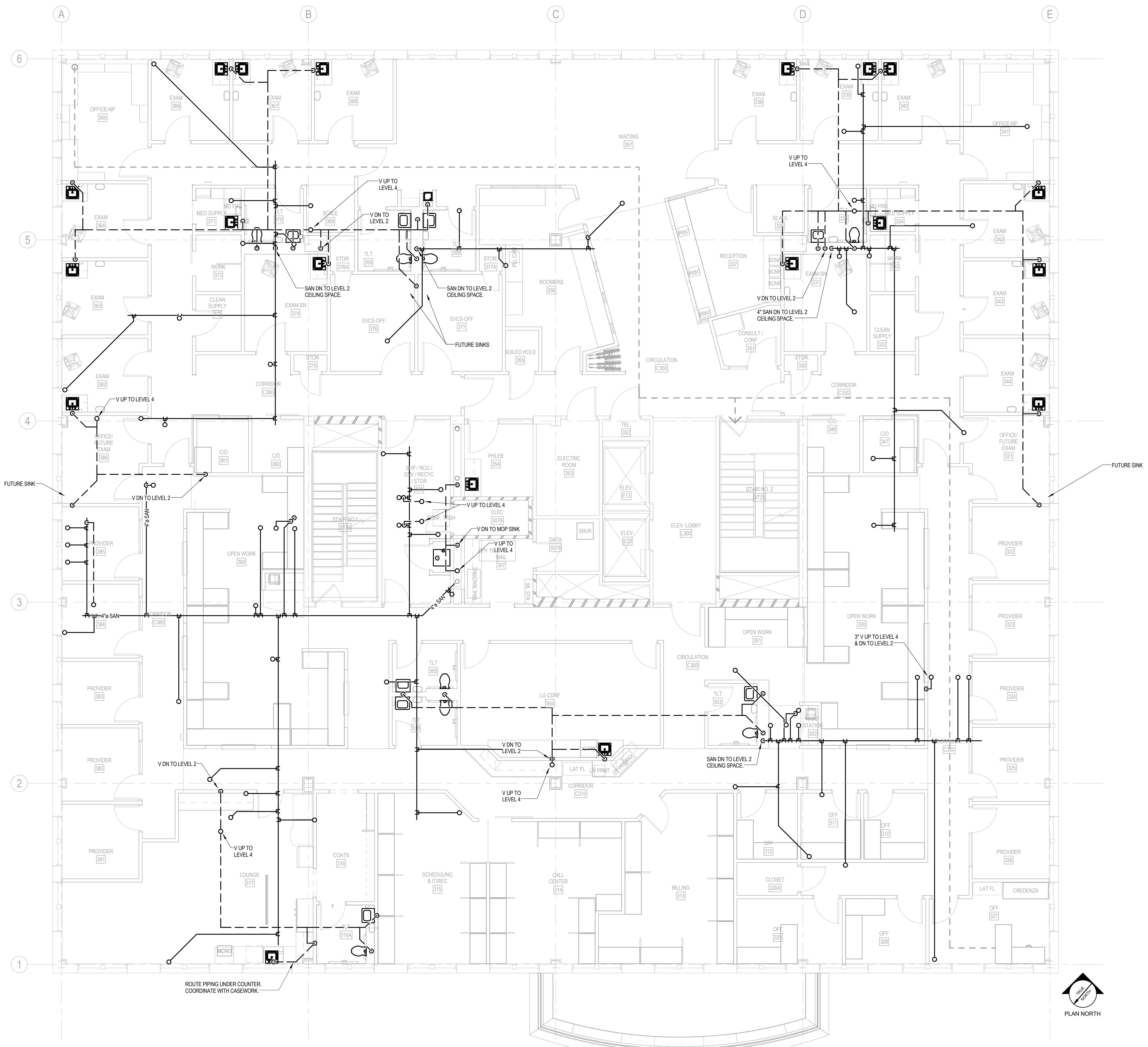
1 PLUMBING SANITARY & VENT LEVEL 3 NEW PLAN 3/18" = 1'-0"
