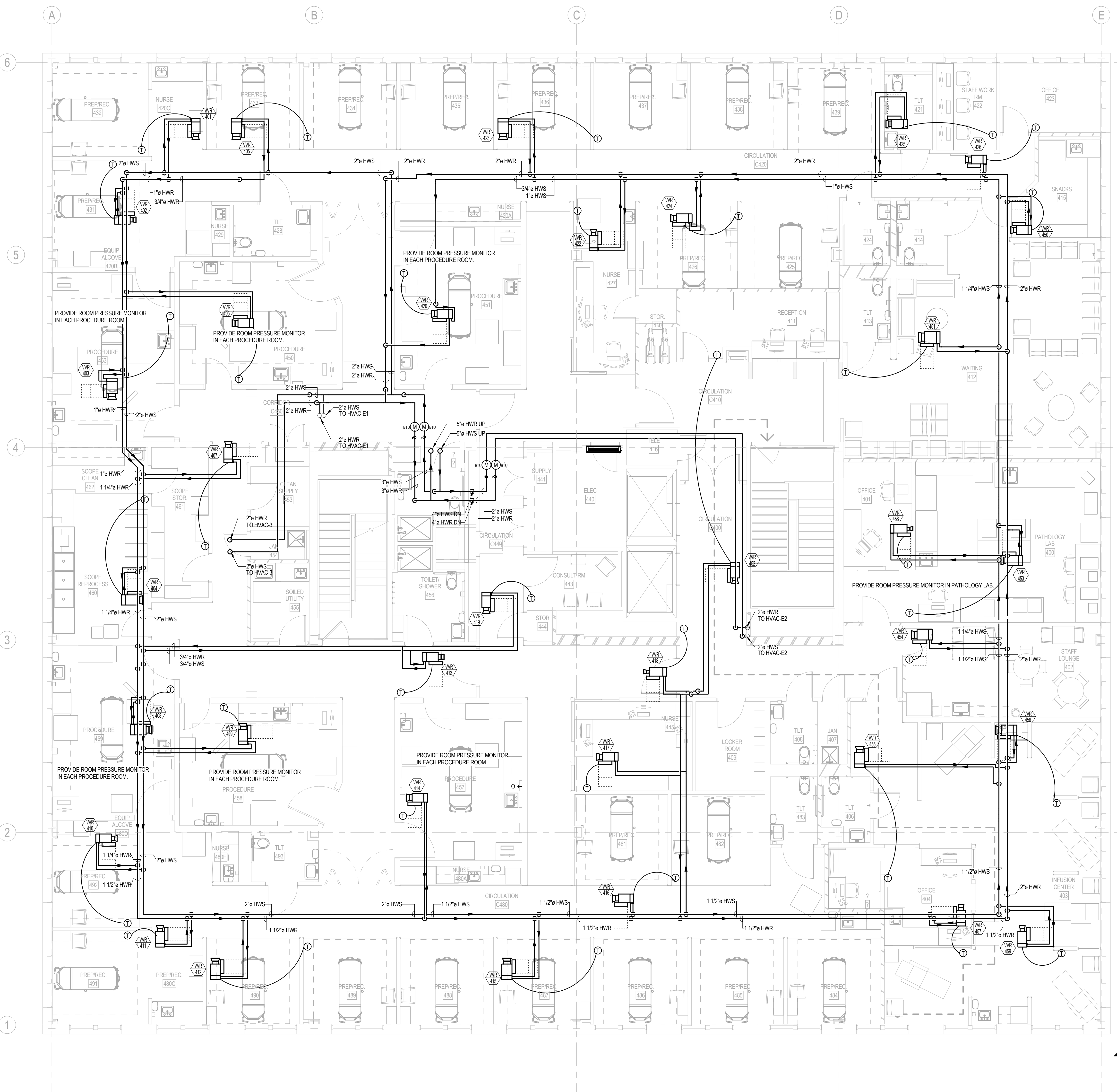
1 HVAC PIPING LEVEL 4 NEW PLAN 3/16" = 1'-0"
