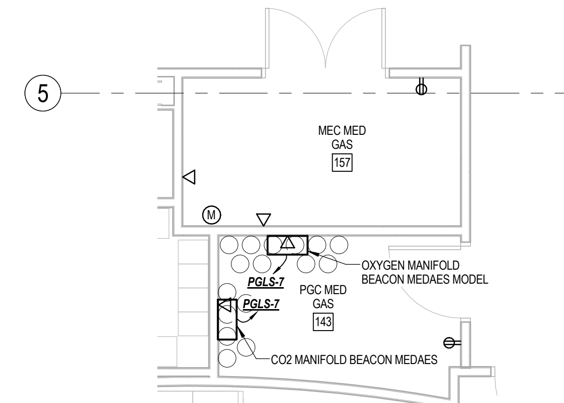
POWER AND SYSTEM LEVEL 1 MEDICAL GAS ROOM PART PLAN 1/4" = 1'-0"
