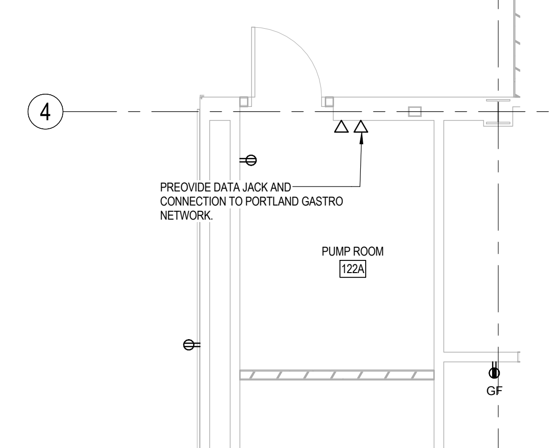
POWER AND SYSTEM LEVEL 1 VACUUM PUMP ROOM PART PLAN 1/4" = 1'-0"
