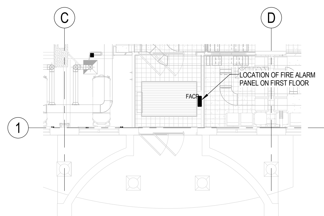
ELECTRICAL SYSTEMS LOBBY ENTRANCE 1/8" = 1'-0"
