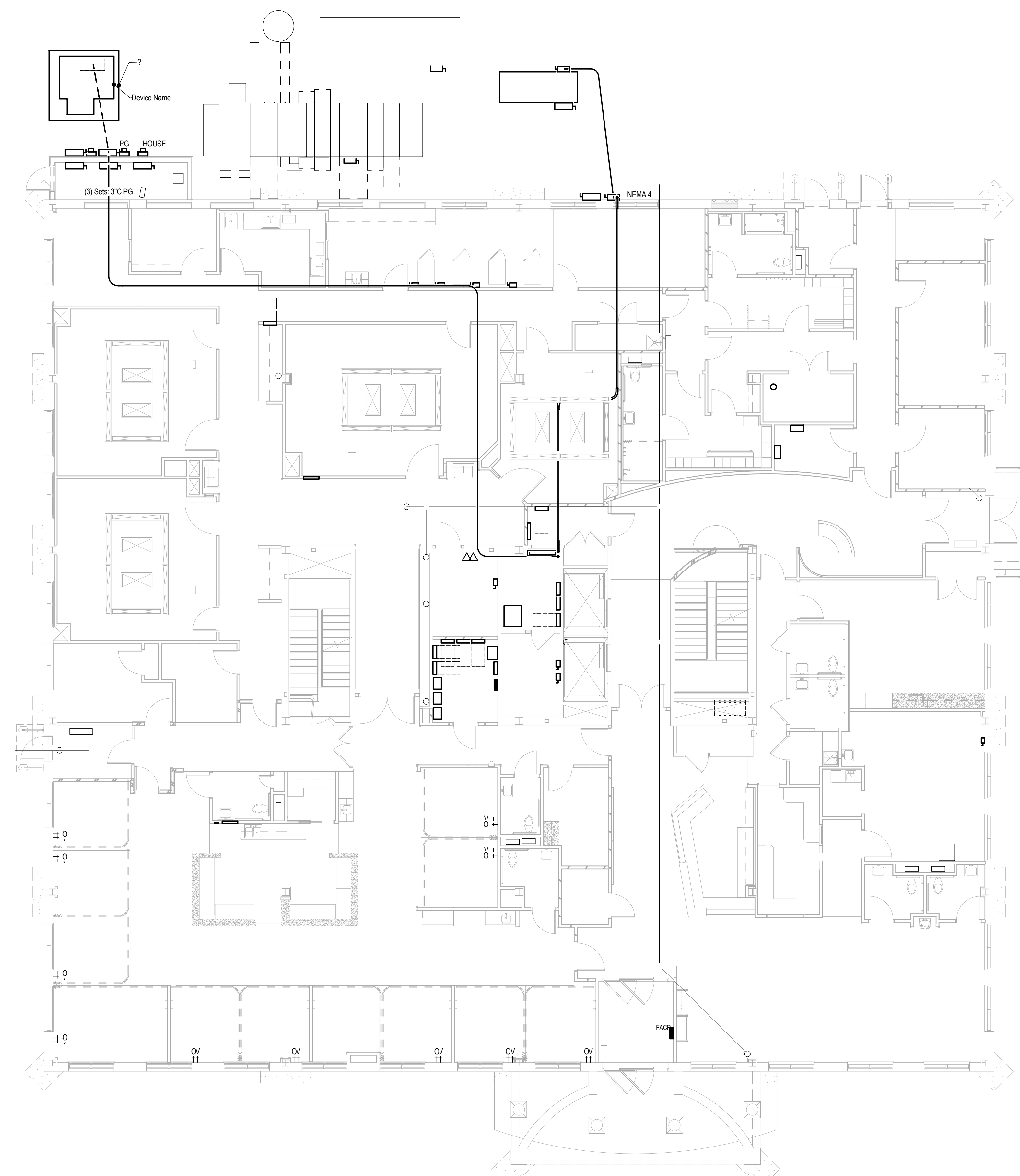
ELECTRICAL SITE PLAN & FIRST FLOOR CONDUIT ROUTING 1/8" = 1'-0"
