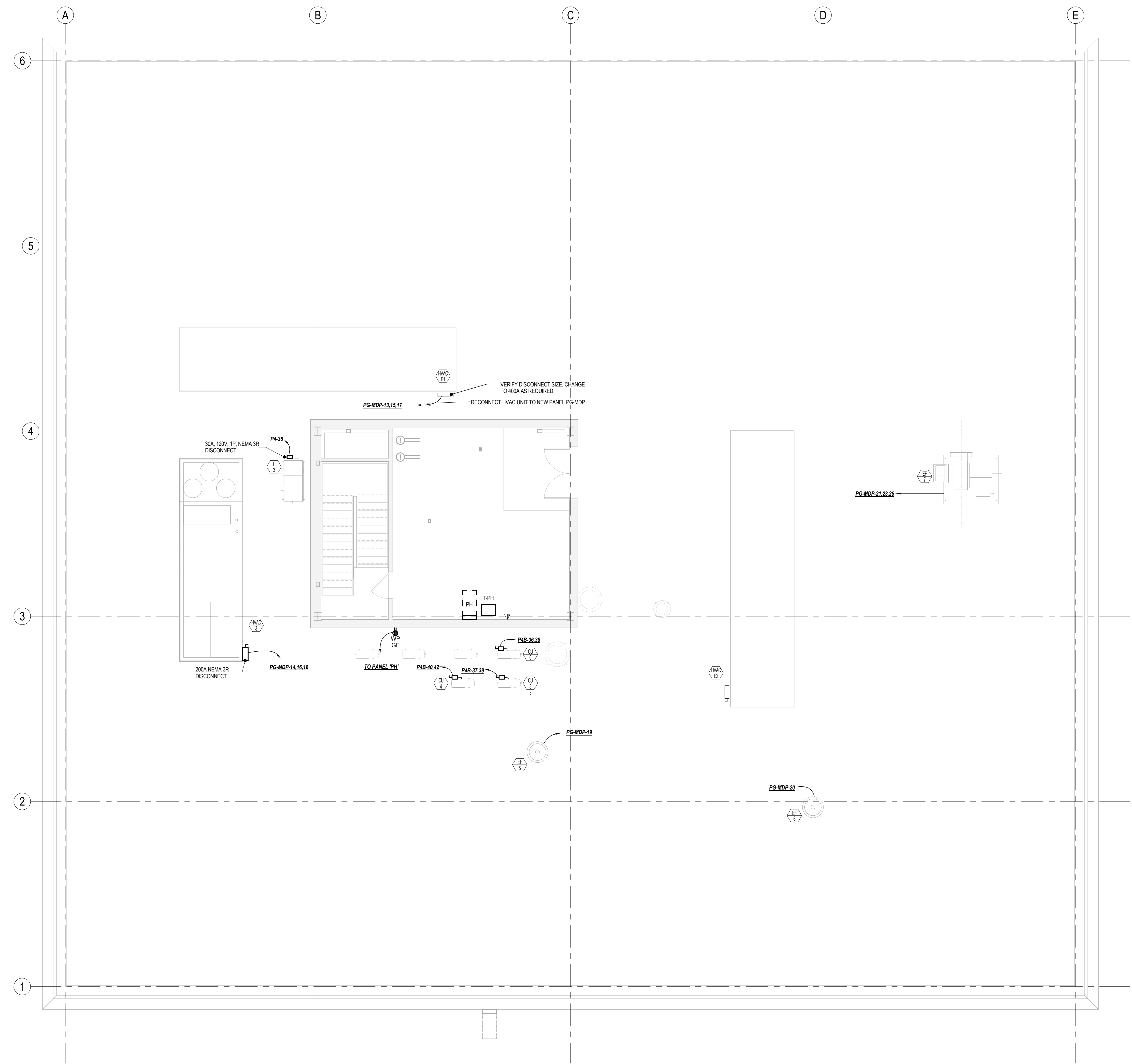
ELECTRICAL POWER LEVEL ROOF / PENTHOUSE NEW PLAN 3/16" = 1'-0"
