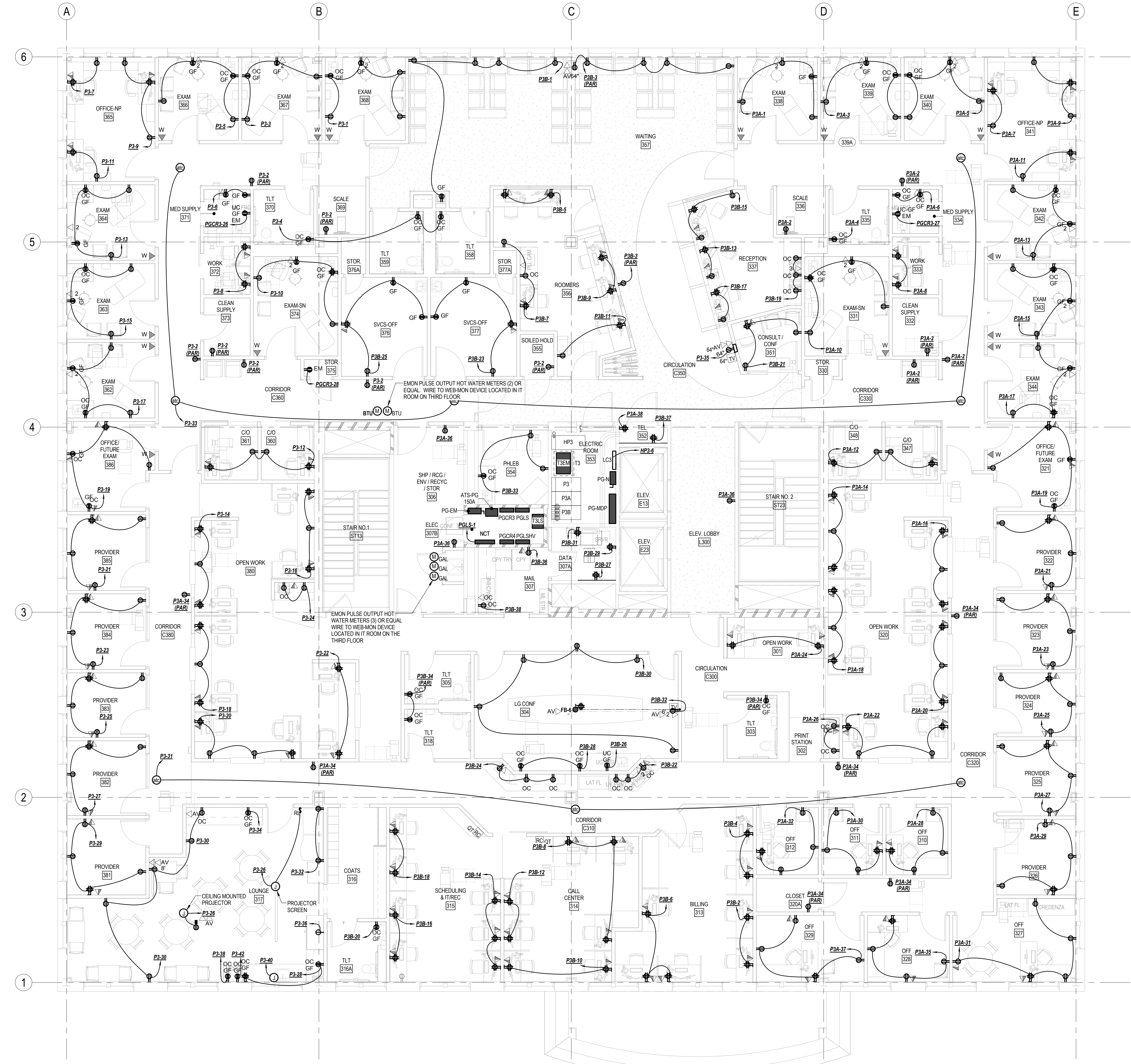
1 ELECTRICAL POWER LEVEL 3 NEW PLAN 3/16" = 1'-0"
