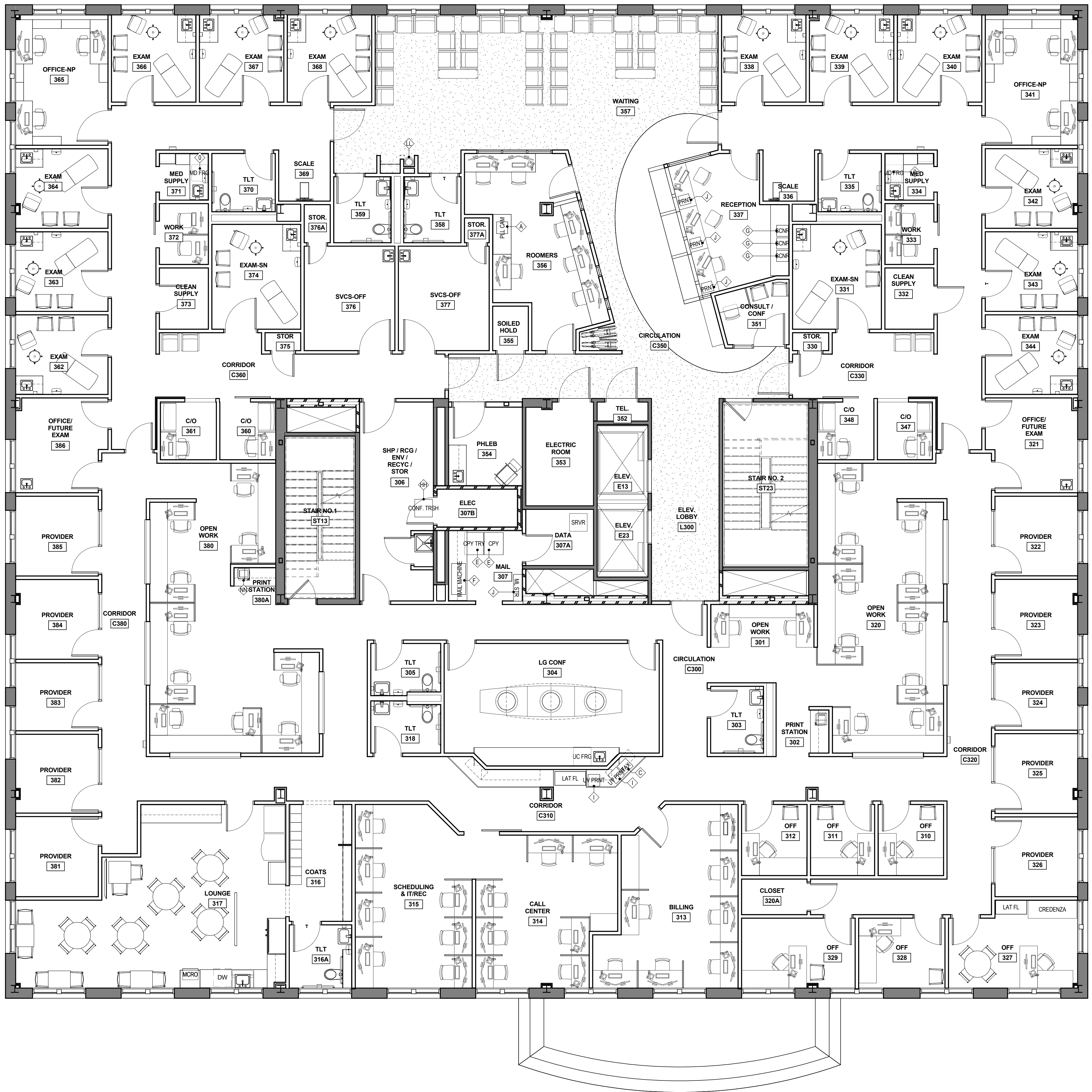
LEVEL 3 - EQUIPMENT AND FURNISHINGS 3/16" = 1'-0"
