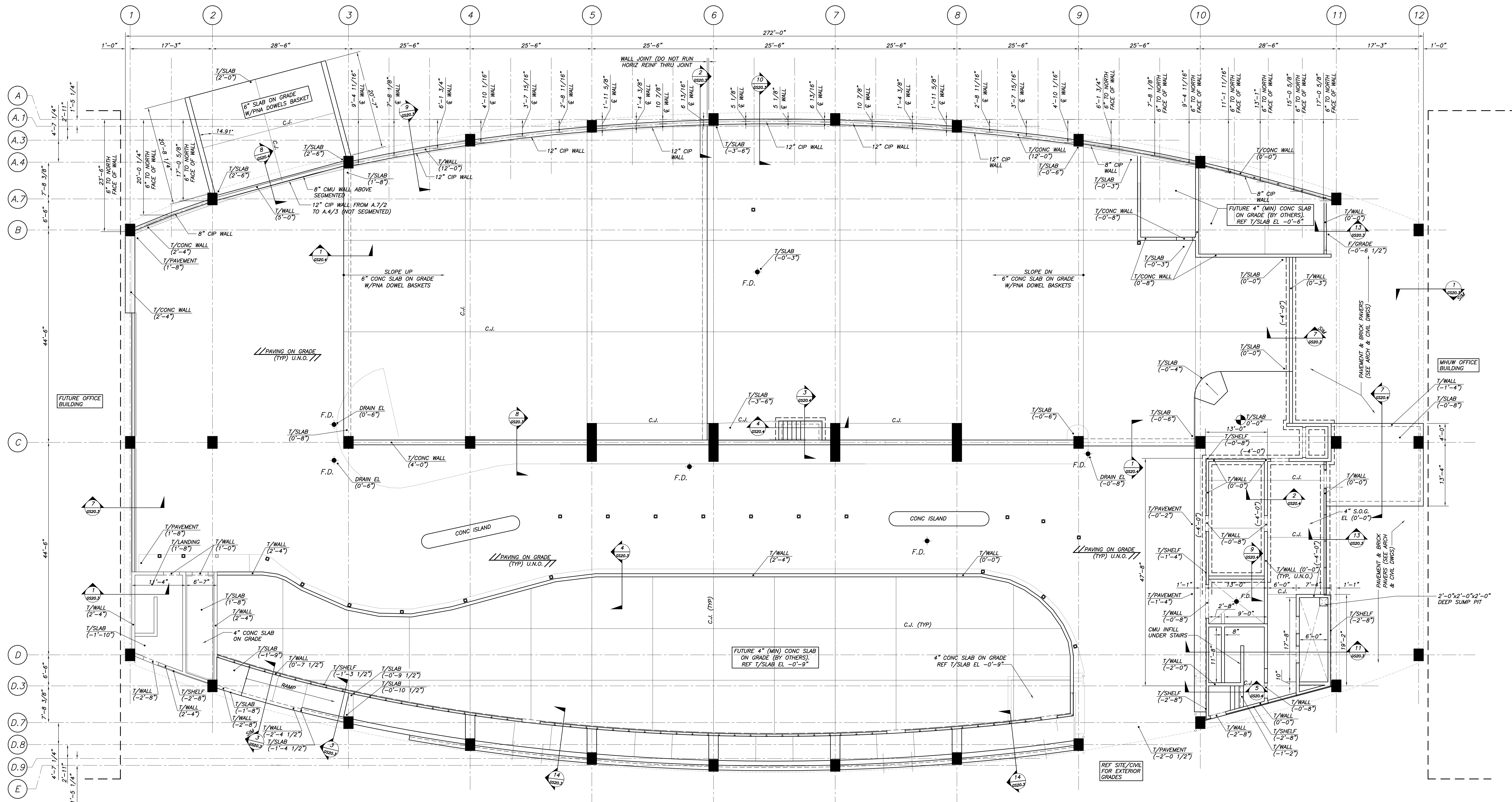
GROUND LEVEL SLAB PLAN 1/8" = 1'-0" TOP OF SLAB EL. 0'-0" = REF. EL. 11.00'
