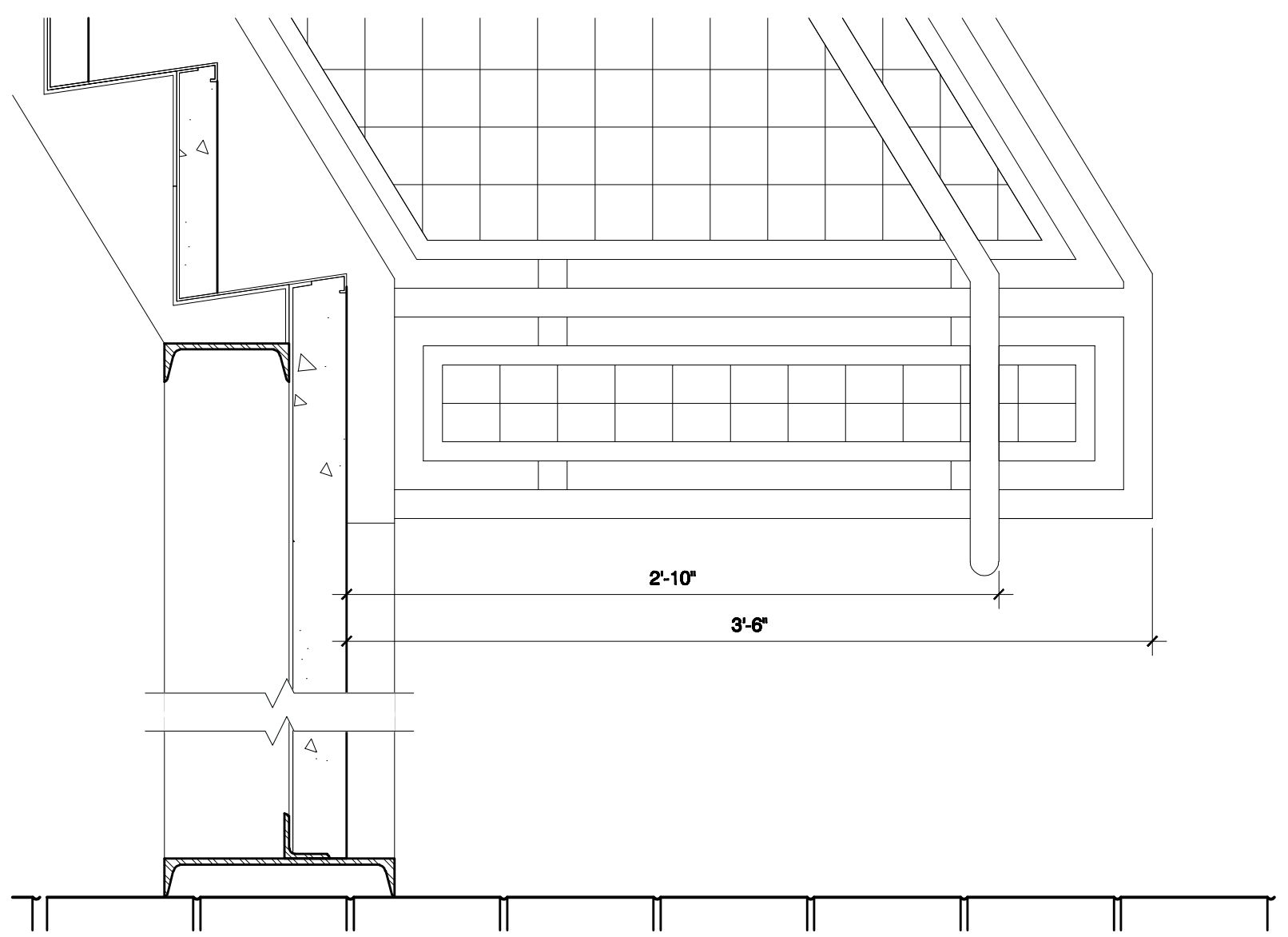
STAIR — TOP LANDING GUARDRAIL DETAIL 1/2" = 1'-0" REF: 7
