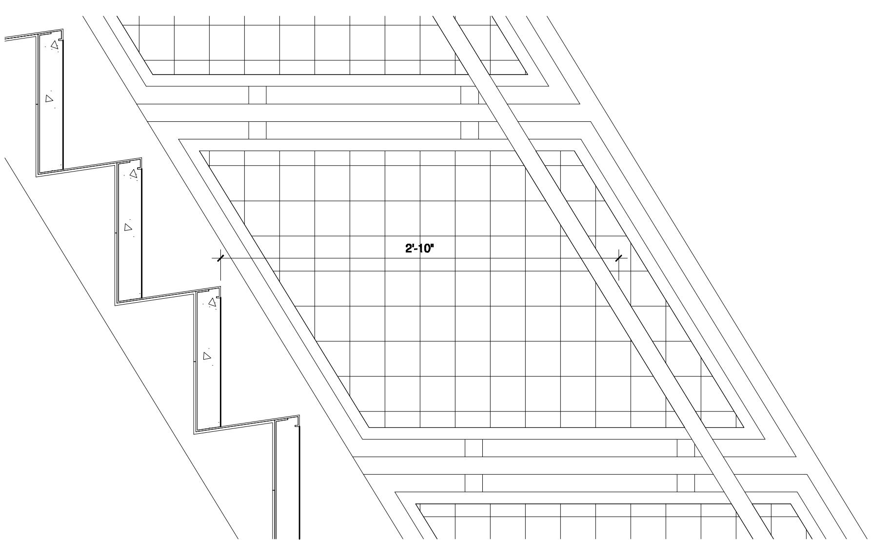
STAIR — GUARDRAIL DETAIL 1/2" = 1'-0" REF: 6
