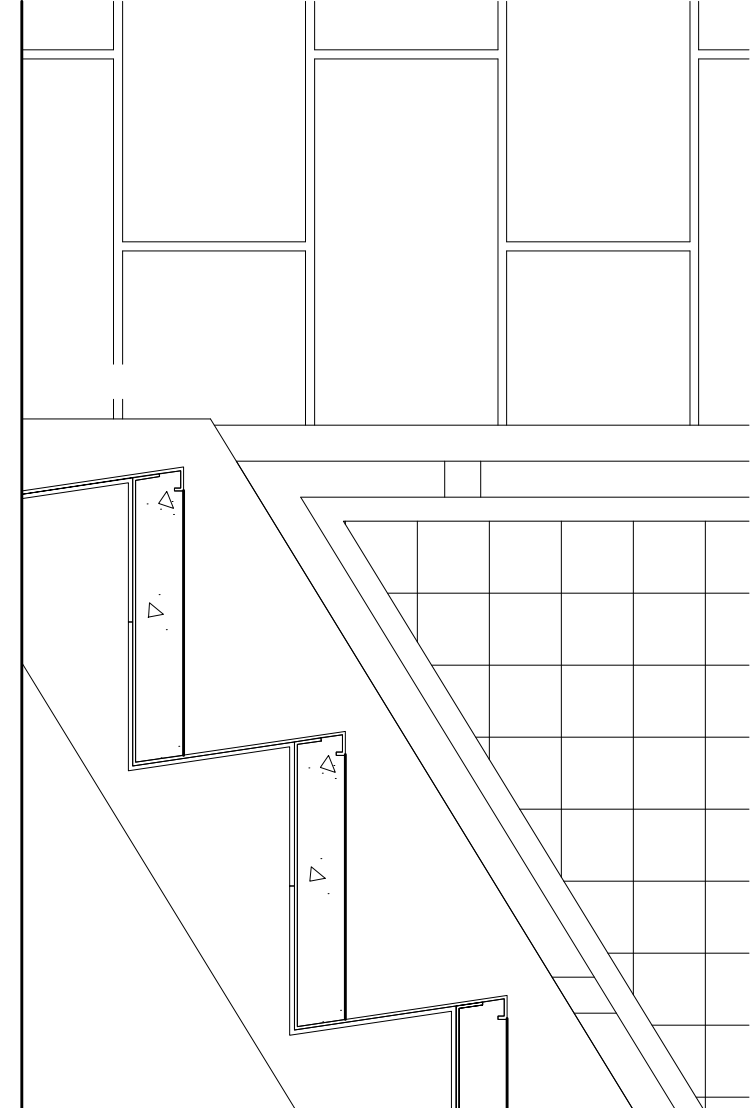
STAIR — GUARDRAIL DETAIL 1/2" = 1'-0" REF: 6
