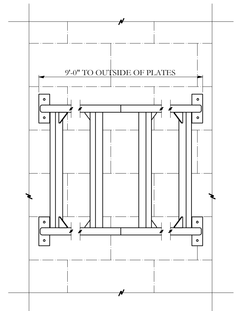
SECTION B SK-2 3/4"=1'-0
