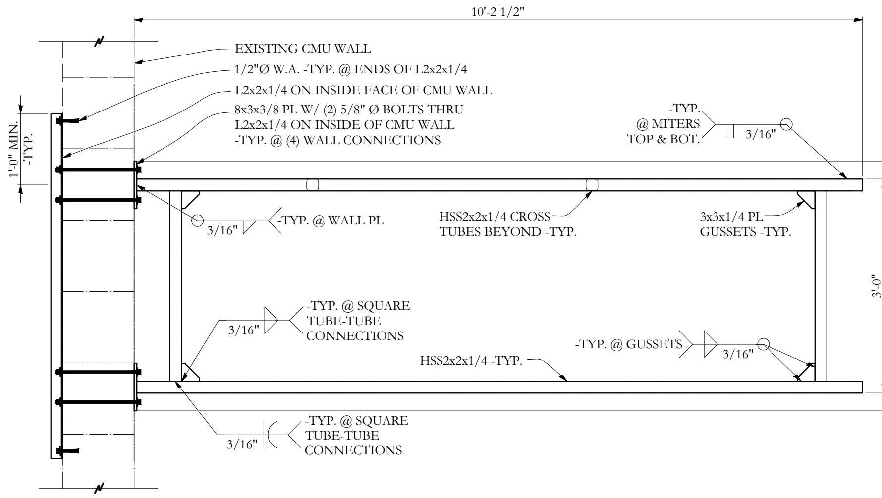
SECTION A SK-2 3/4"=1'-0
