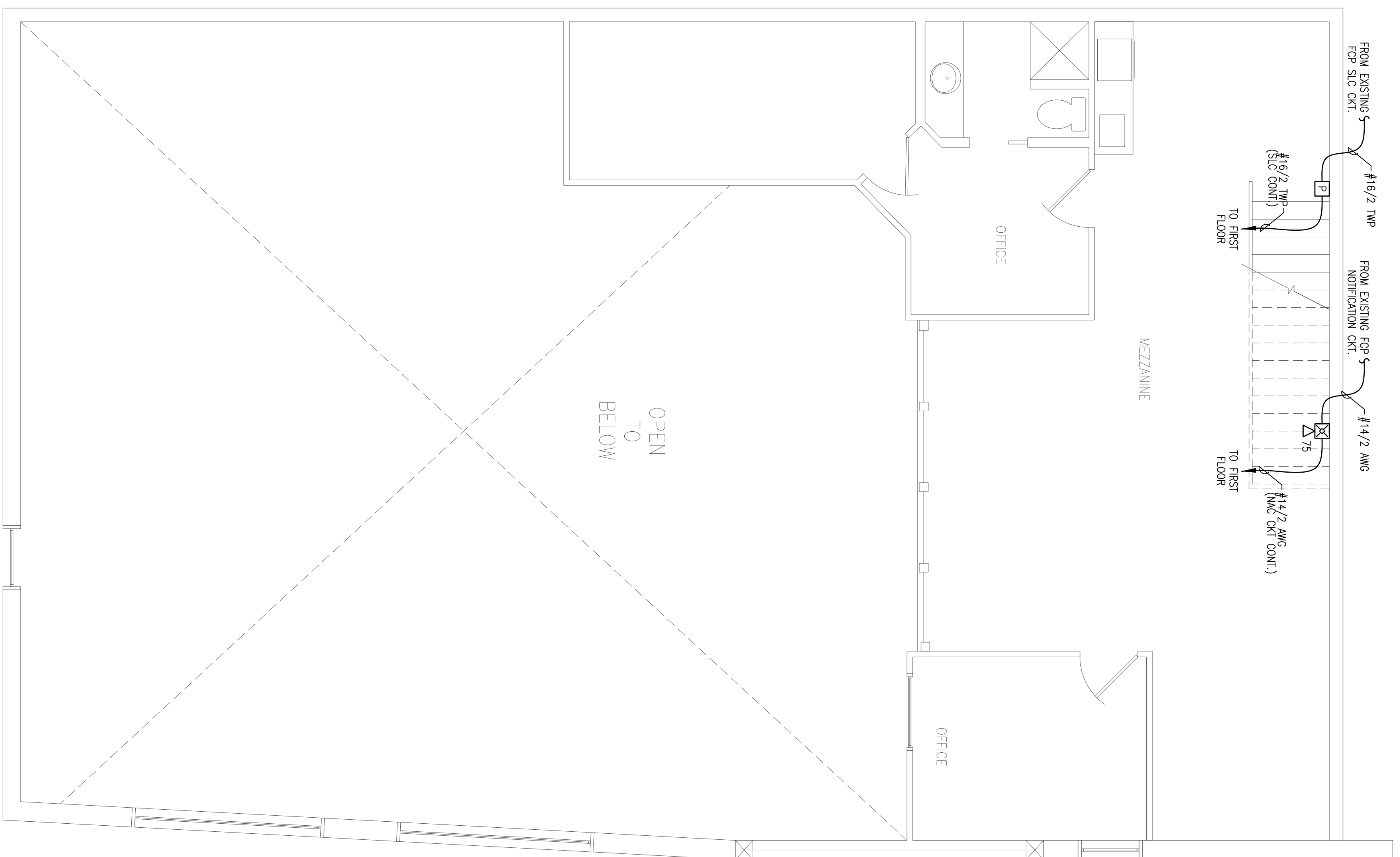
MEZZANINE FIRE ALARM PLAN SCALE: 1/4"=1'-0"
