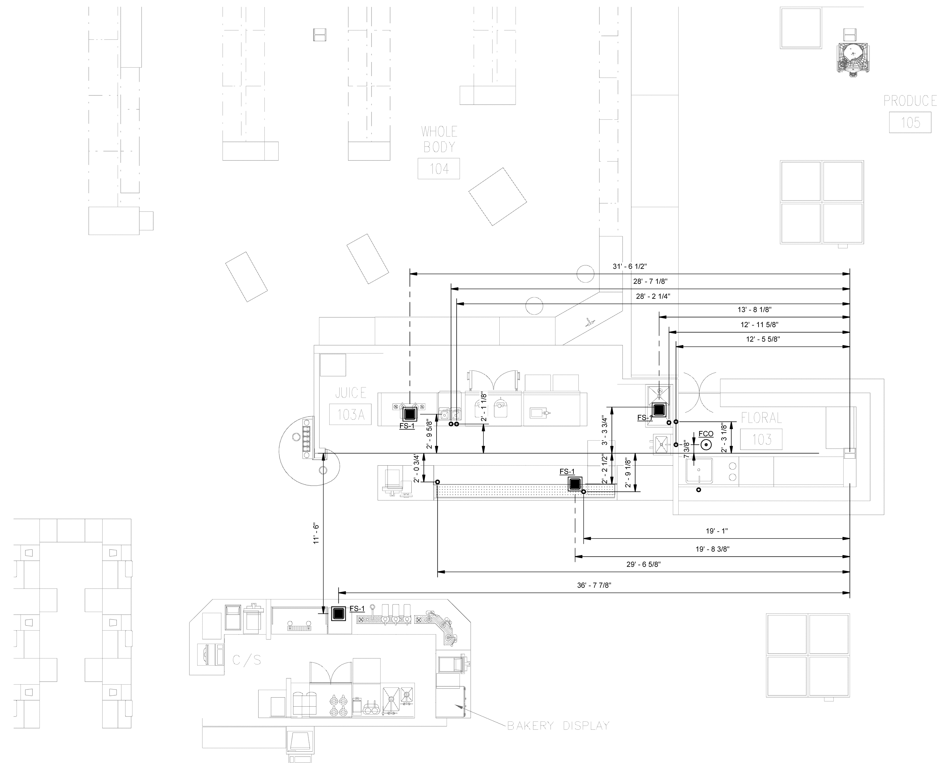
1 PUB DRAINAGE DIMENSION PART-PLAN
