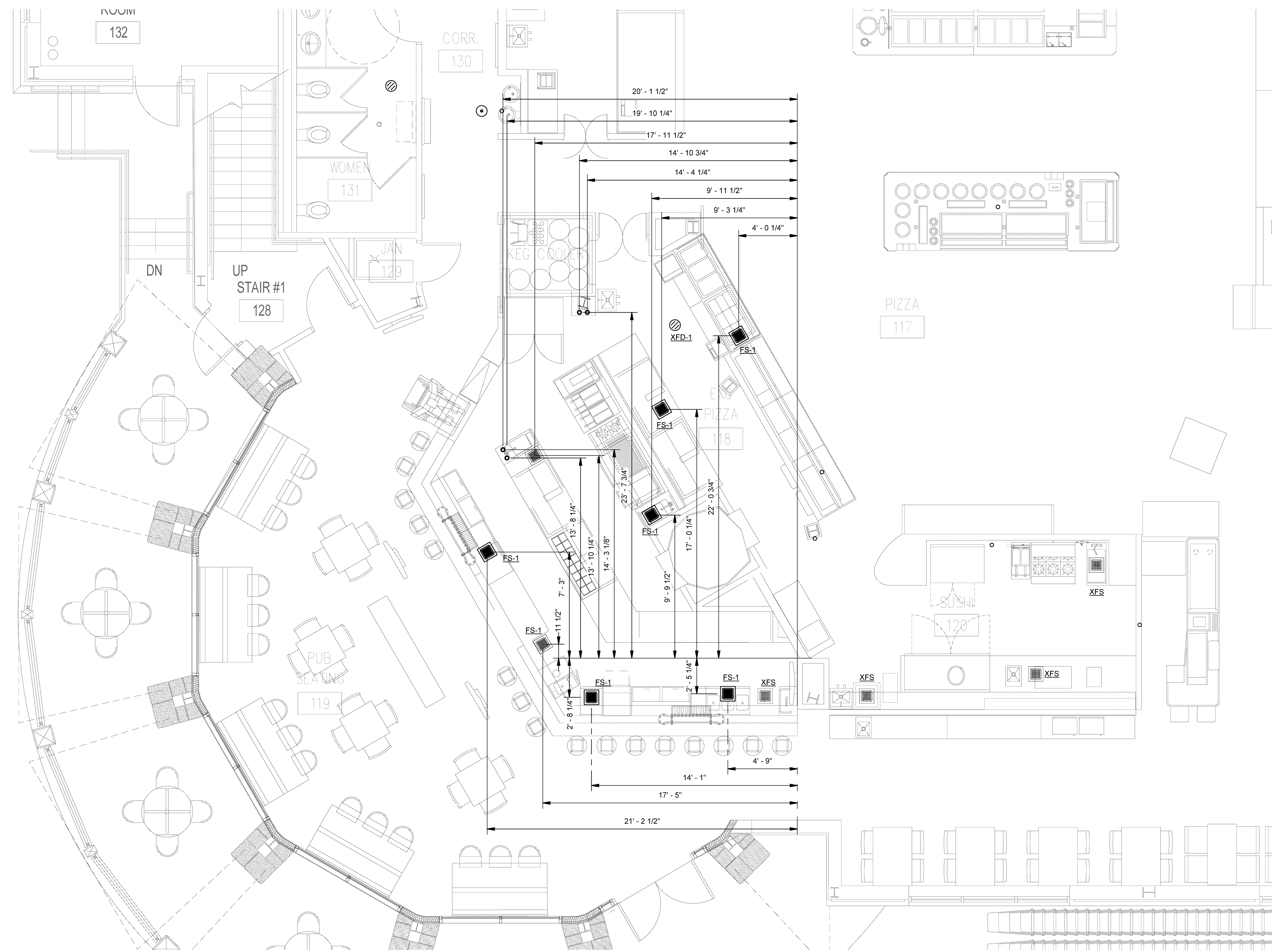
1 PUB DRAINAGE DIMENSION PART-PLAN
