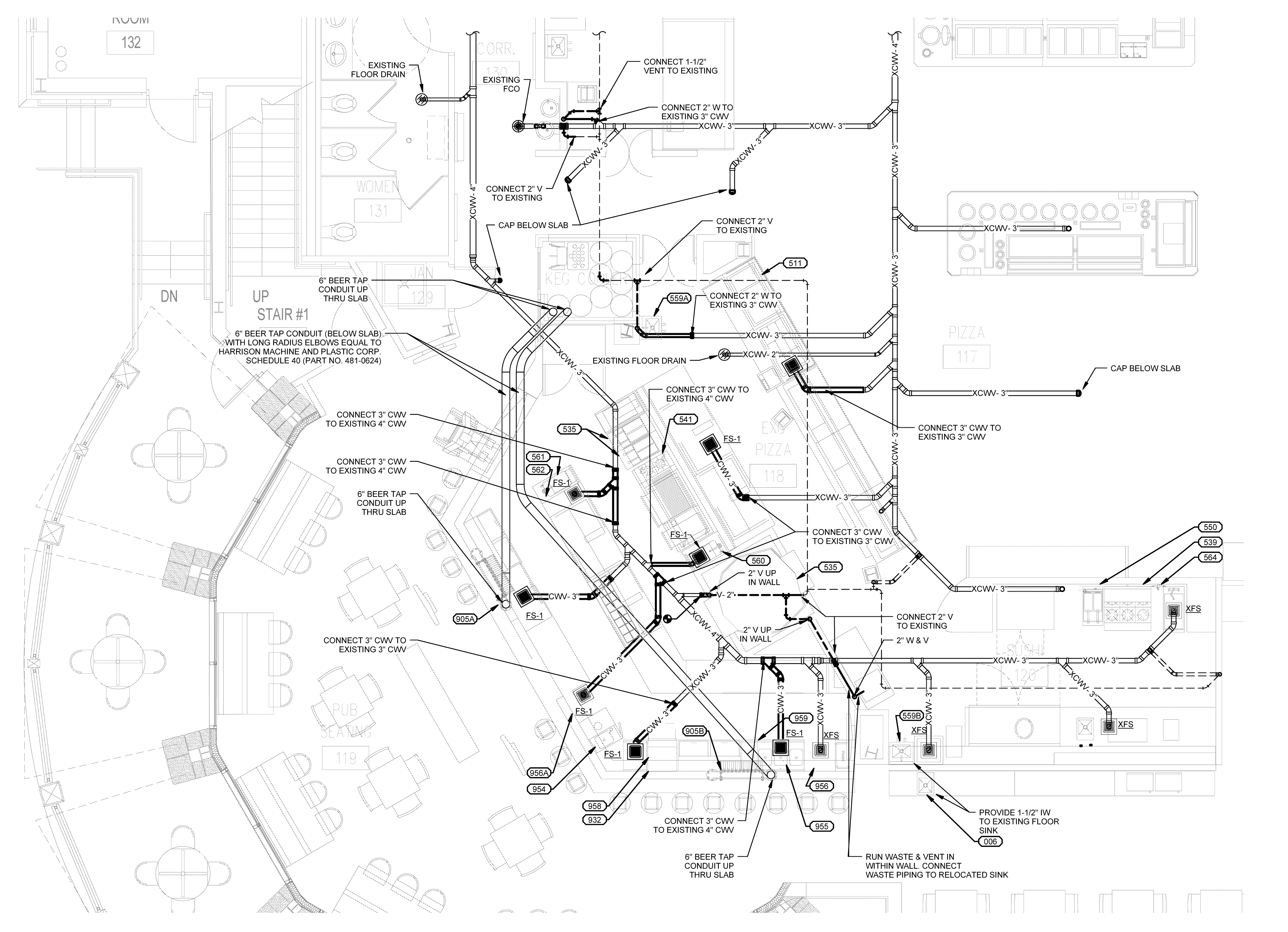
1 PUB DRAINAGE PART-PLAN SCALE: 1/4" = 1'-0"
