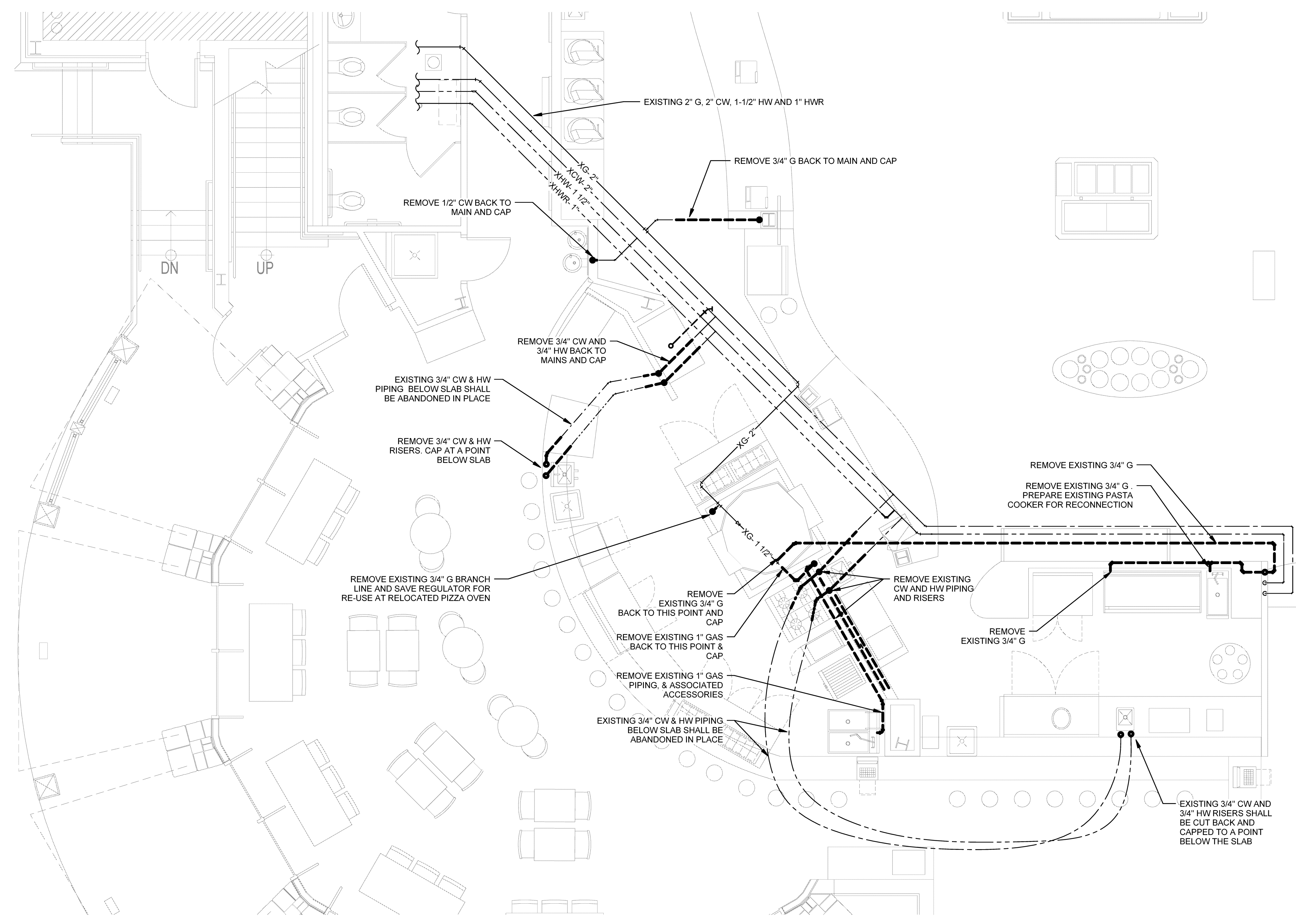
4 DEMOLITION SUPPLY PLAN SCALE: 1/4" = 1'-0"
