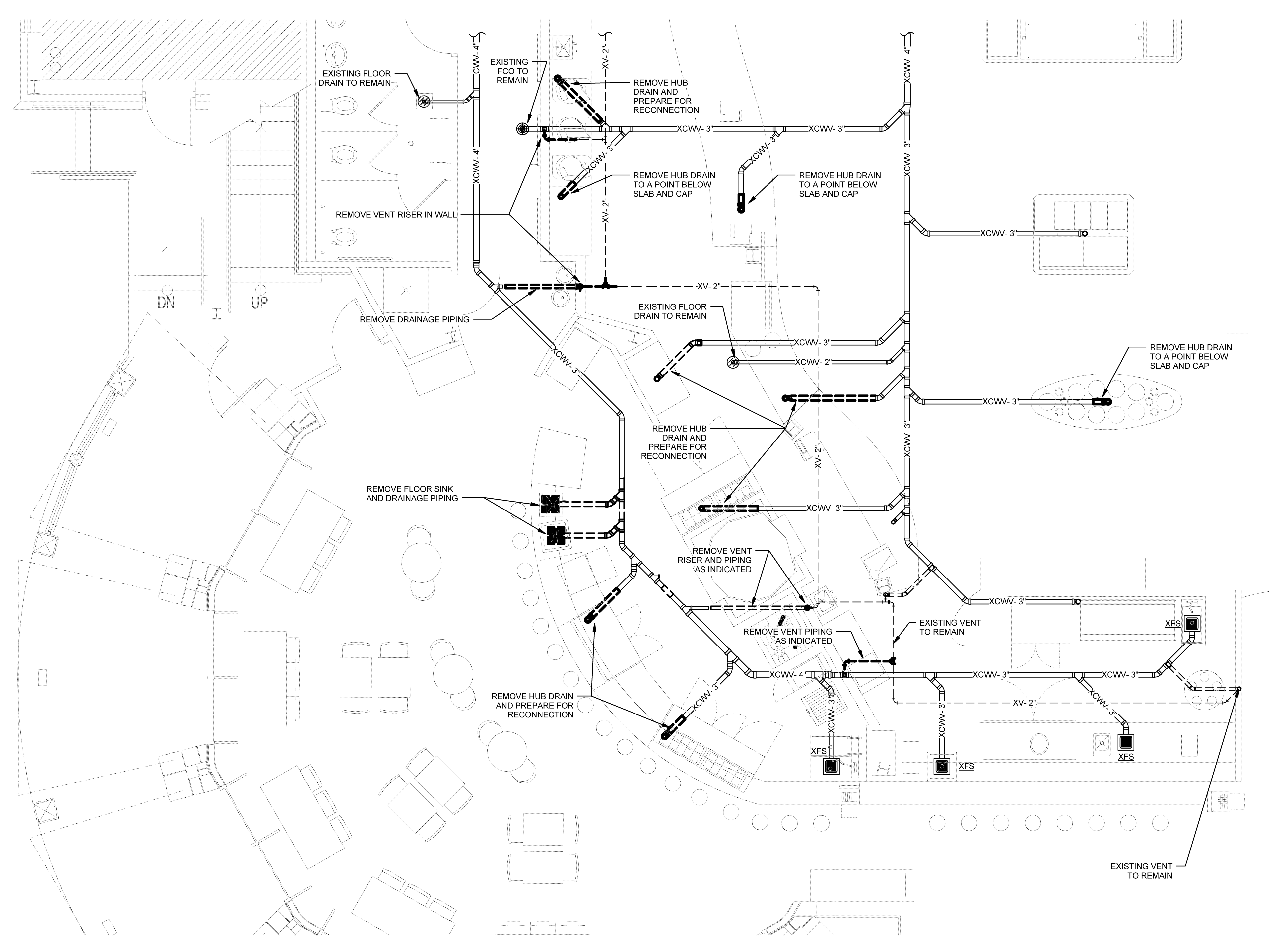
3 DEMOLITION DRAINAGE PLAN SCALE: 1/4" = 1'-0"
