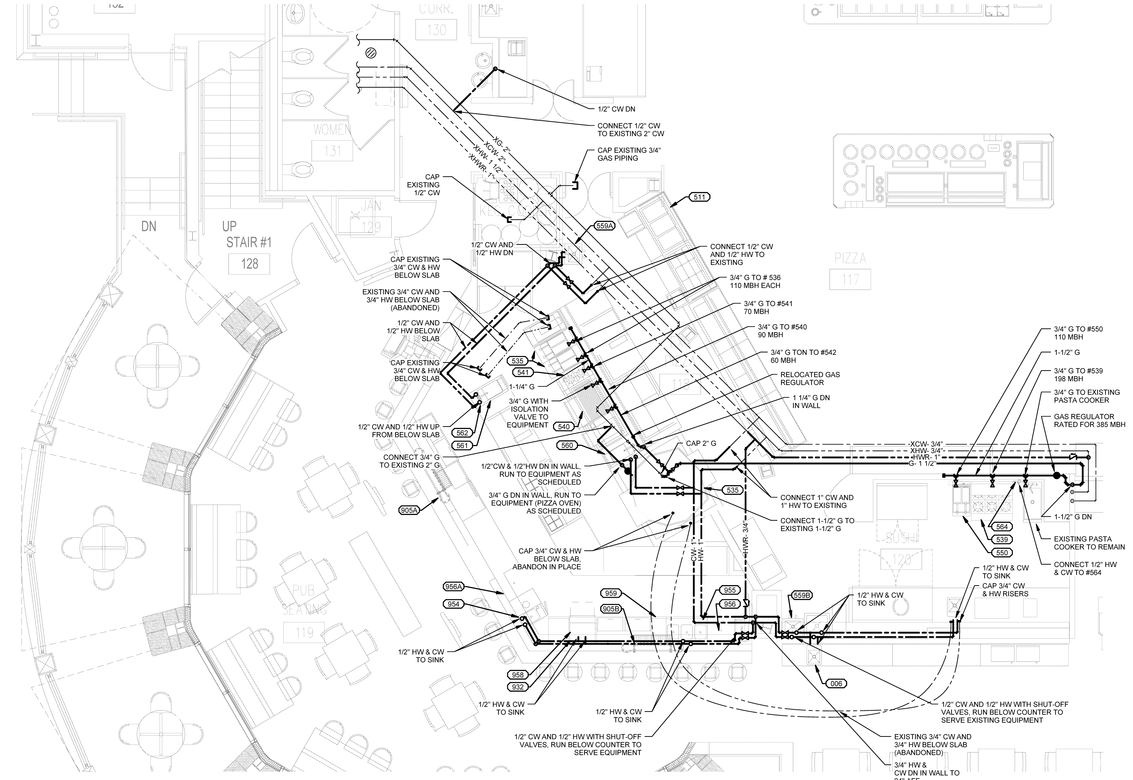
2 PUB SUPPLY PART-PLAN SCALE: 1/4" = 1'-0"
