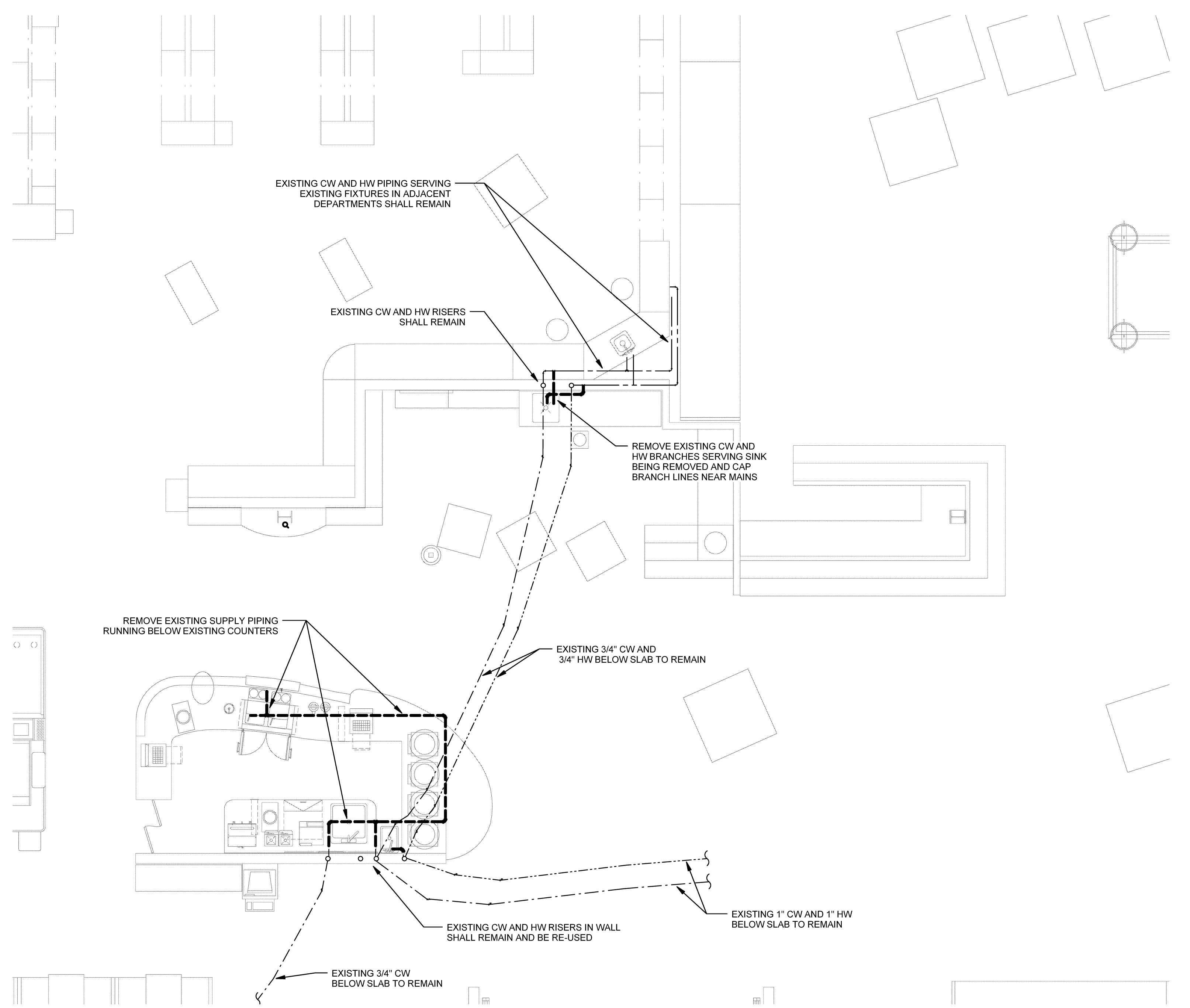
4 DEMOLITION SUPPLY PLAN SCALE: 1/4" = 1'-0"
