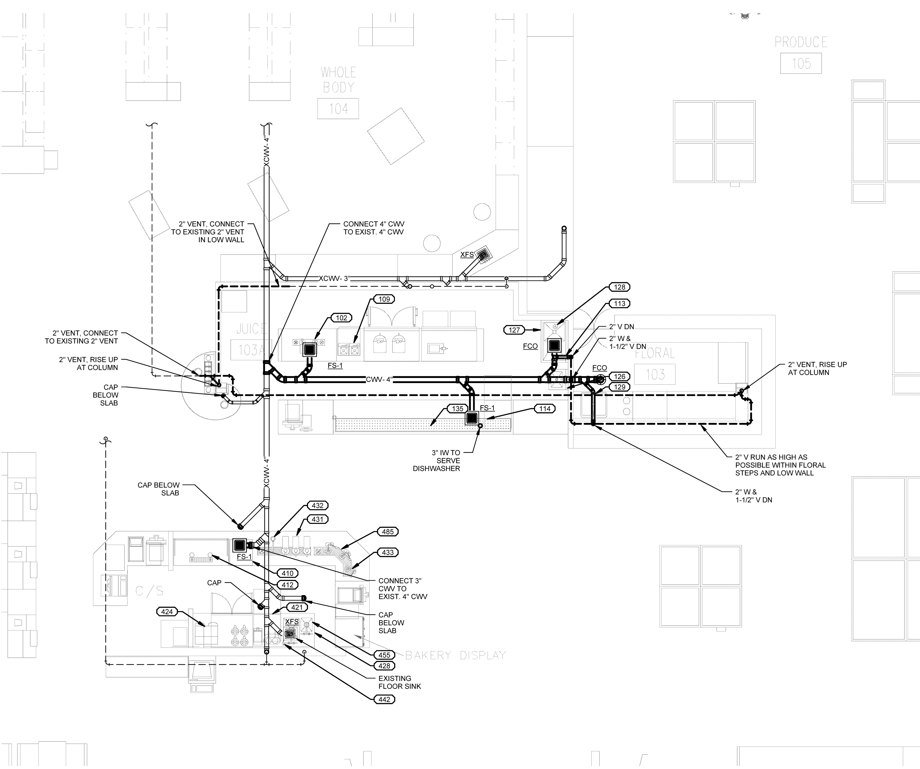
1 JUICE DRAINAGE PART-PLAN SCALE: 1/4" = 1'-0"
