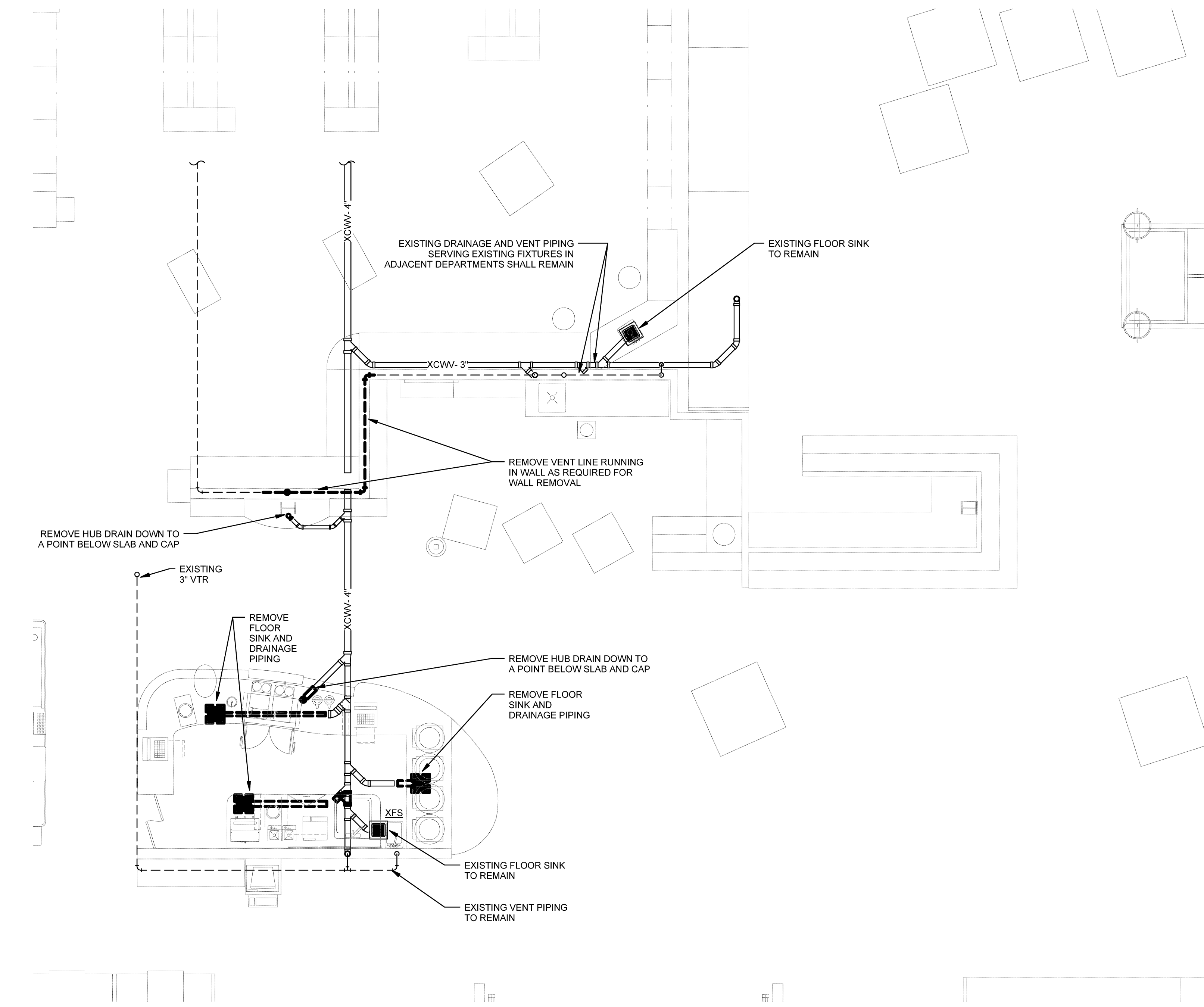
3 DEMOLITION DRAINAGE PLAN SCALE: 1/4" = 1'-0"
