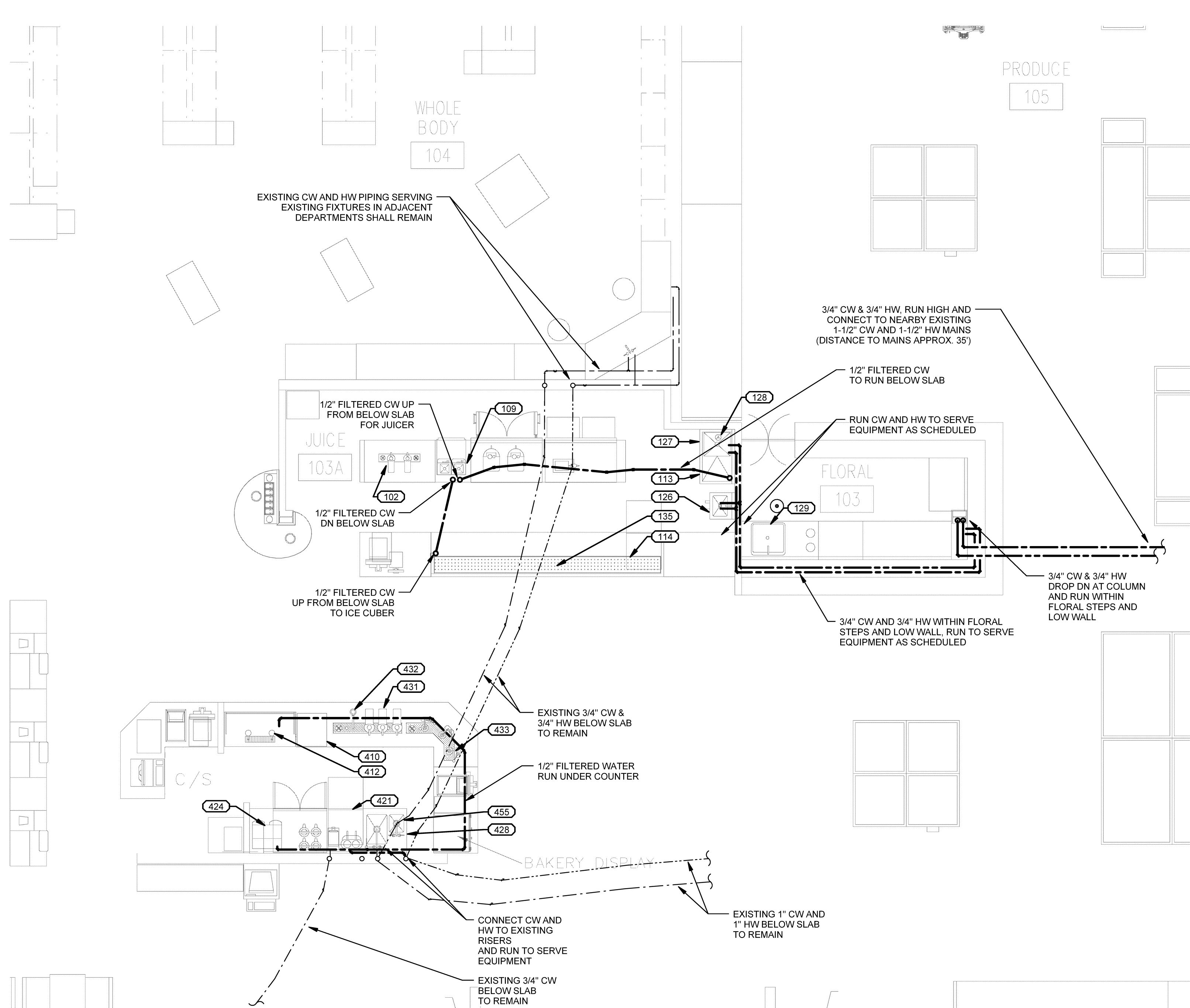
2 JUICE SUPPLY PART-PLAN SCALE: 1/4" = 1'-0"
