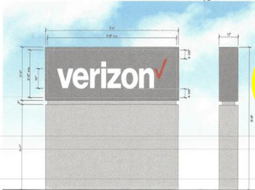
C FRONT VIEW - 16 SF Scale: 3/16" = 1'-0"
