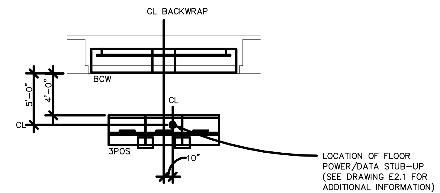
3POS DIAGRAM
