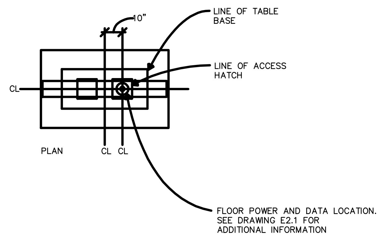
2 HTVE SHELF: DATA / MUD RING / RECEPTACLE E3.2 N.T.S
