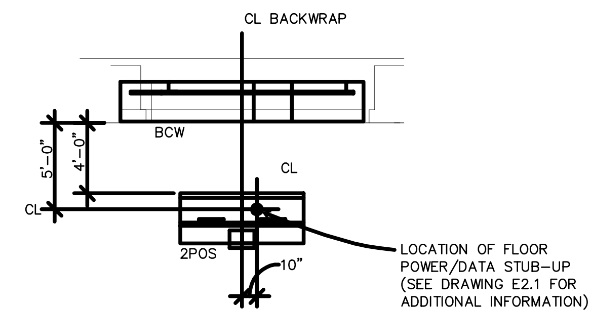
5 POS POWER/DATA DETAIL E3.2 N.T.S
