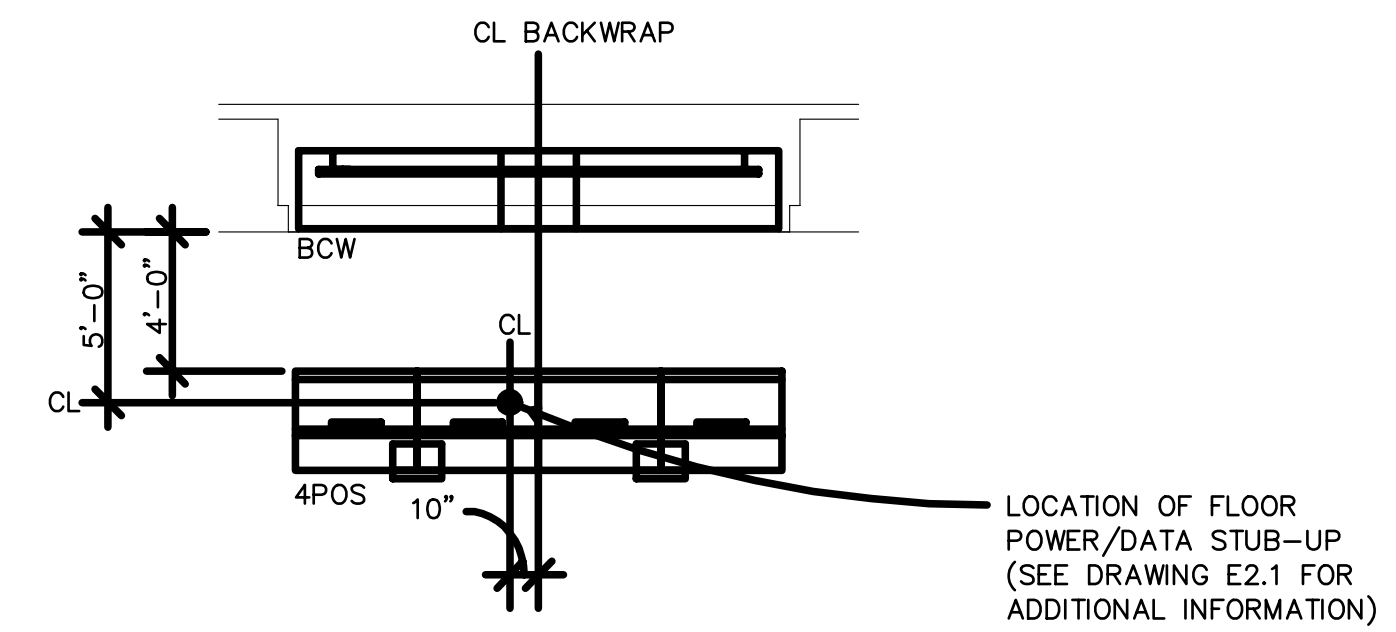
4POS DIAGRAM
