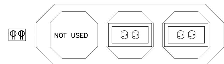
2 HTVE SHELF: DATA / MUD RING / RECEPTACLE E3.2 N.T.S
