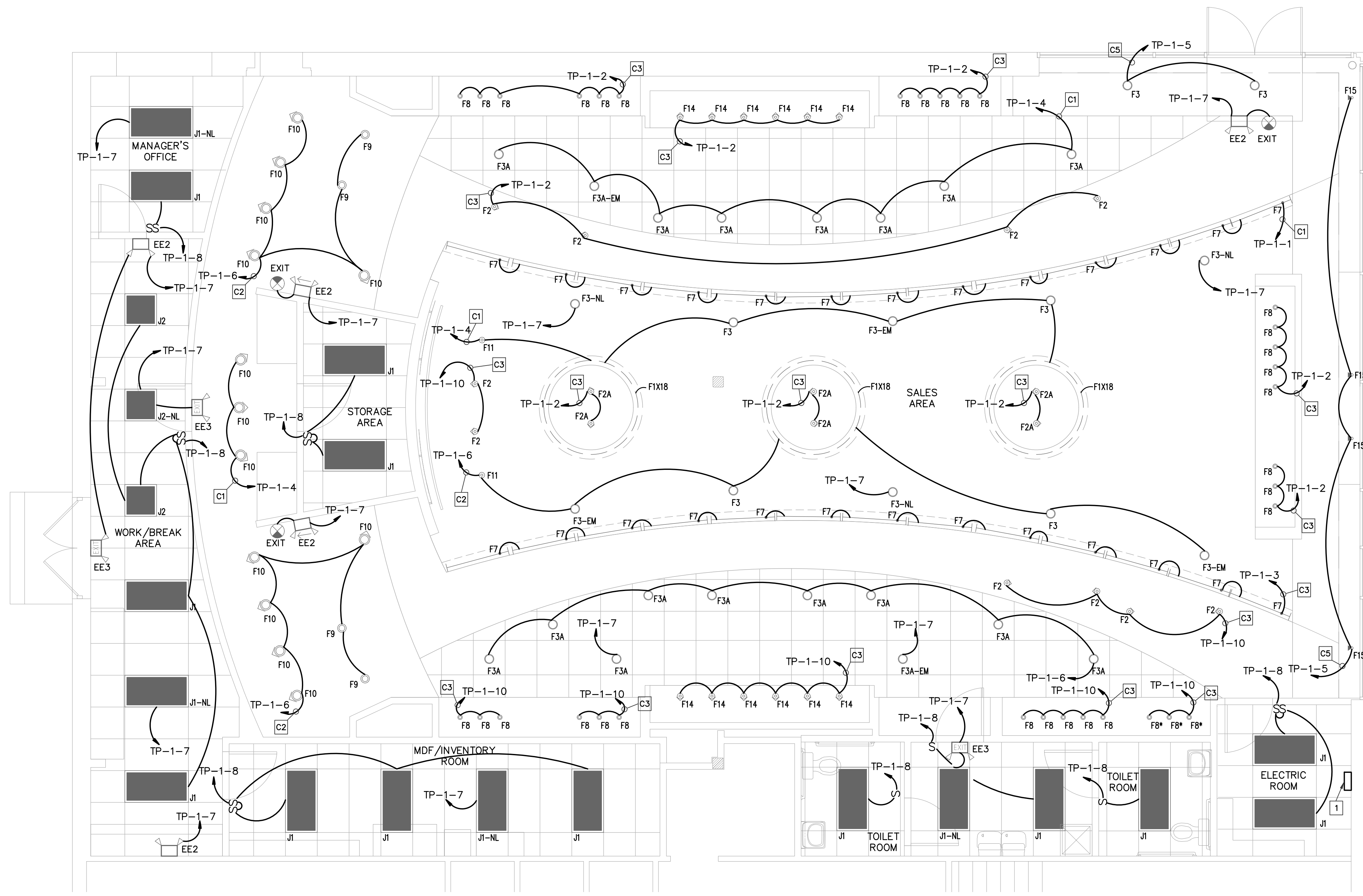
1 LIGHTING PLAN E2.2
