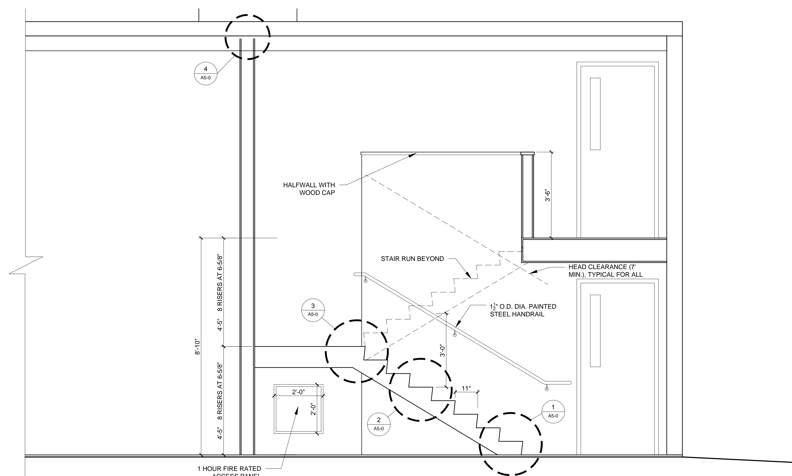
2 SECTION VIEW THROUGH MEZZANINE 1/2" = 1'-0"
