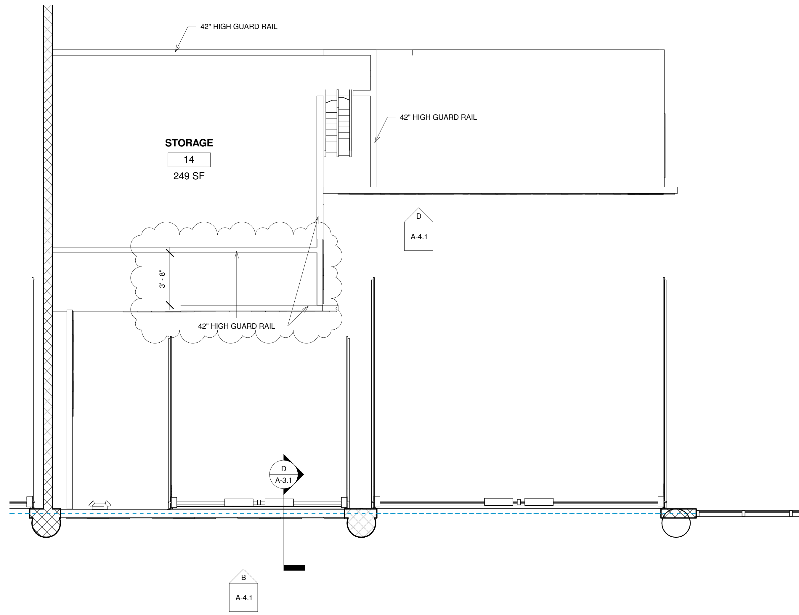
A MEZZANINE 1/4" = 1'-0"
