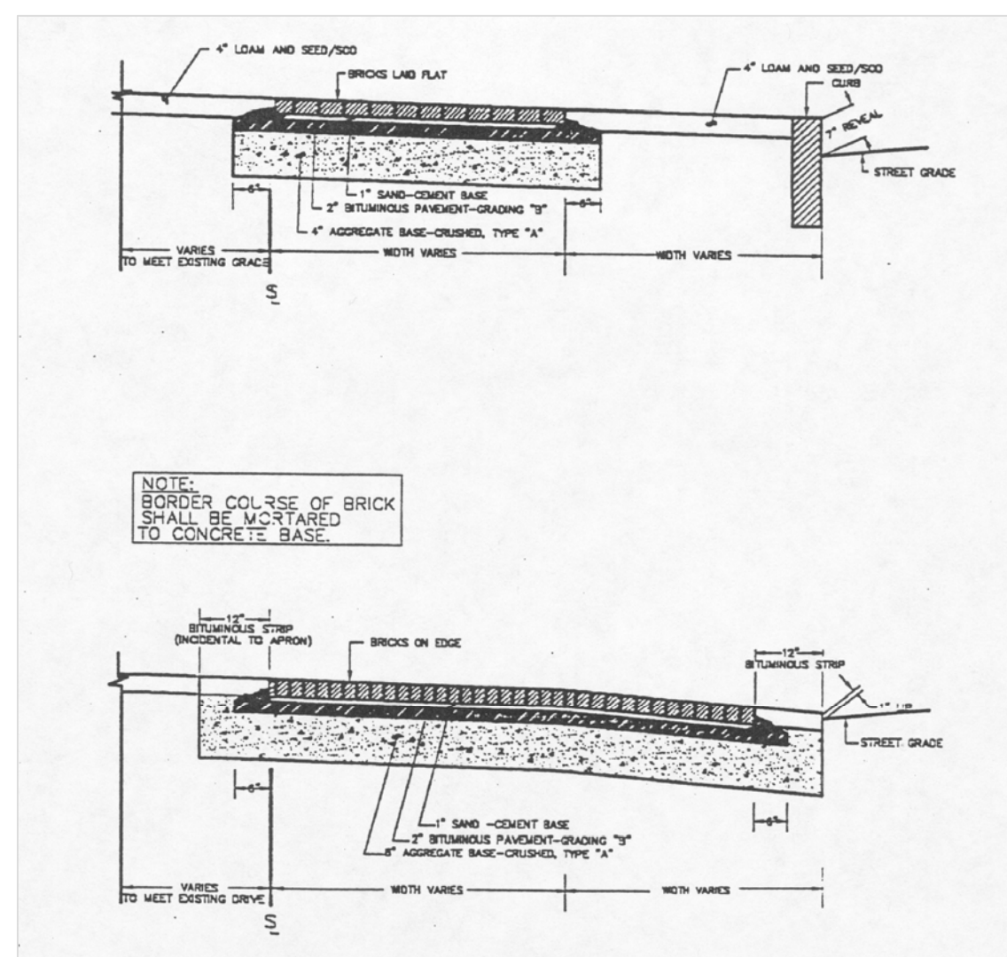
9 BRICK WITH BITUMINOUS BASE SIDEWALK AND DRIVEWAY CONSTRUCTION NOT TO SCALE
