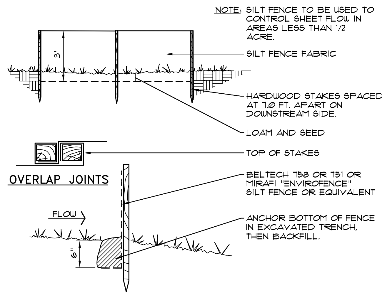
5 SILT FENCE DETAIL NOT TO SCALE
