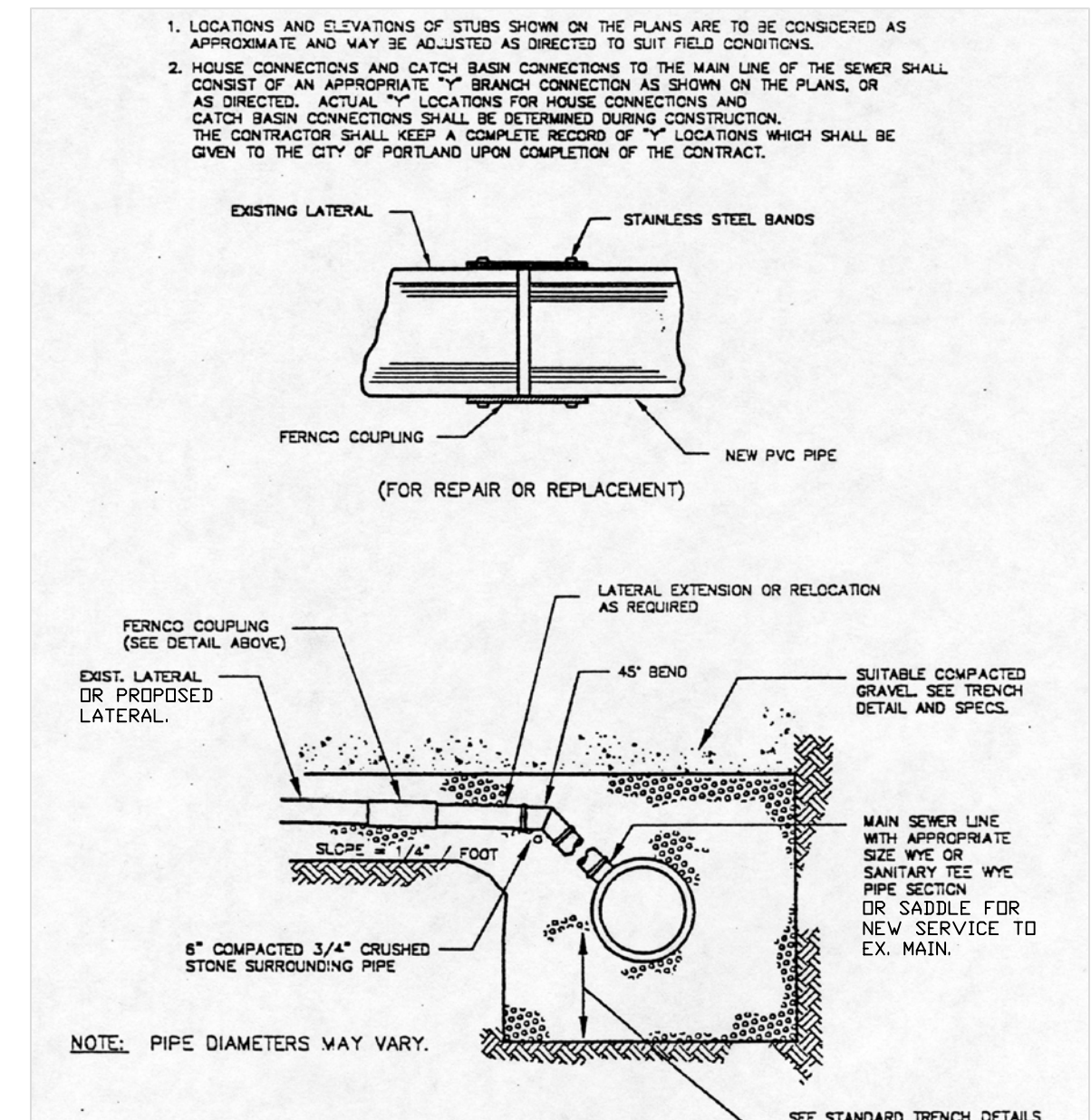
6 TYP. EXISTING LATERAL CONNECTION NOT TO SCALE
