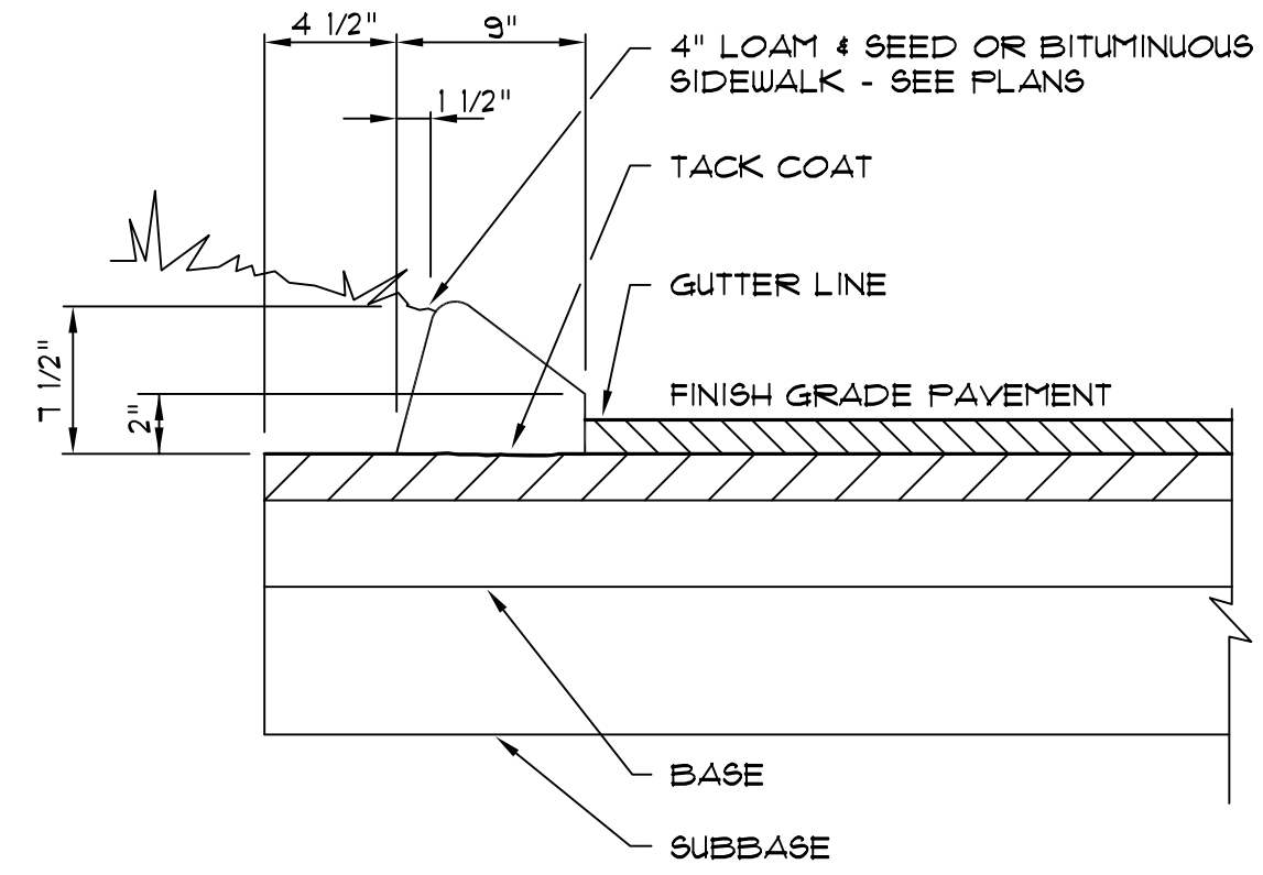
4 SLOPED BITUMINOUS CURB DETAIL NOT TO SCALE
