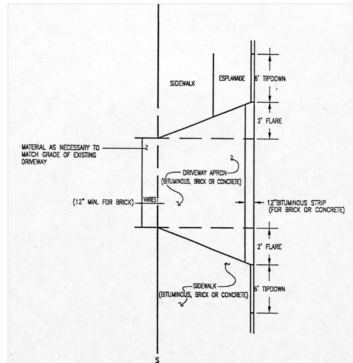
8 SIDEWALK & DRIVEWAY CONSTRUCTION NOT TO SCALE
