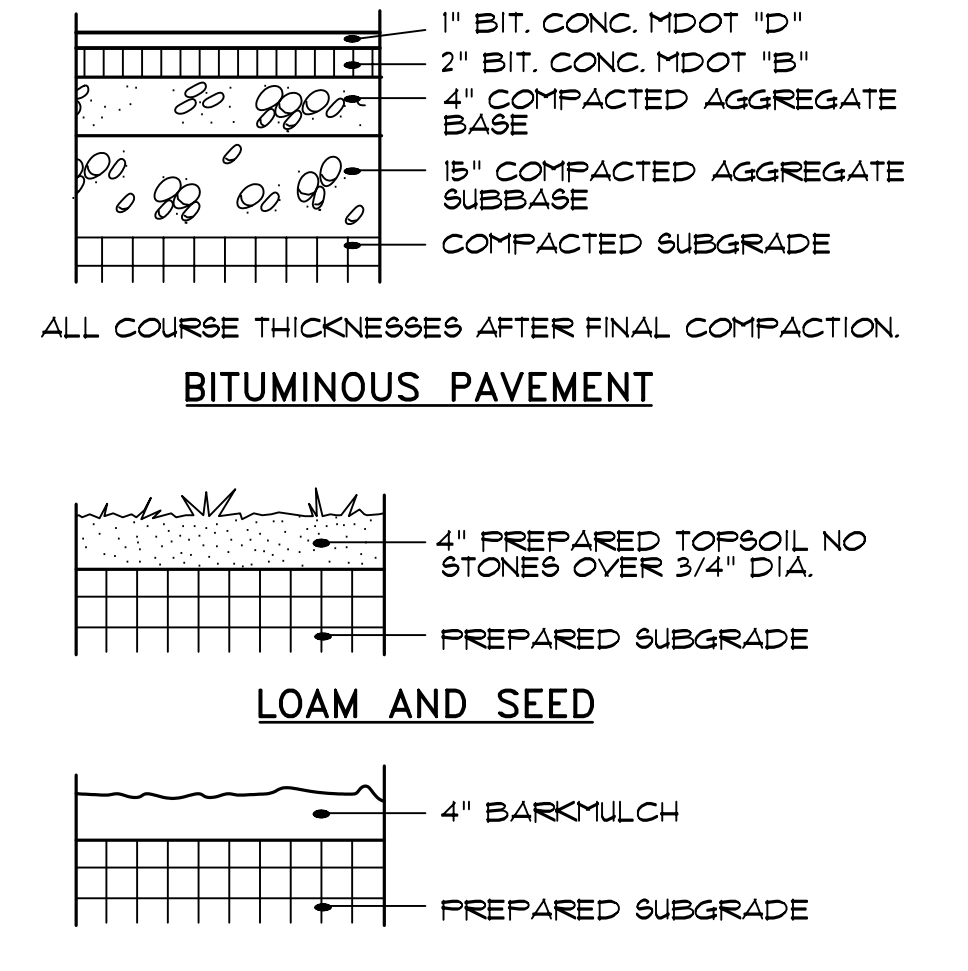
1 SURFACING DETAILS NOT TO SCALE
