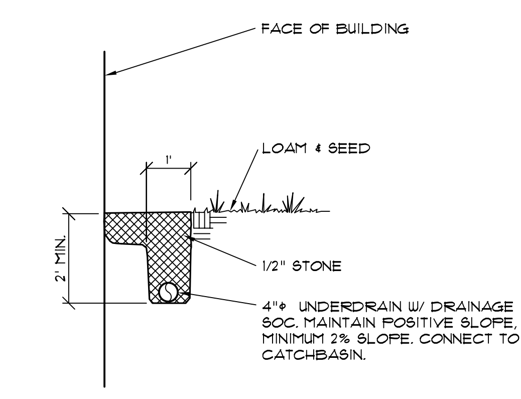
3 STONE DRIPSTRIP SECTION NOT TO SCALE
