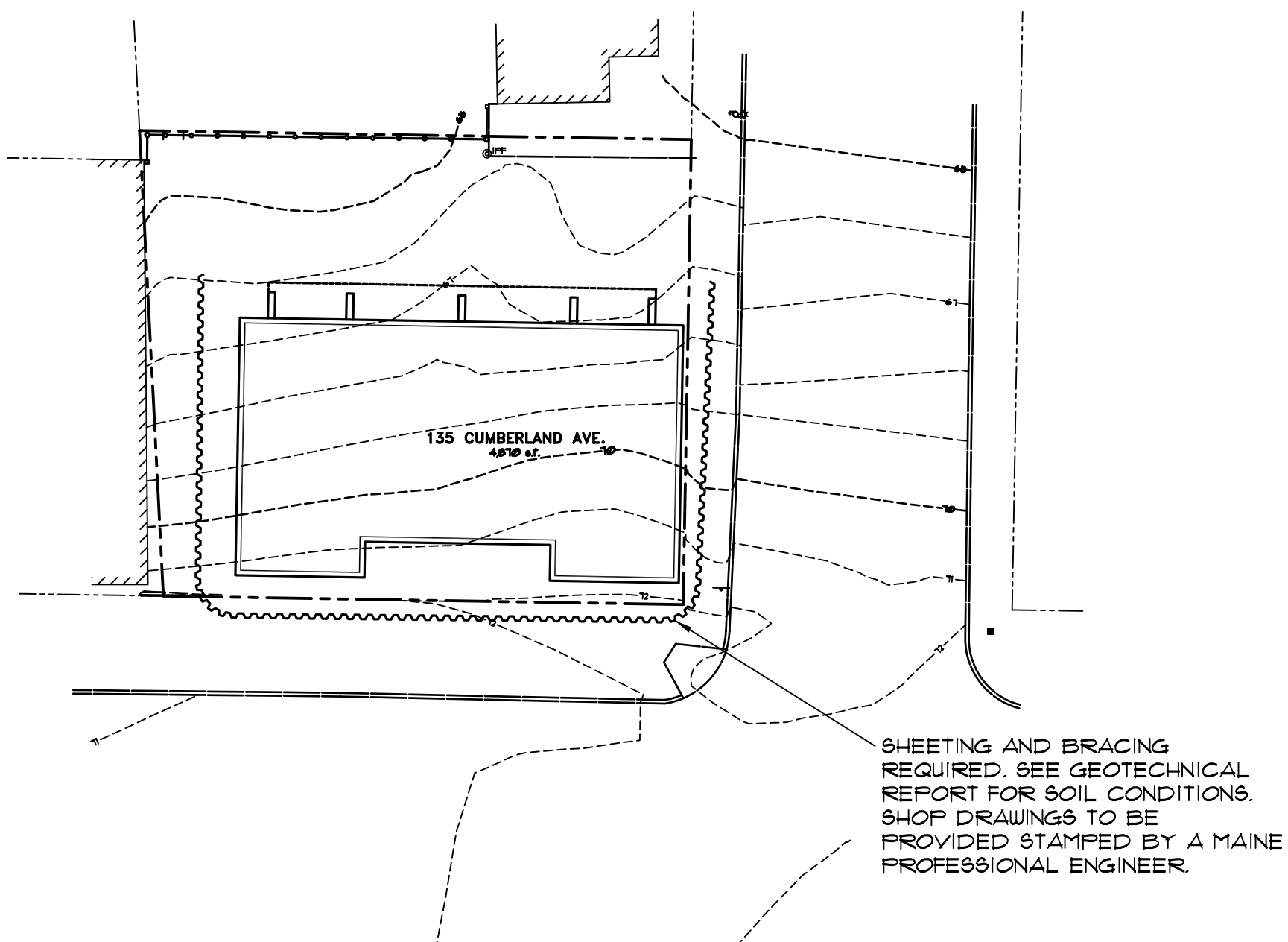
12 SHORING PLAN SCALE: 1"=20'
