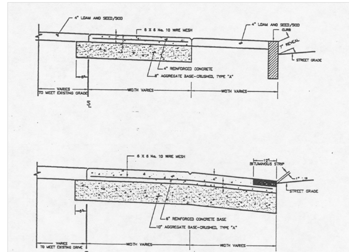
7 CONCRETE SIDEWALK AND DRIVEWAY CONSTRUCTION NOT TO SCALE
