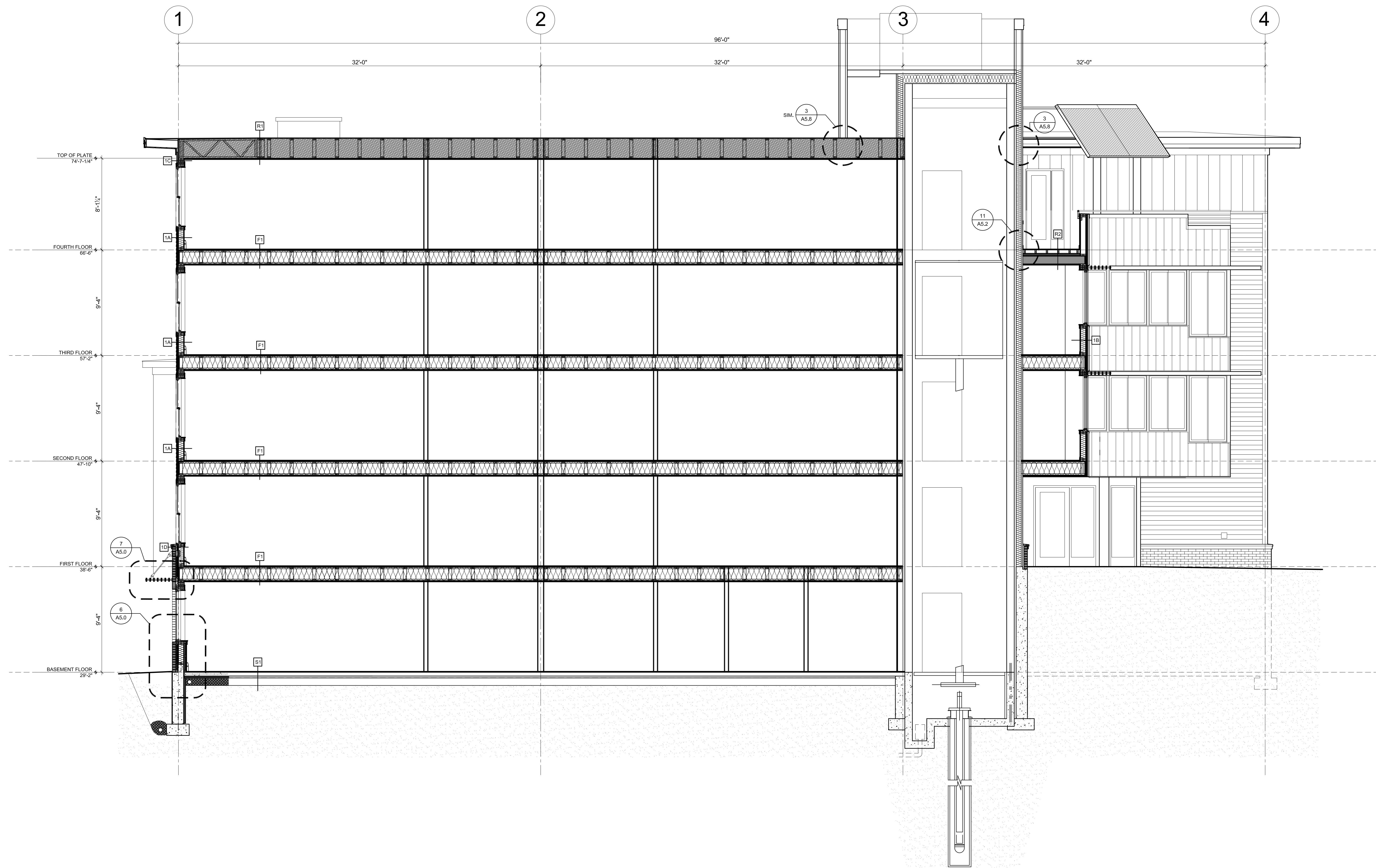
1 SECTION A3.1 1/4" = 1'-0"
