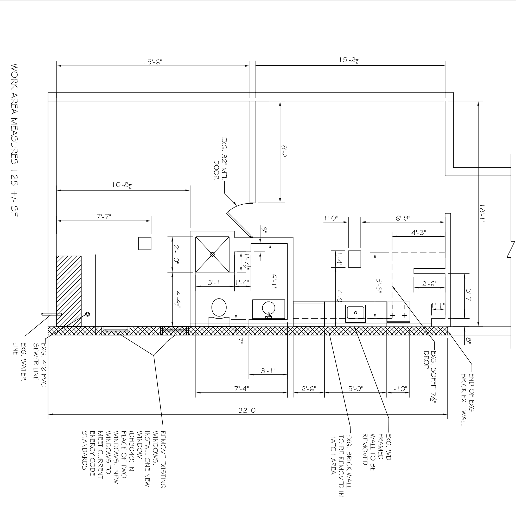
B3 EXG. BASEMENT PLAN SCALE: 1/2" = 1'-0"
