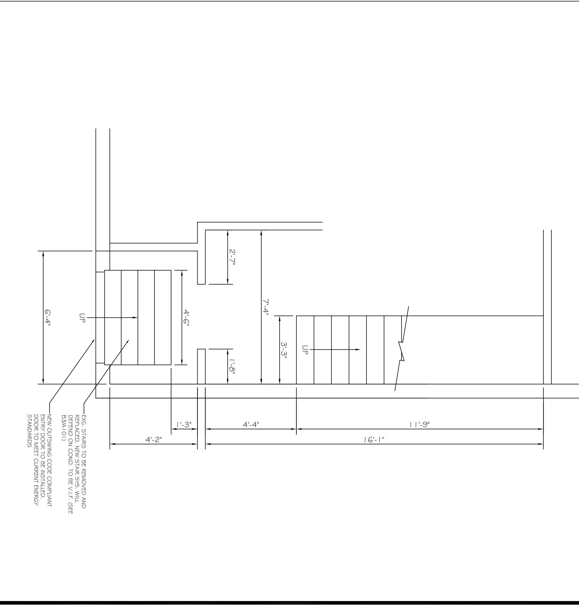
B1 EXG. FIRST FLOOR ENTRY STAIR PLAN SCALE: 3/8" = 1'-0"
