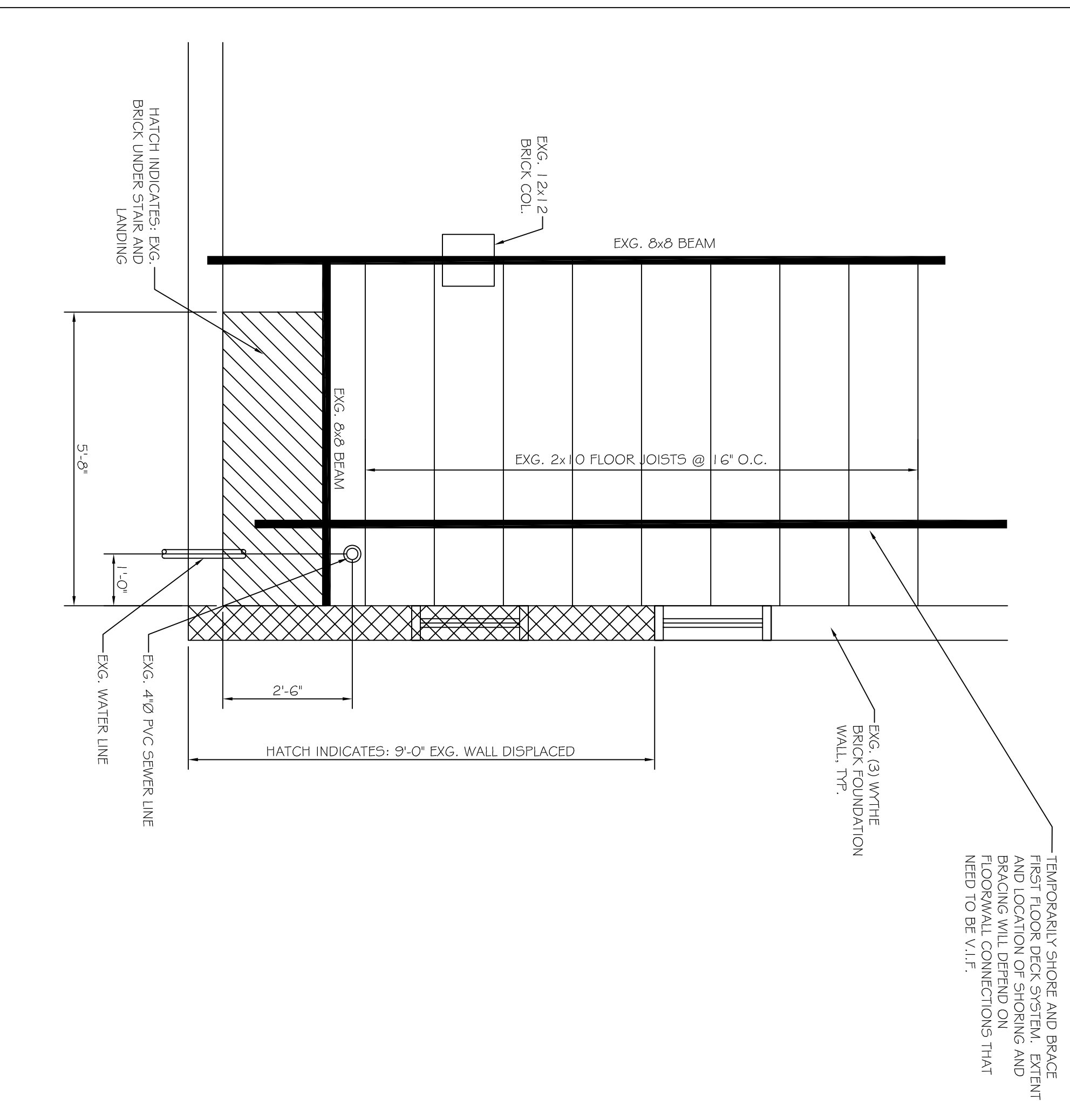
B2 EXG. FIRST FLOOR FRAMING PLAN SCALE: 1/2" = 1'-0"
