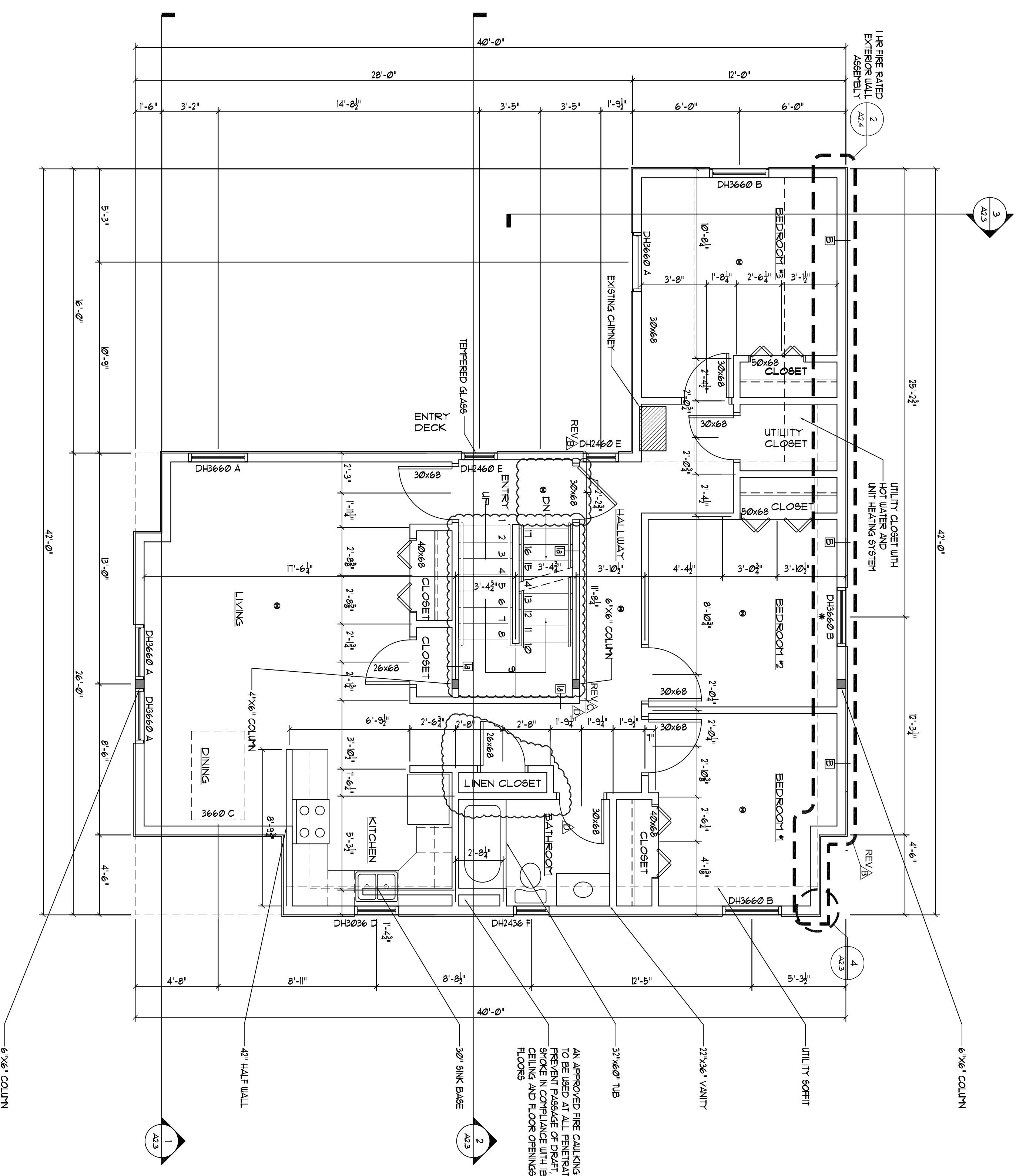
1 New Third Floor Plan Scale: 1/4" = 1'-0"
