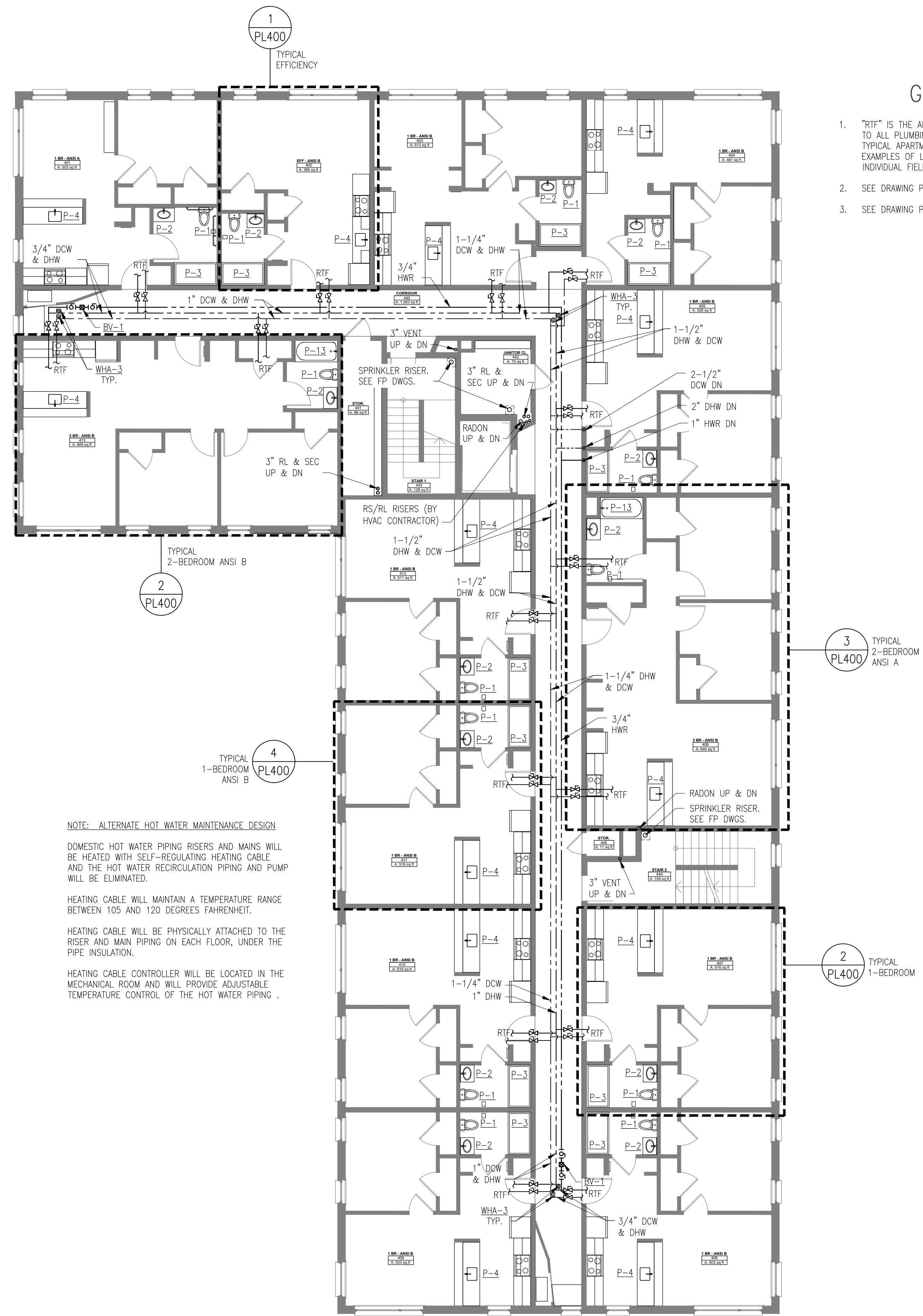
FOURTH FLOOR PIPING PLAN
