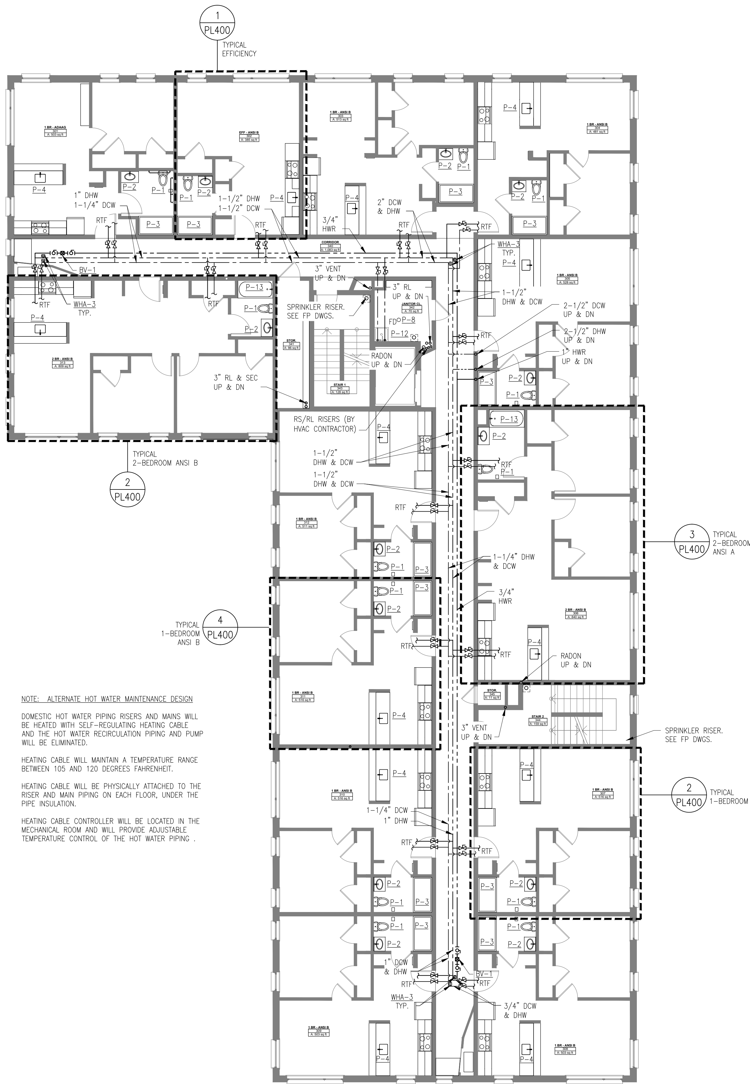
THIRD FLOOR PIPING PLAN
