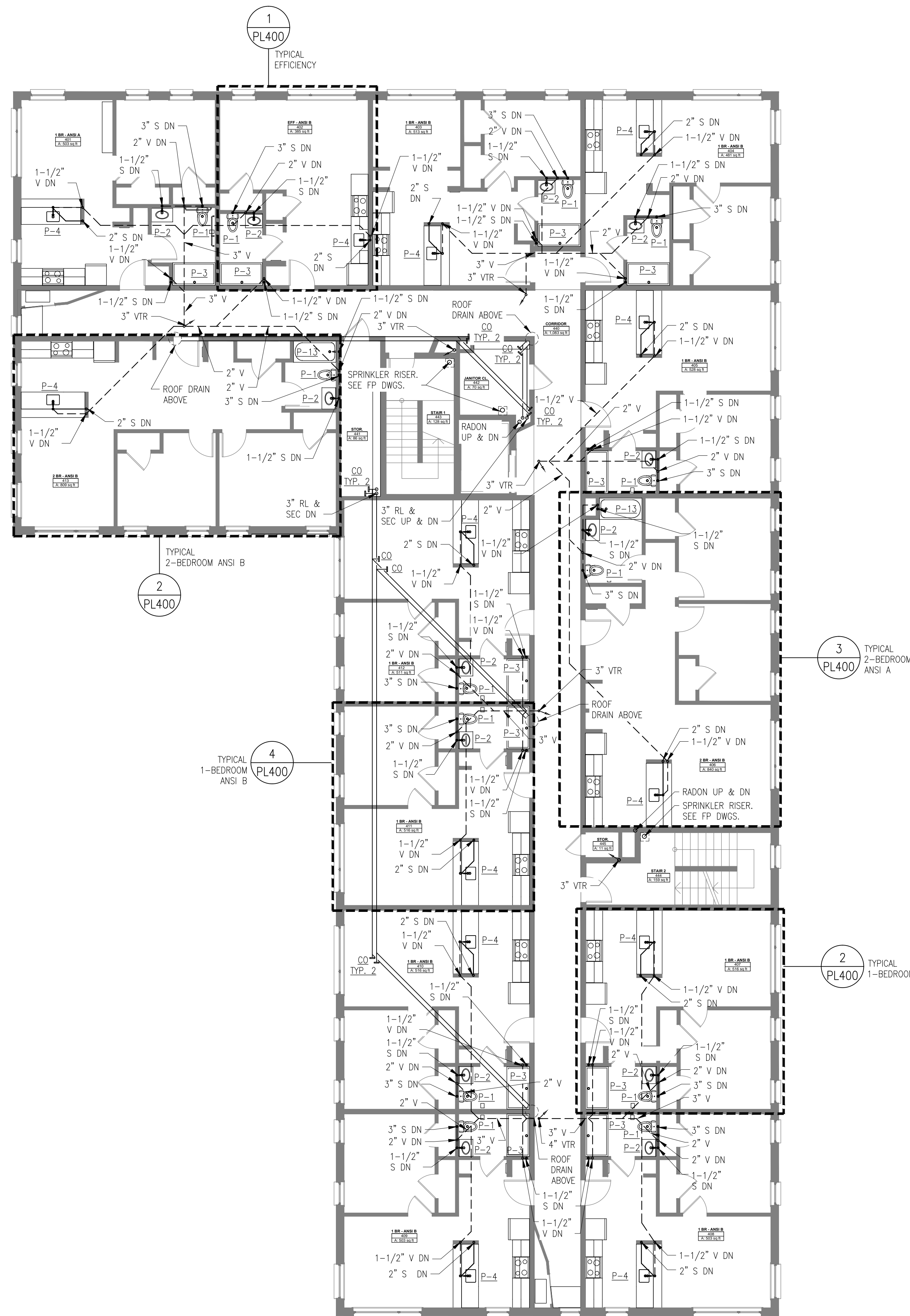
FOURTH FLOOR DRAIN, WASTE, VENT PLAN
