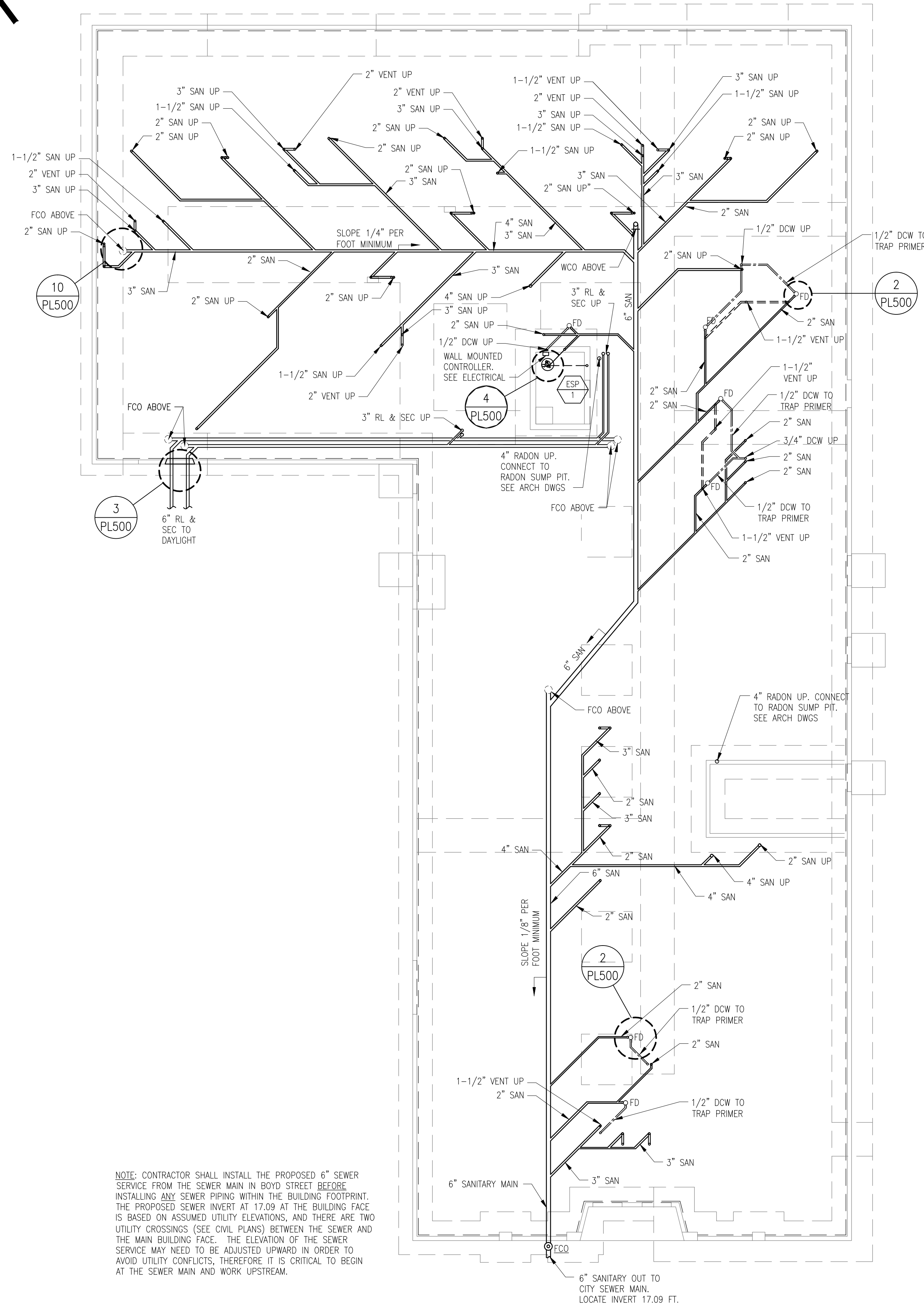
UNDERSLAB PIPING PLAN
