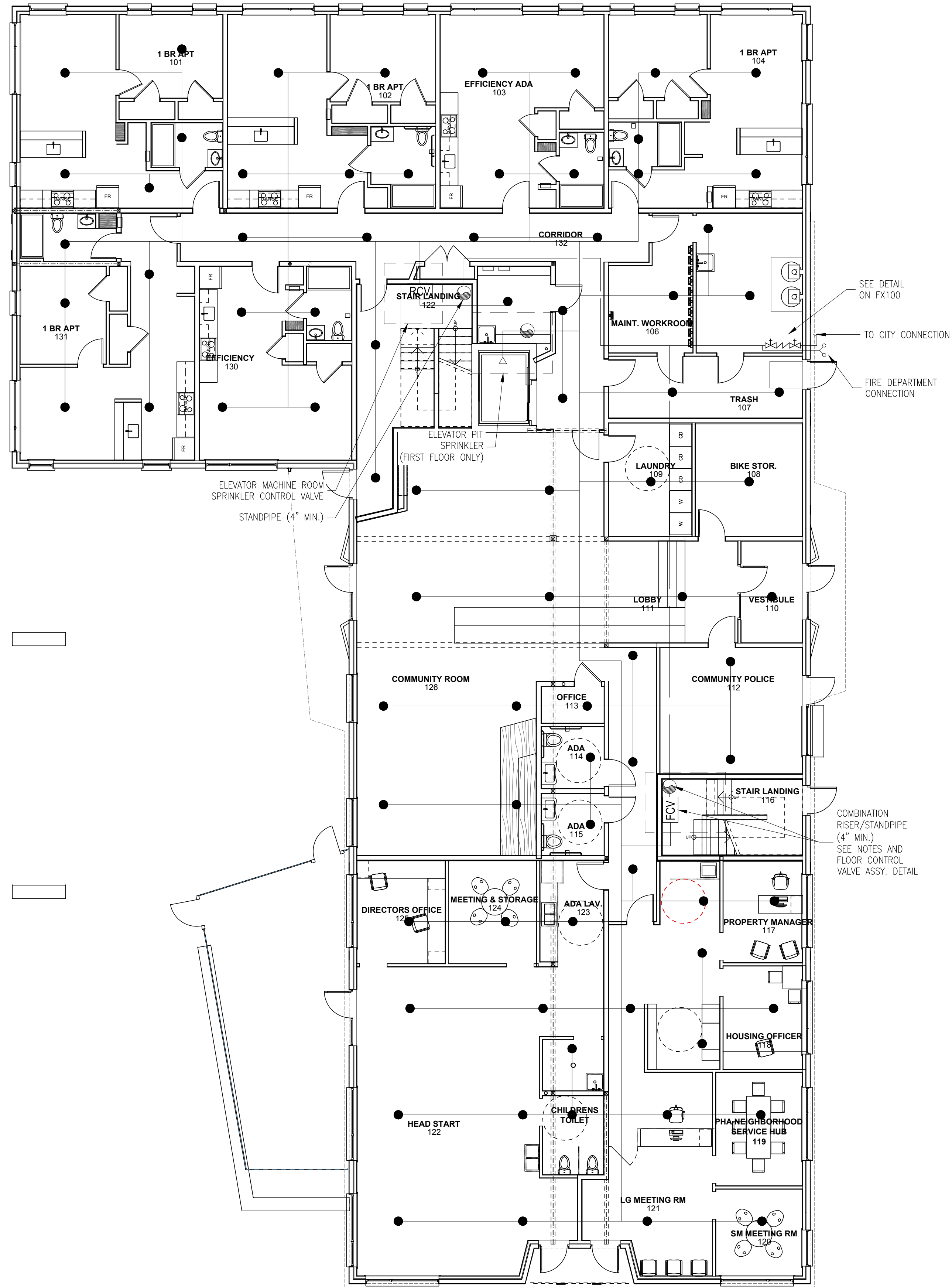
FIRE SPRINKLER FIRST FLOOR PLAN
