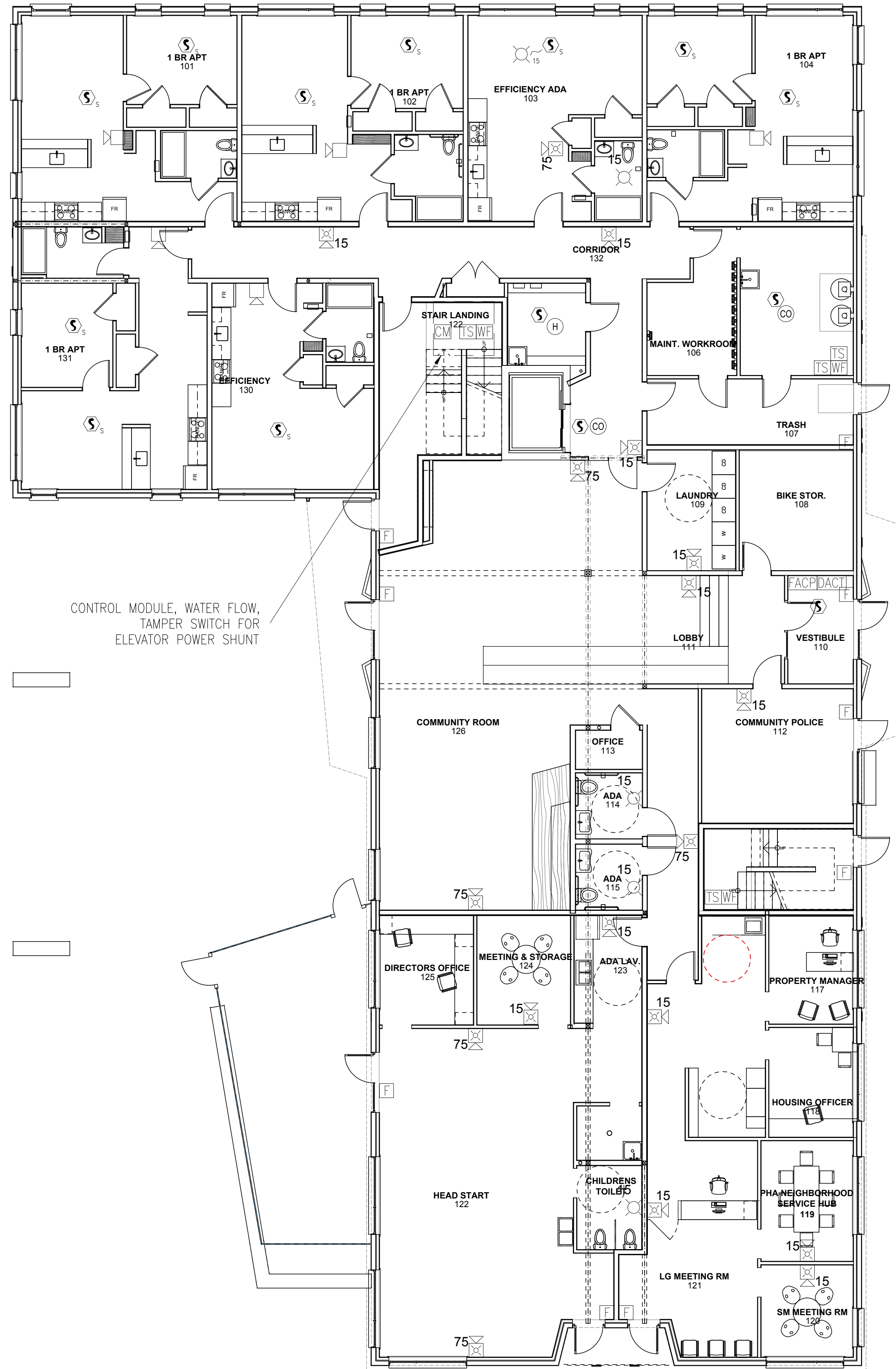
FIRE ALARM FIRST FLOOR PLAN SCALE: 1/8" = 1'-0"
