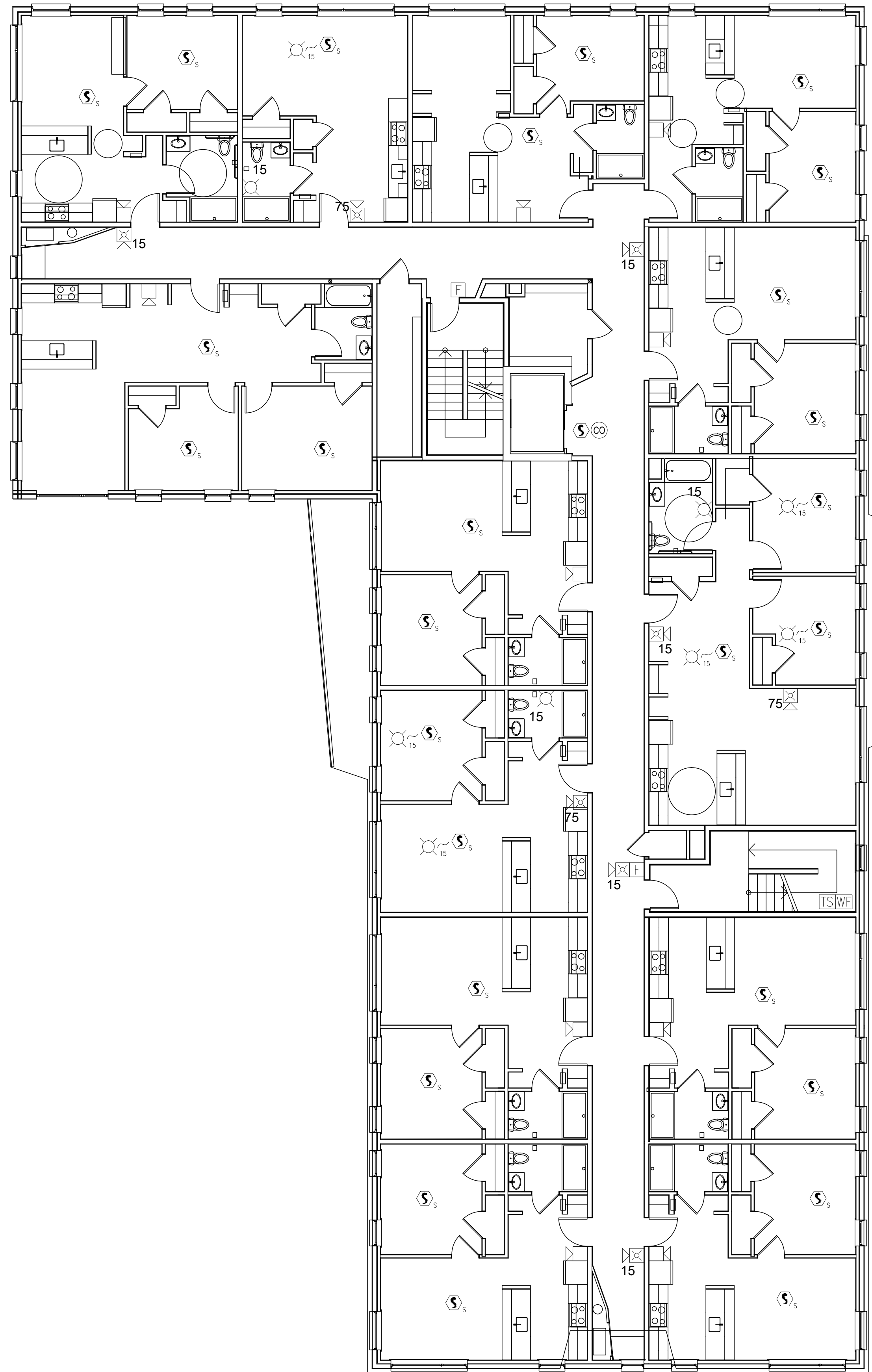
FIRE ALARM SECOND FLOOR PLAN SCALE: 1/8" = 1'-0"
