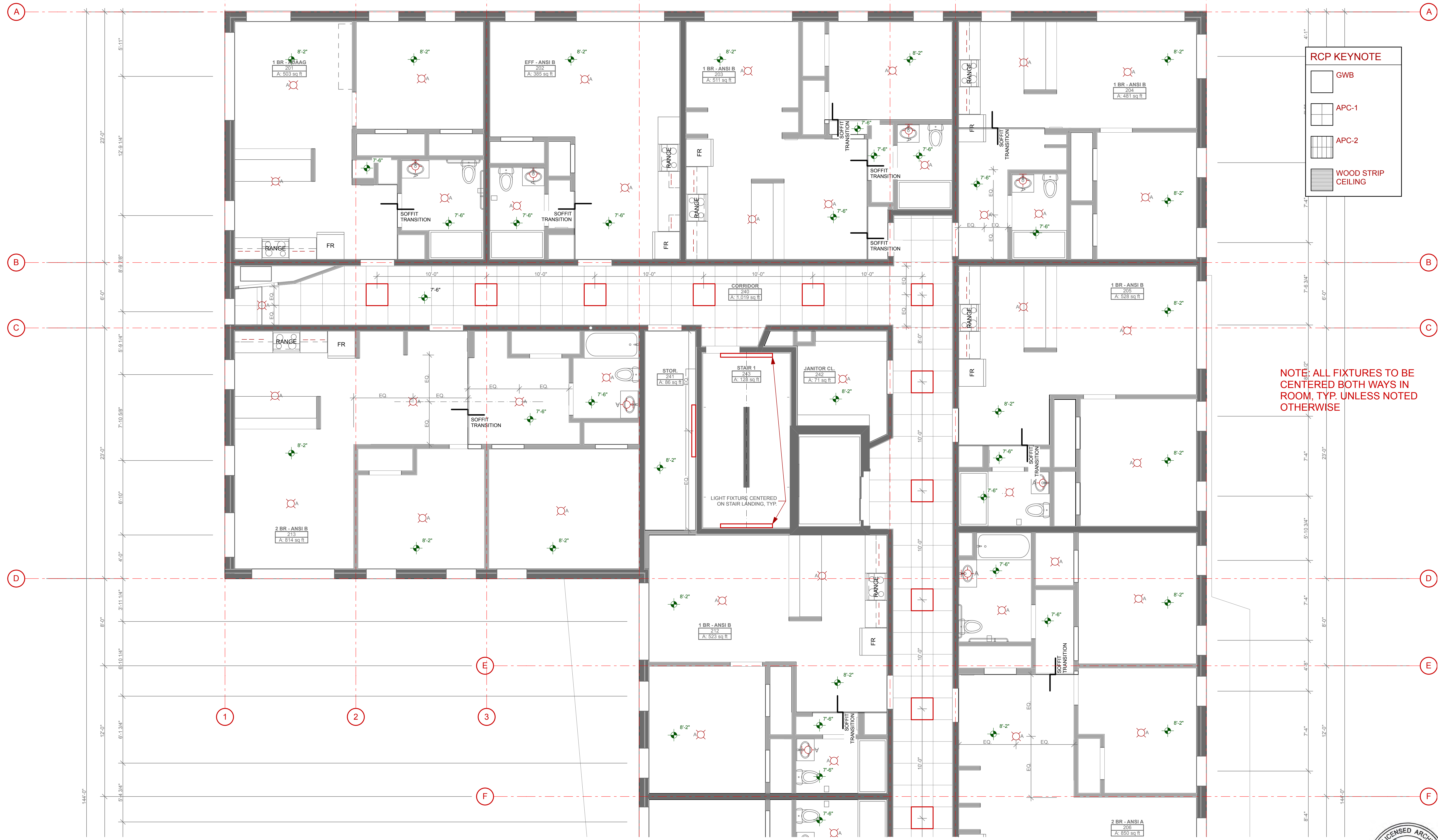
1 TYP. UPPER FLOOR RELECTED CEILING PLAN SCALE: 1/4" = 1'-0"
