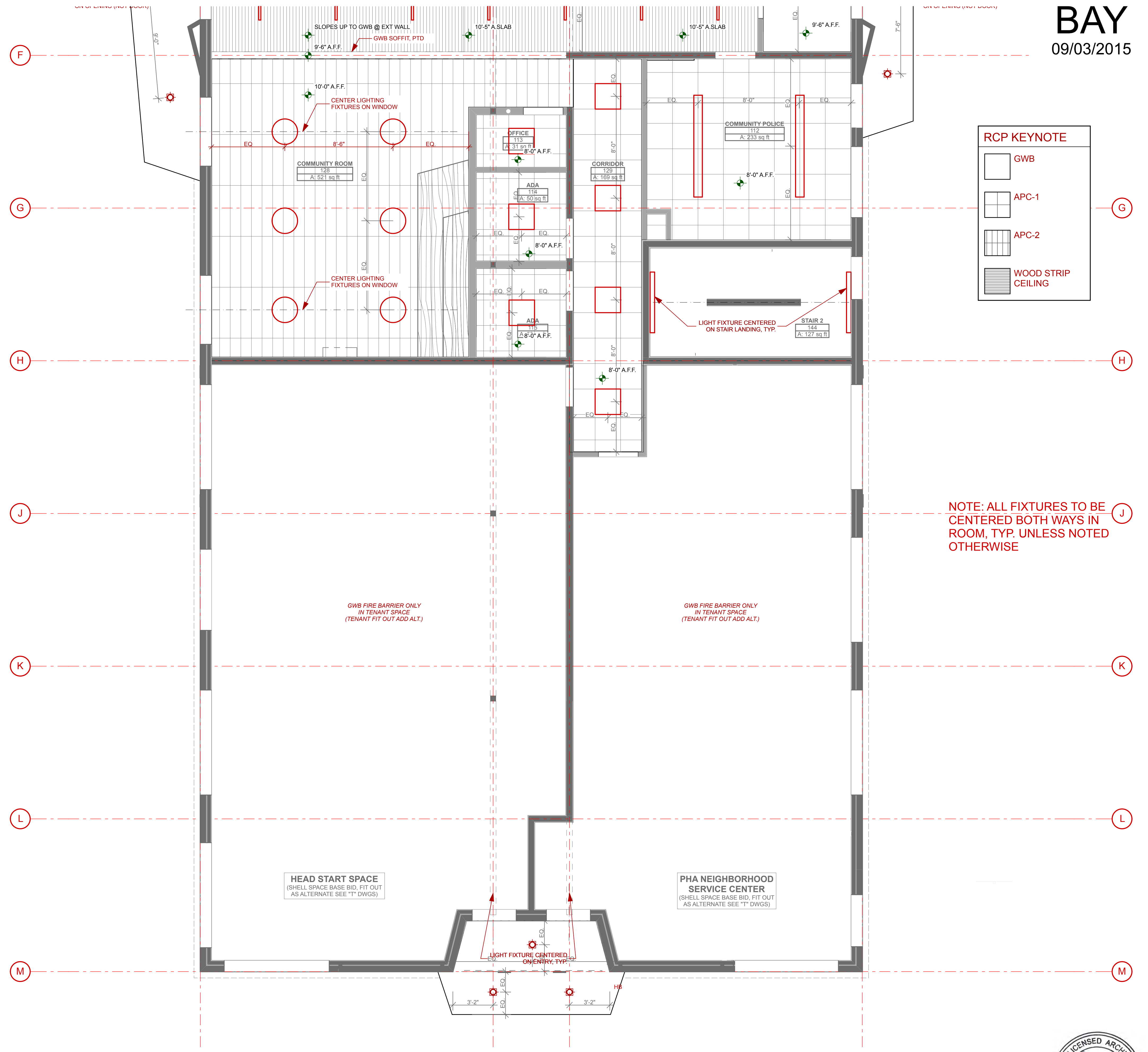
1 1st FLOOR REFLECTED CEILING PLAN SCALE: 1/4" = 1'-0"
