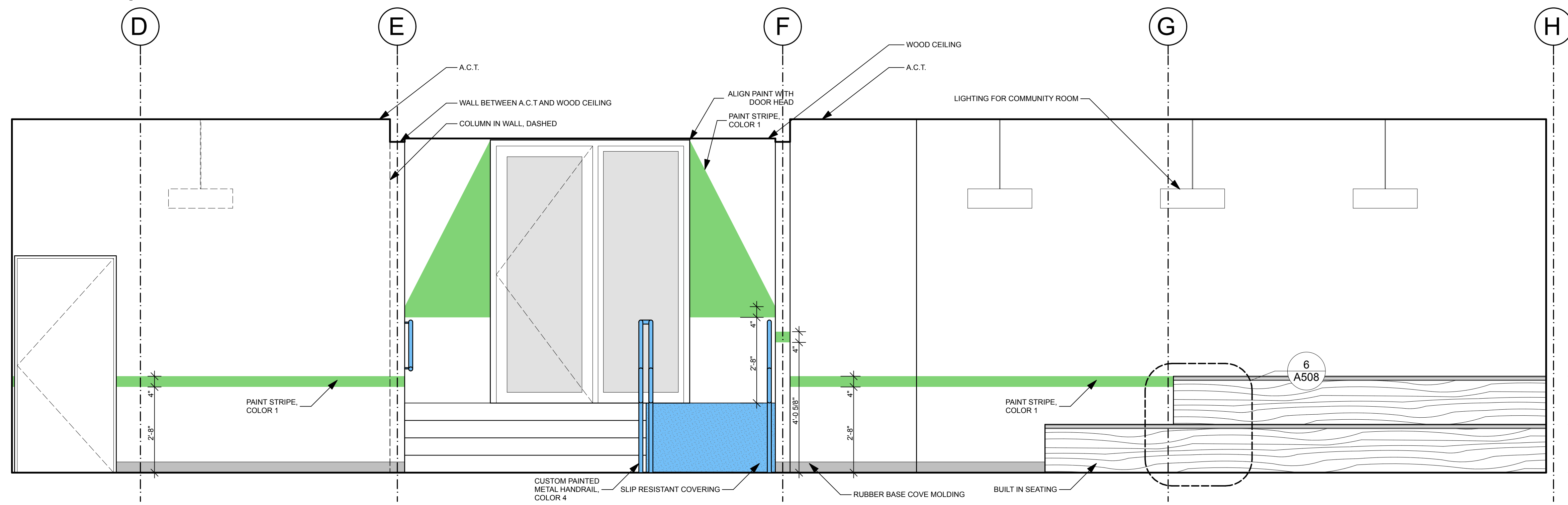
5 LOBBY AND COMMUNITY ROOM SE SCALE: 1/2" = 1'-0"
