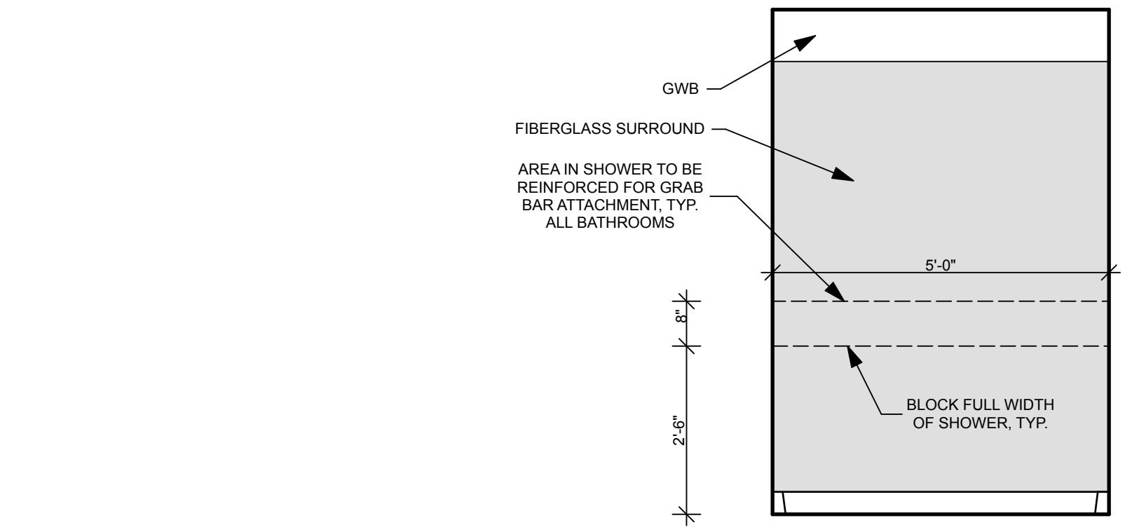
15 ANSI-B BATHROOM - TYP. SCALE: 1/2" = 1'-0" 0 1' 2' 4'
