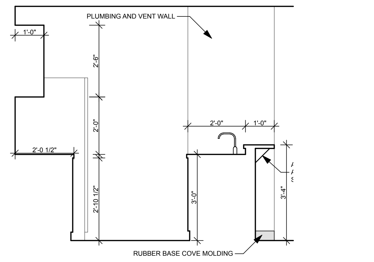
6 ANSI-B KITCHEN - TYP. SCALE: 1/2" = 1'-0" 0 1' 2' 4'
