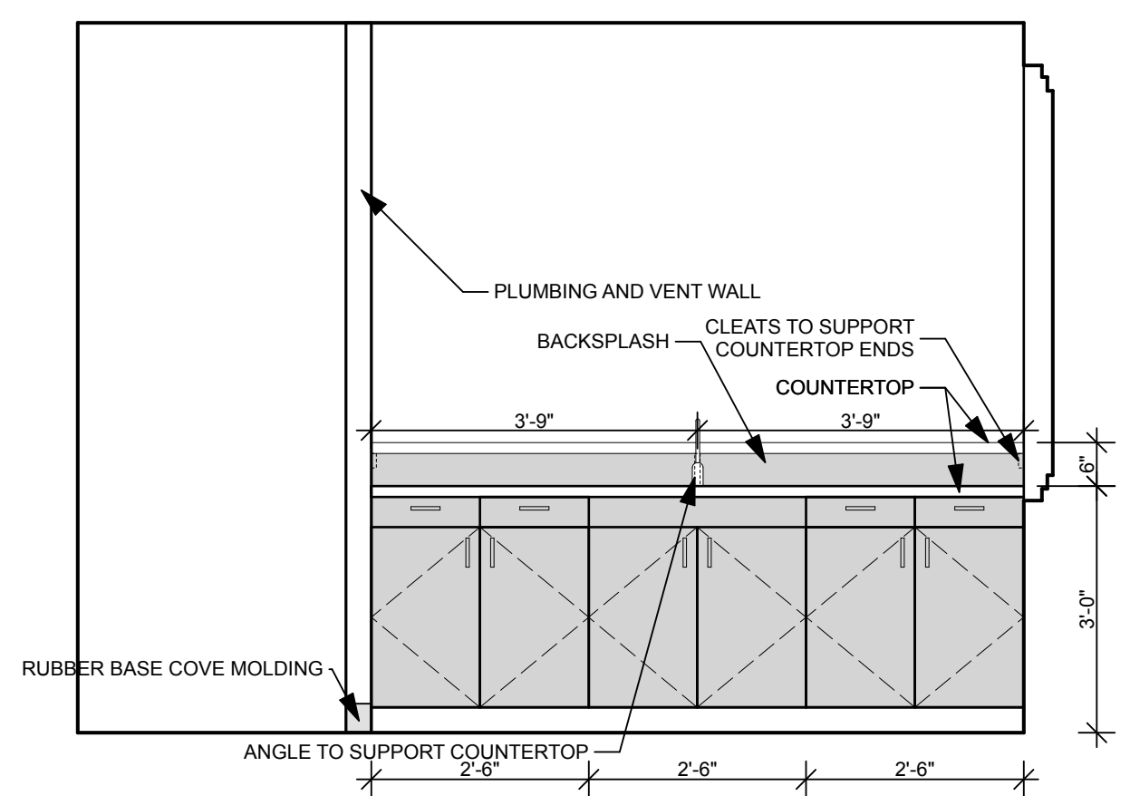
7 ANSI-B KITCHEN - TYP. SCALE: 1/2" = 1'-0" 0 1' 2' 4'
