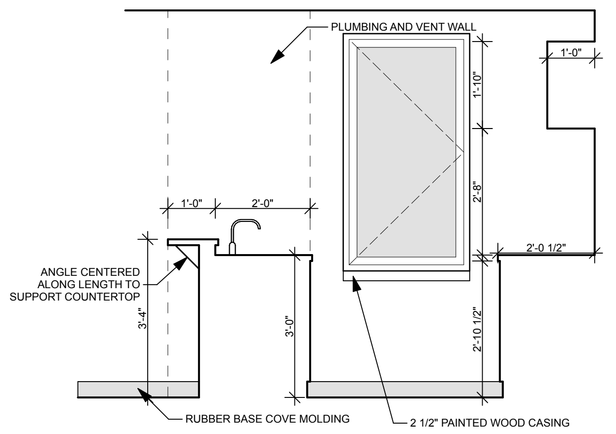
8 ANSI-B KITCHEN - TYP. SCALE: 1/2" = 1'-0" 0 1' 2' 4'
