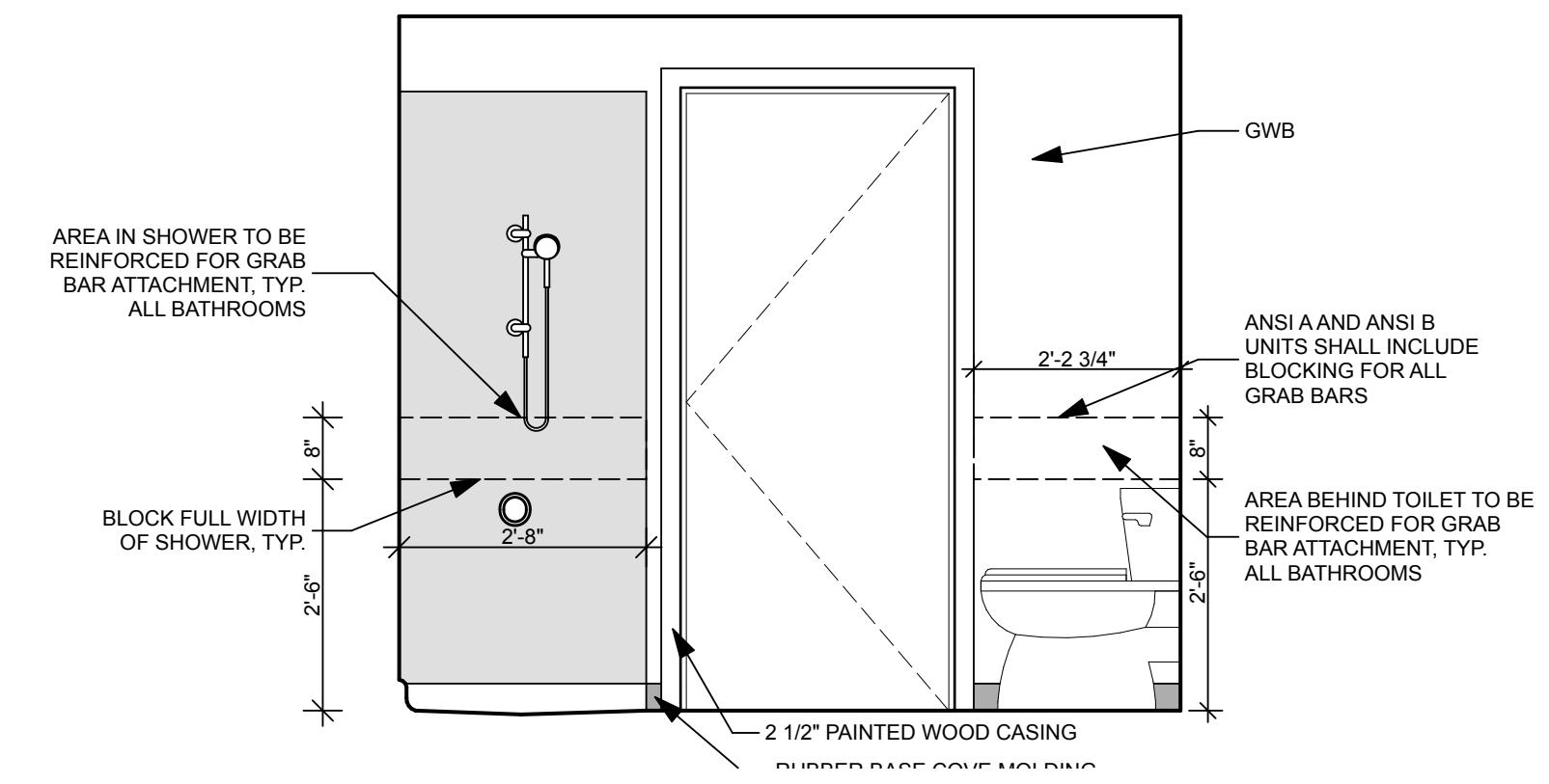
16 ANSI-B BATHROOM - TYP. SCALE: 1/2" = 1'-0" 0 1' 2' 4'
