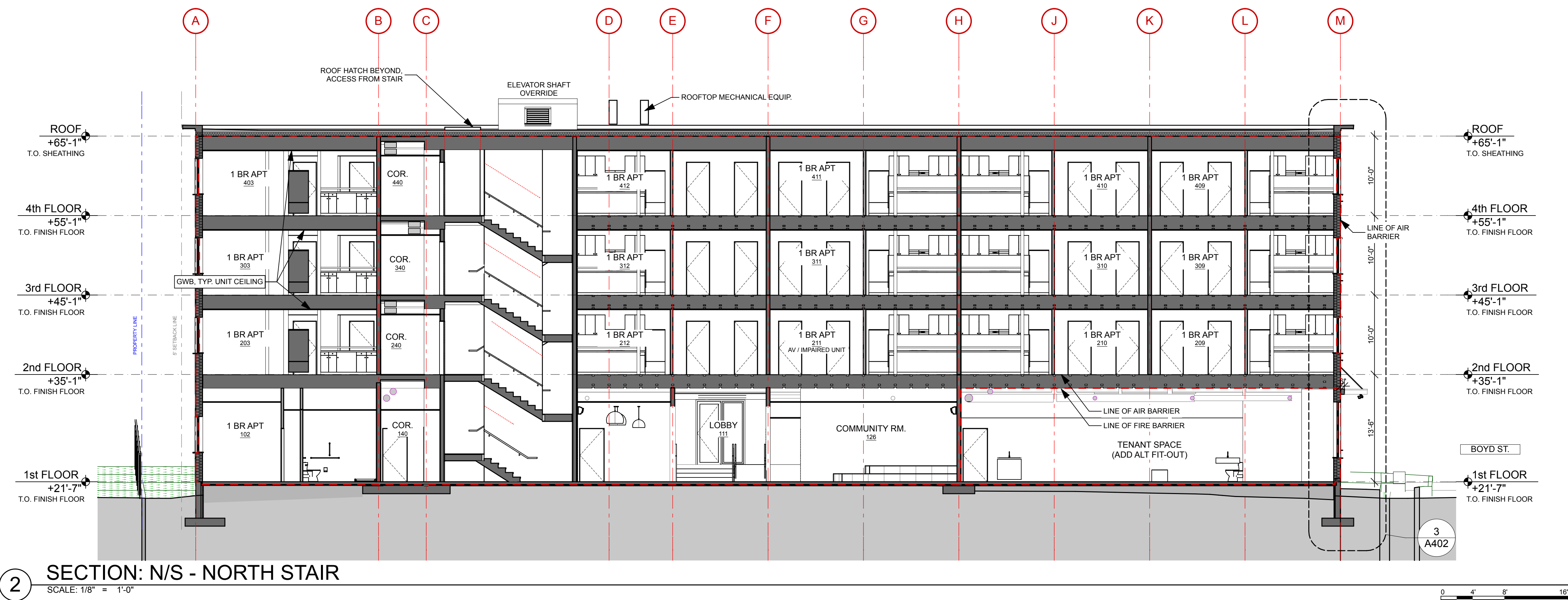
1 SECTION: N/S - SOUTH STAIR SCALE: 1/8" = 1'-0"
