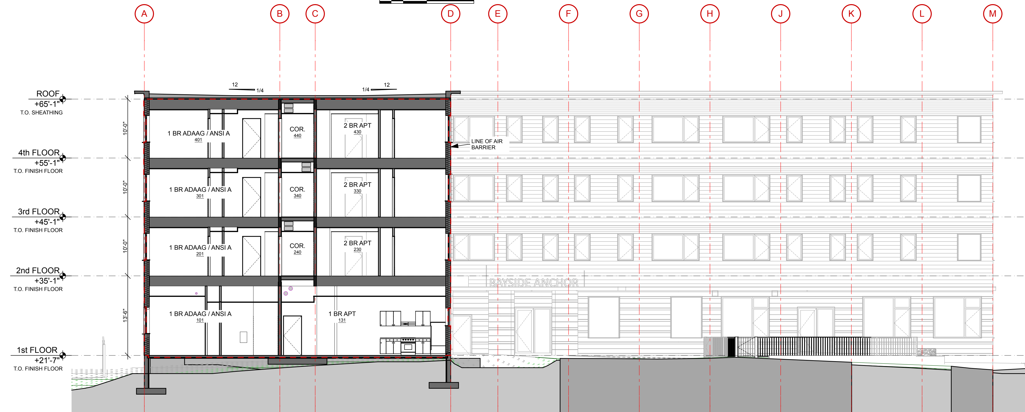
3 SECTION: N/S - UNITS SCALE: 1/8" = 1'-0"
