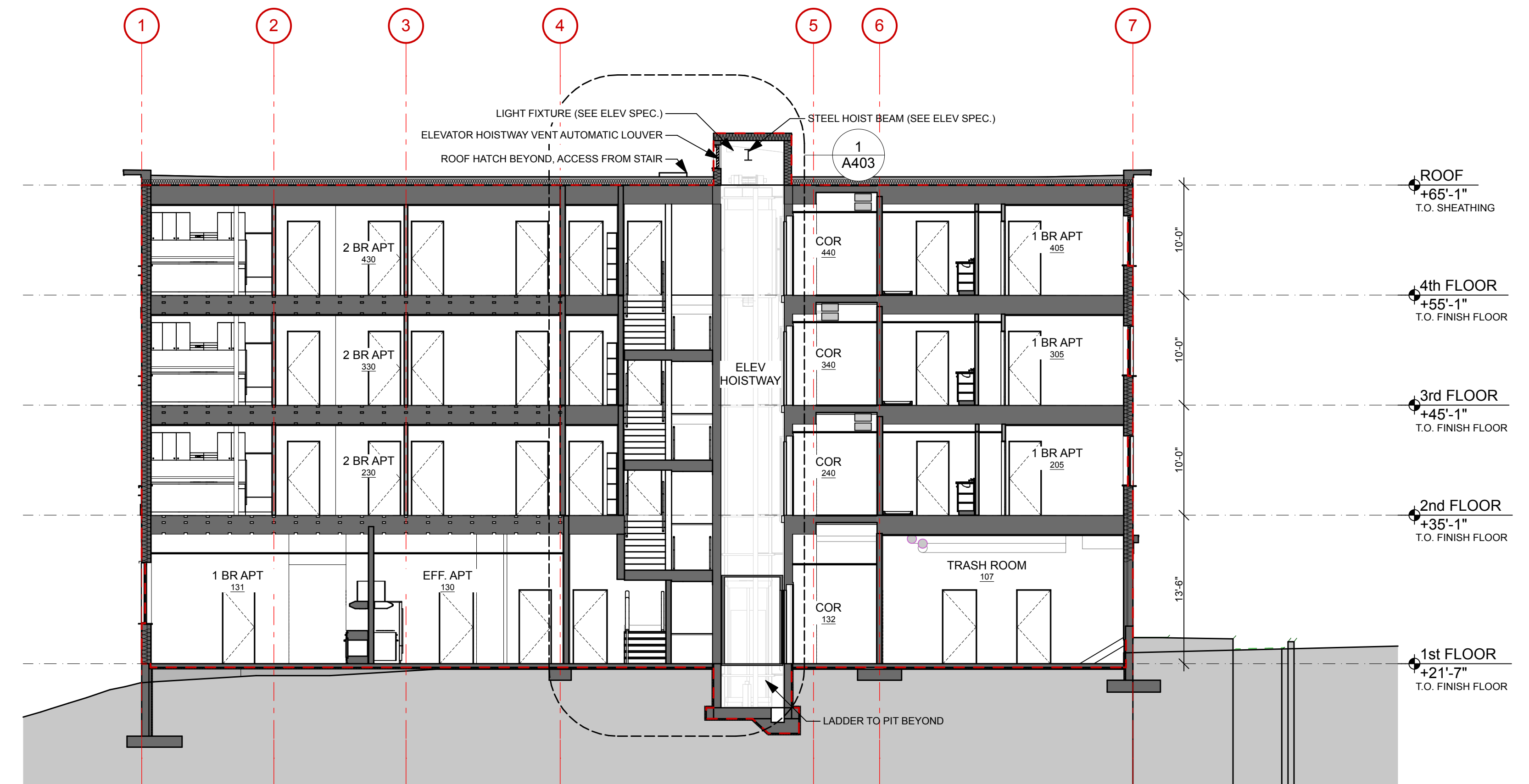
1 SECTION: E/W ELEVATOR SCALE: 1/8" = 1'-0"
