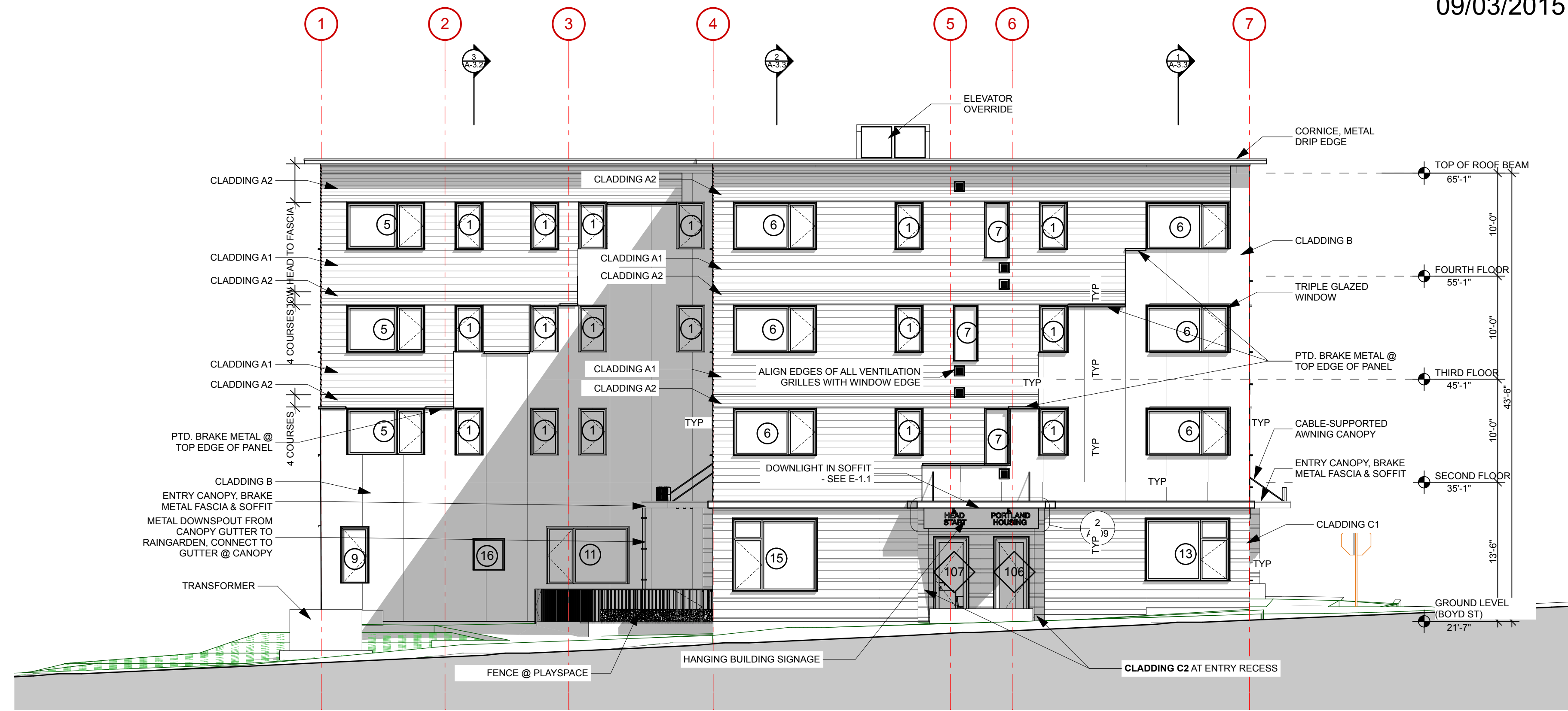
1 SOUTHWEST ELEVATION SCALE: 1/8" = 1'-0"
