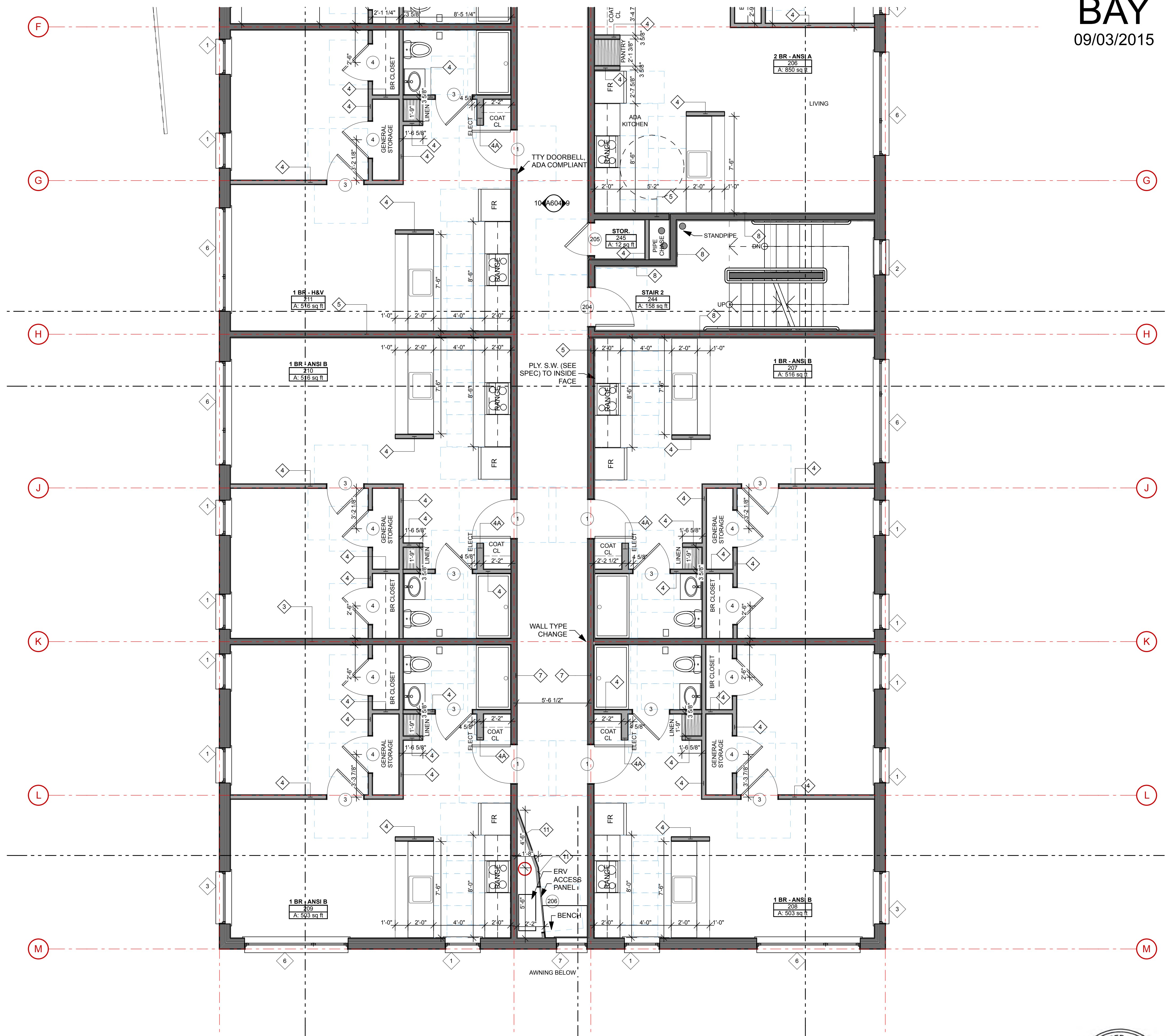
1 TYPICAL UNIT PLANS SCALE: 1/4" = 1'-0"
