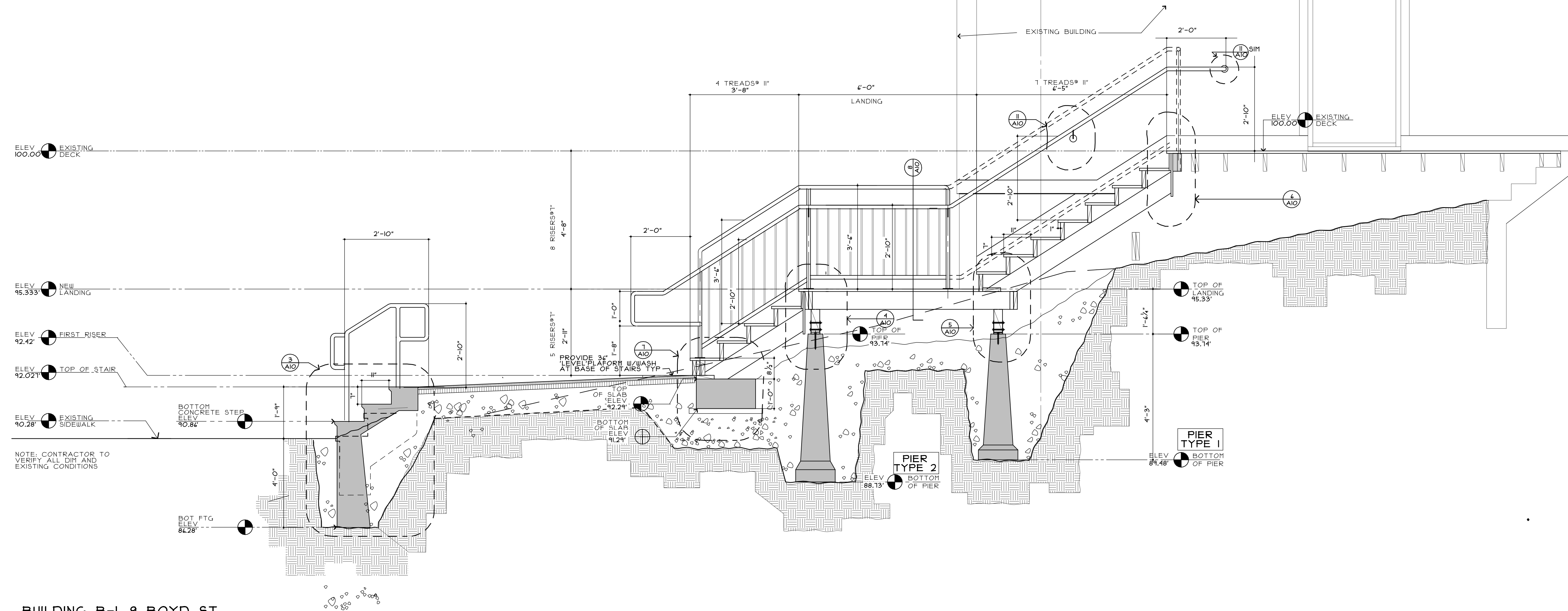
BUILDING B-1, 9 BOYD ST STAIR #1 SECTION THRU STAIR SCALE: 1/2" = 1'-0"
