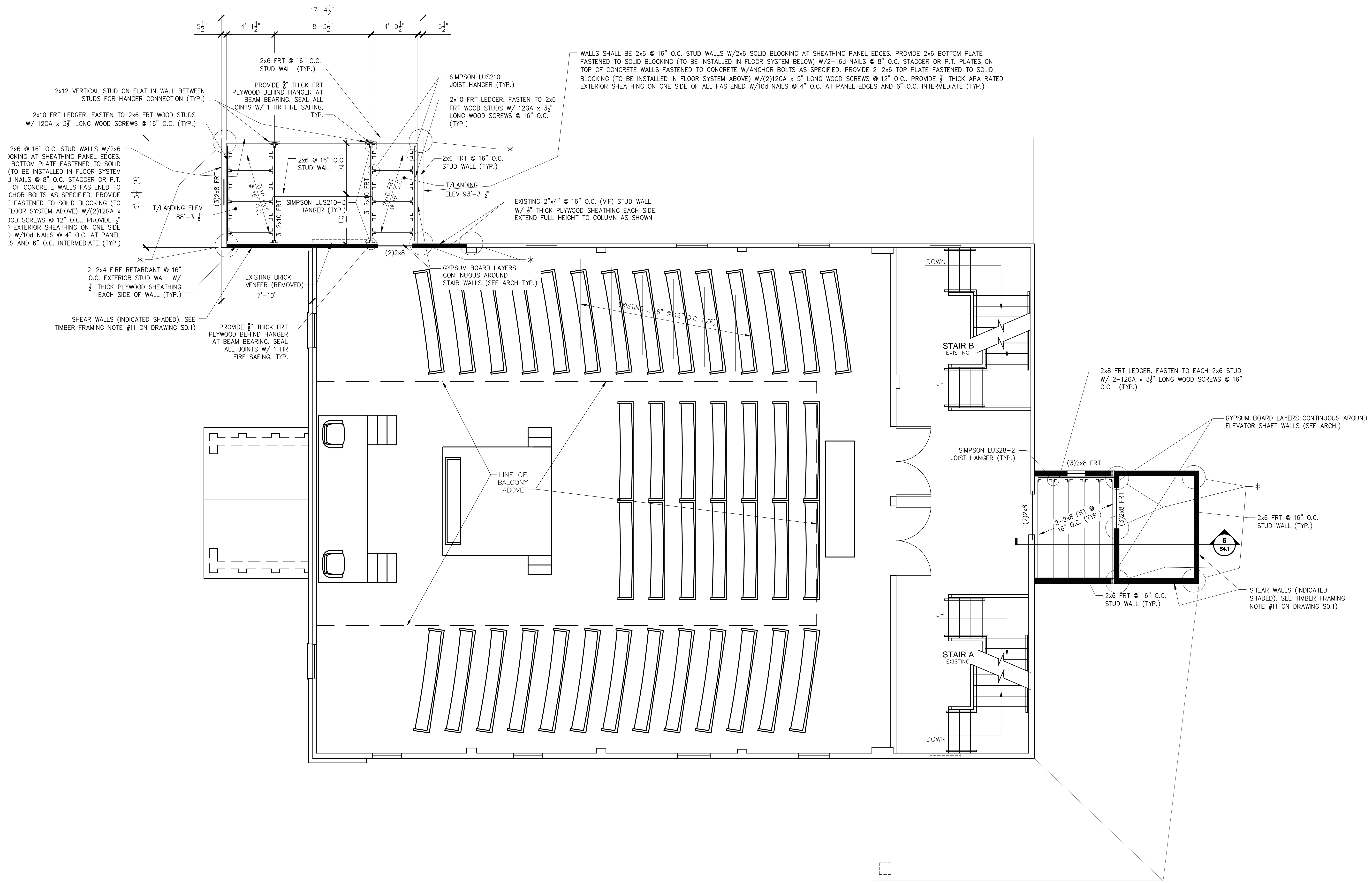
THIRD FLOOR FRAMING PLAN 1/4" = 1'-0"
