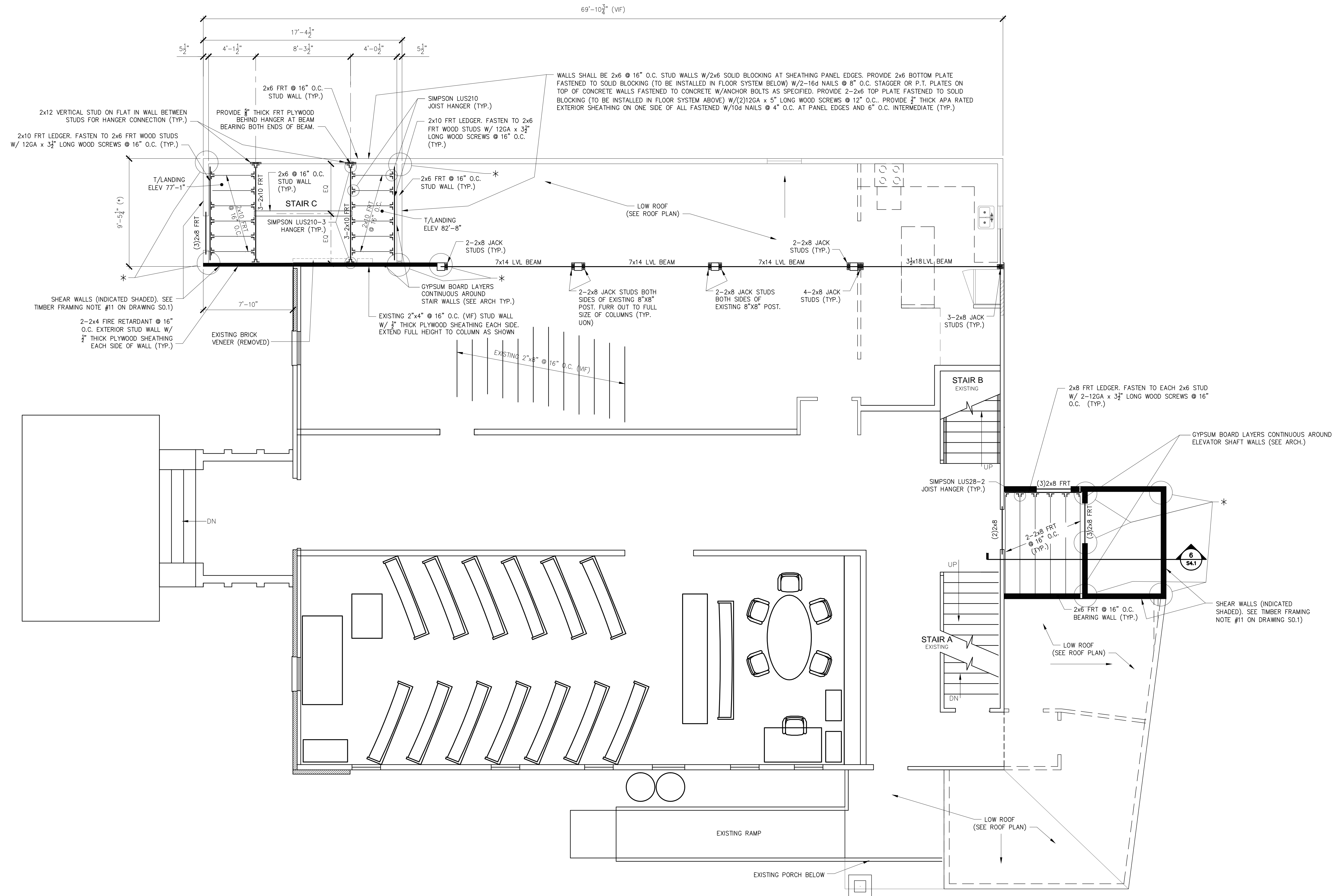
SECOND FLOOR FRAMING PLAN 1/4" = 1'-0"
