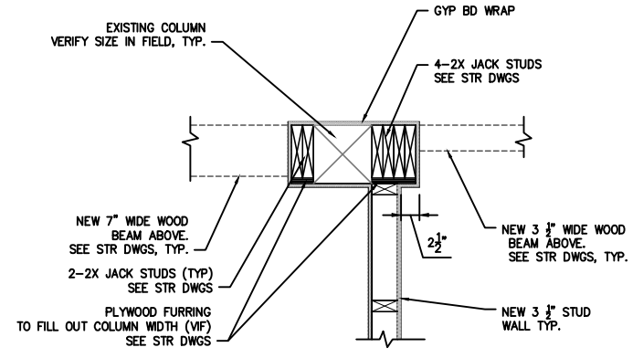
PLAN DETAIL C 1" = 1'-0" A2
