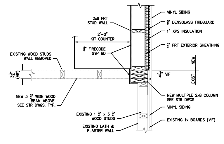
PLAN DETAIL B 1" = 1'-0" A1, A2
