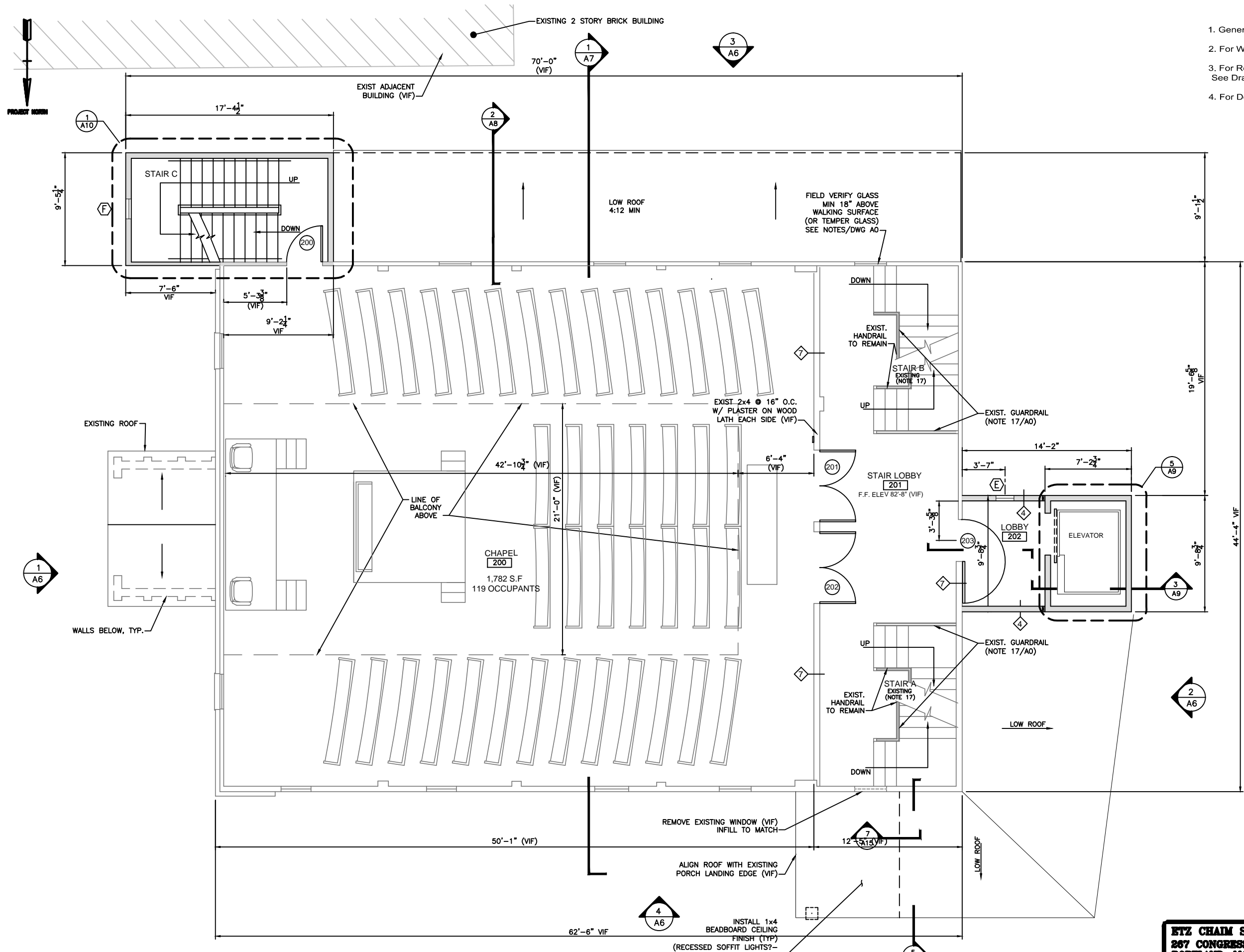
SECOND FLOOR PLAN 1/4" = 1'-0"
