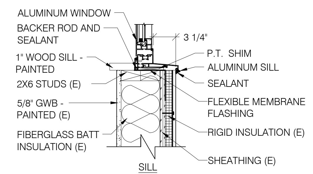
4 WINDOW DETAILS @ METAL SIDING SCALE: 1 1/2" = 1'-0"
