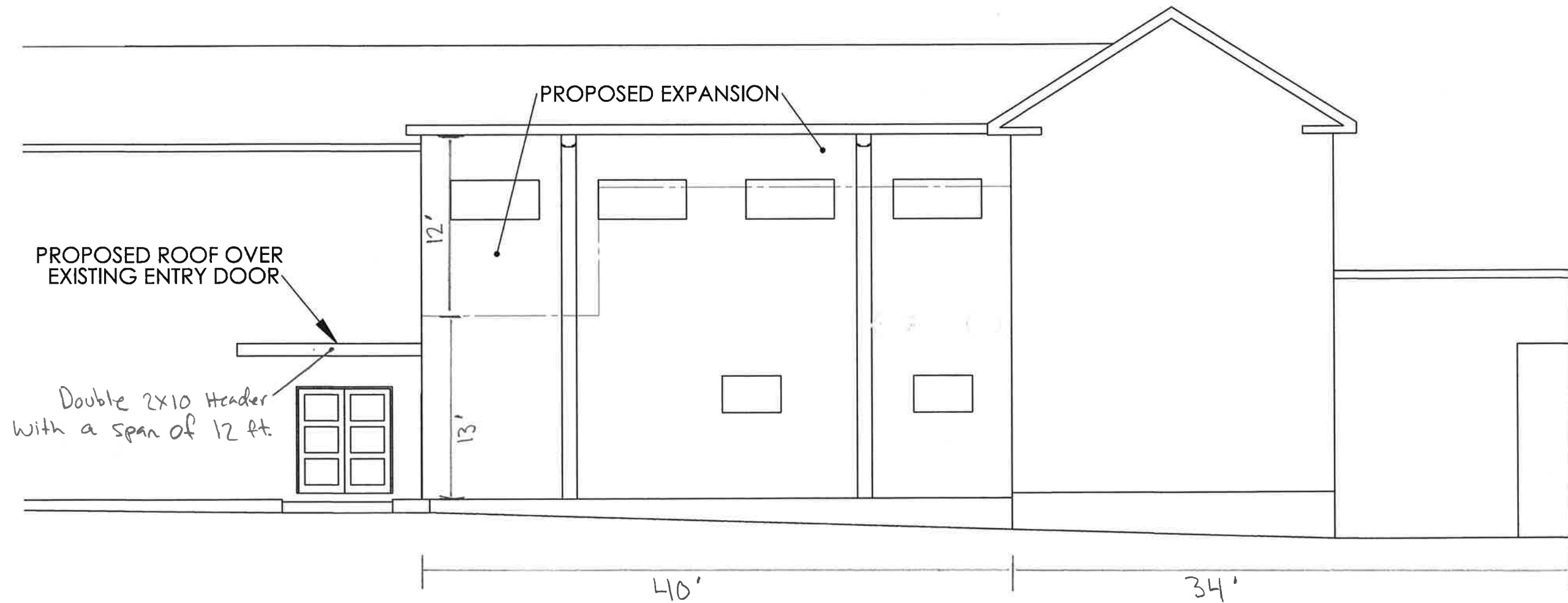
WEST ELEVATION - PROPOSED CONSTRUCTION
